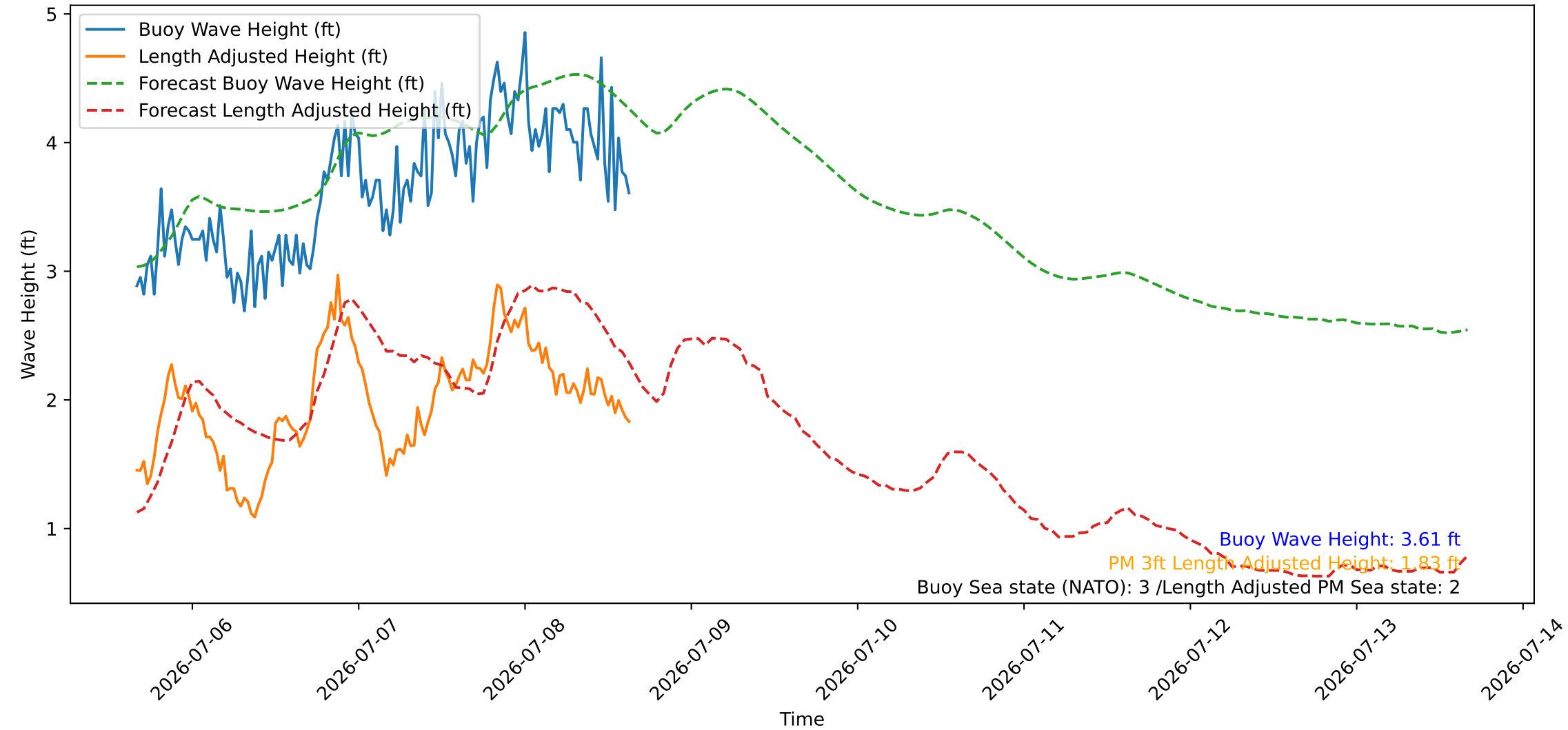
Wave Heights over Time for Red Beach at 2026-07-08 15:40:45
