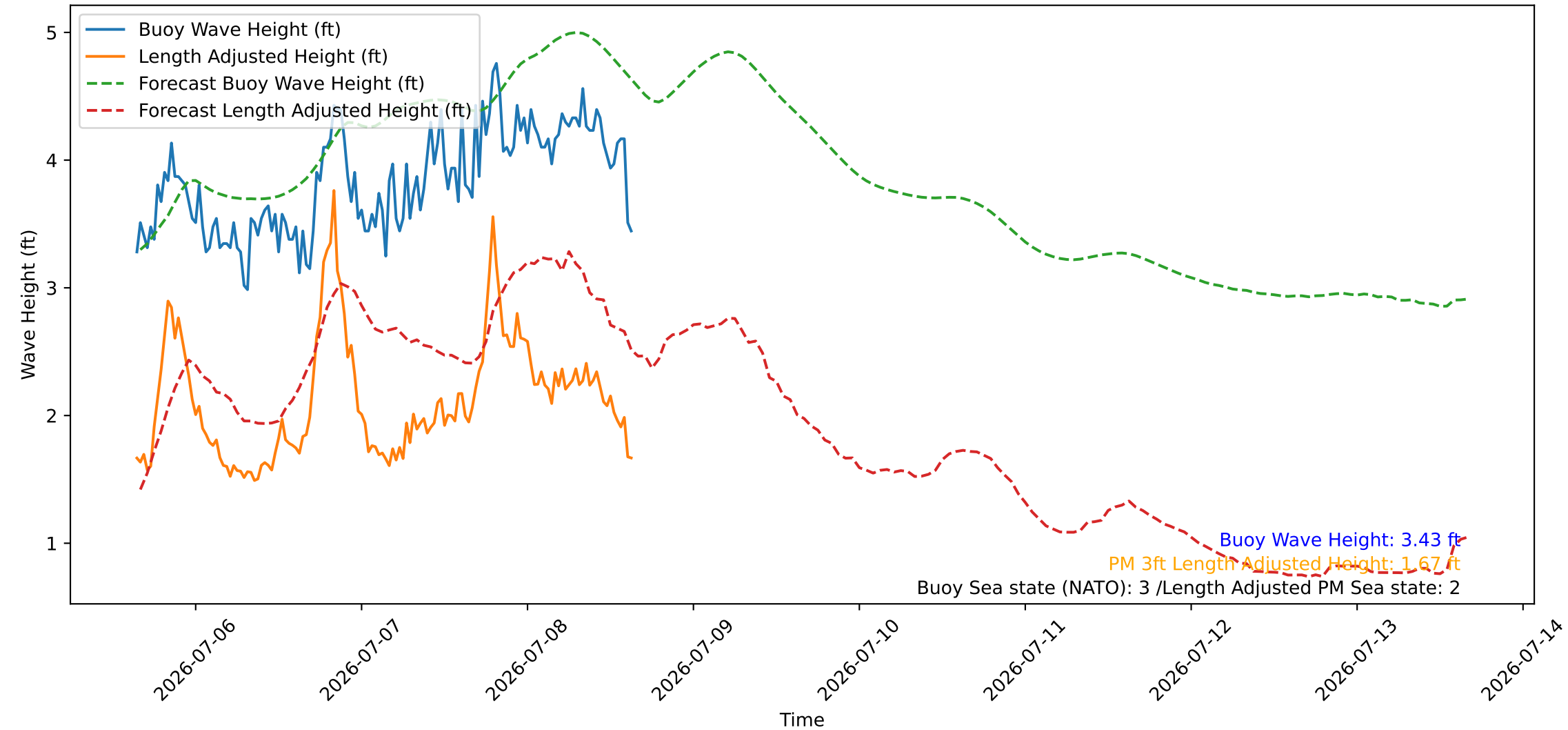
Wave Heights over Time for Green Beach at 2026-07-08 15:41:07
