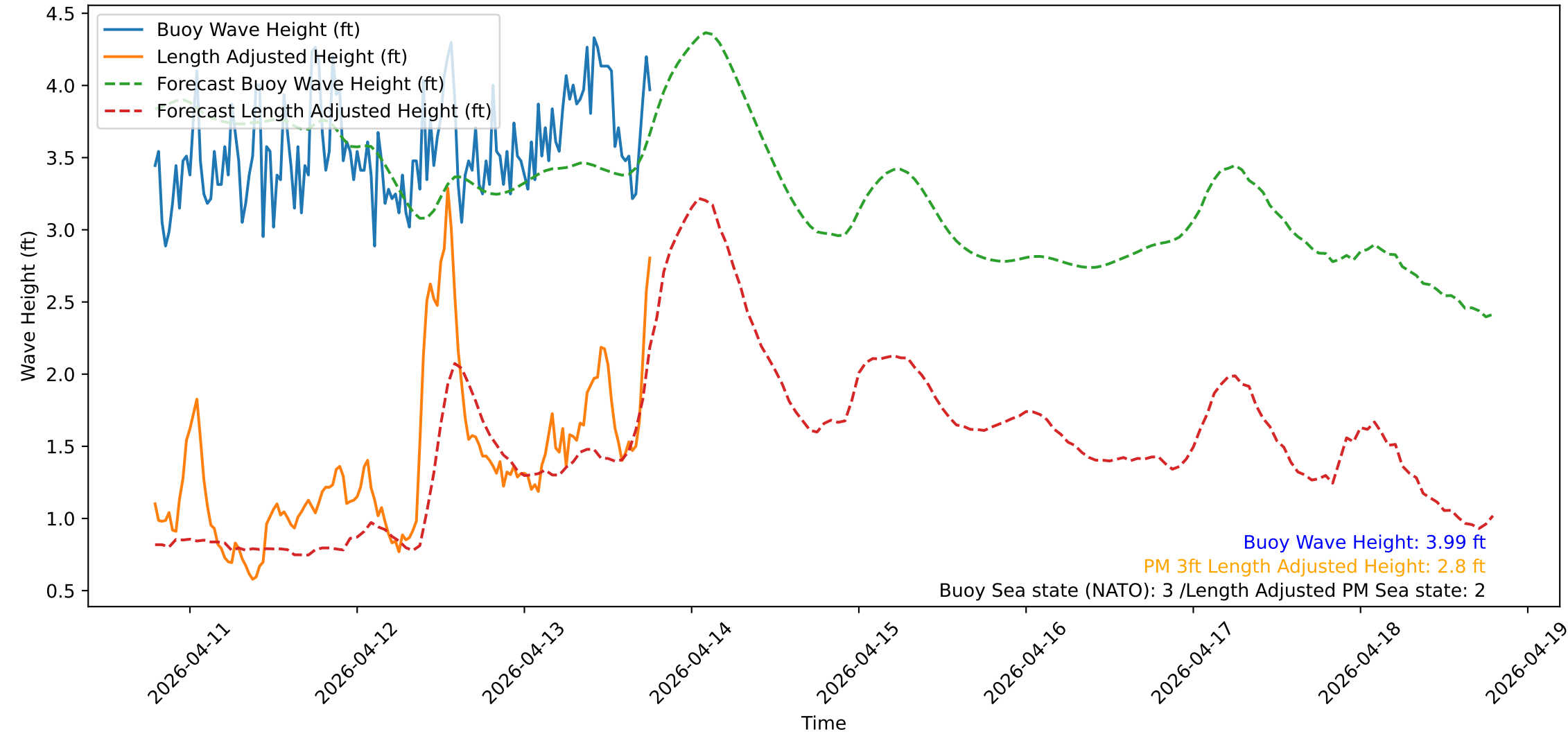
Wave Heights over Time for Red Beach at 2026-04-13 18:40:51
