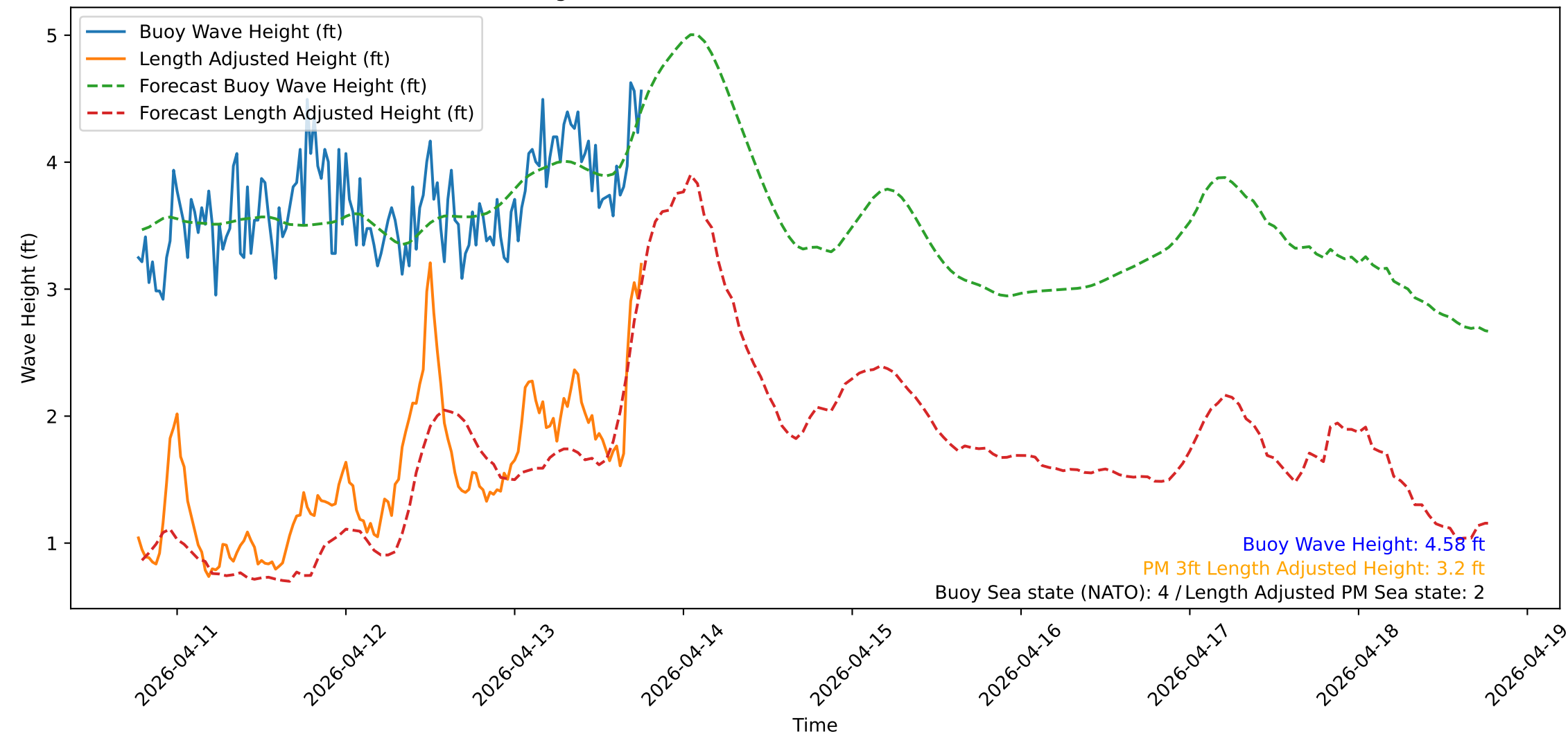
Wave Heights over Time for Green Beach at 2026-04-13 18:41:13
