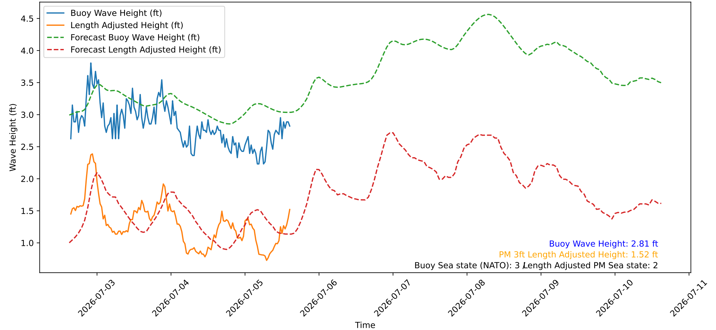
Wave Heights over Time for Red Beach at 2026-07-05 15:20:47
