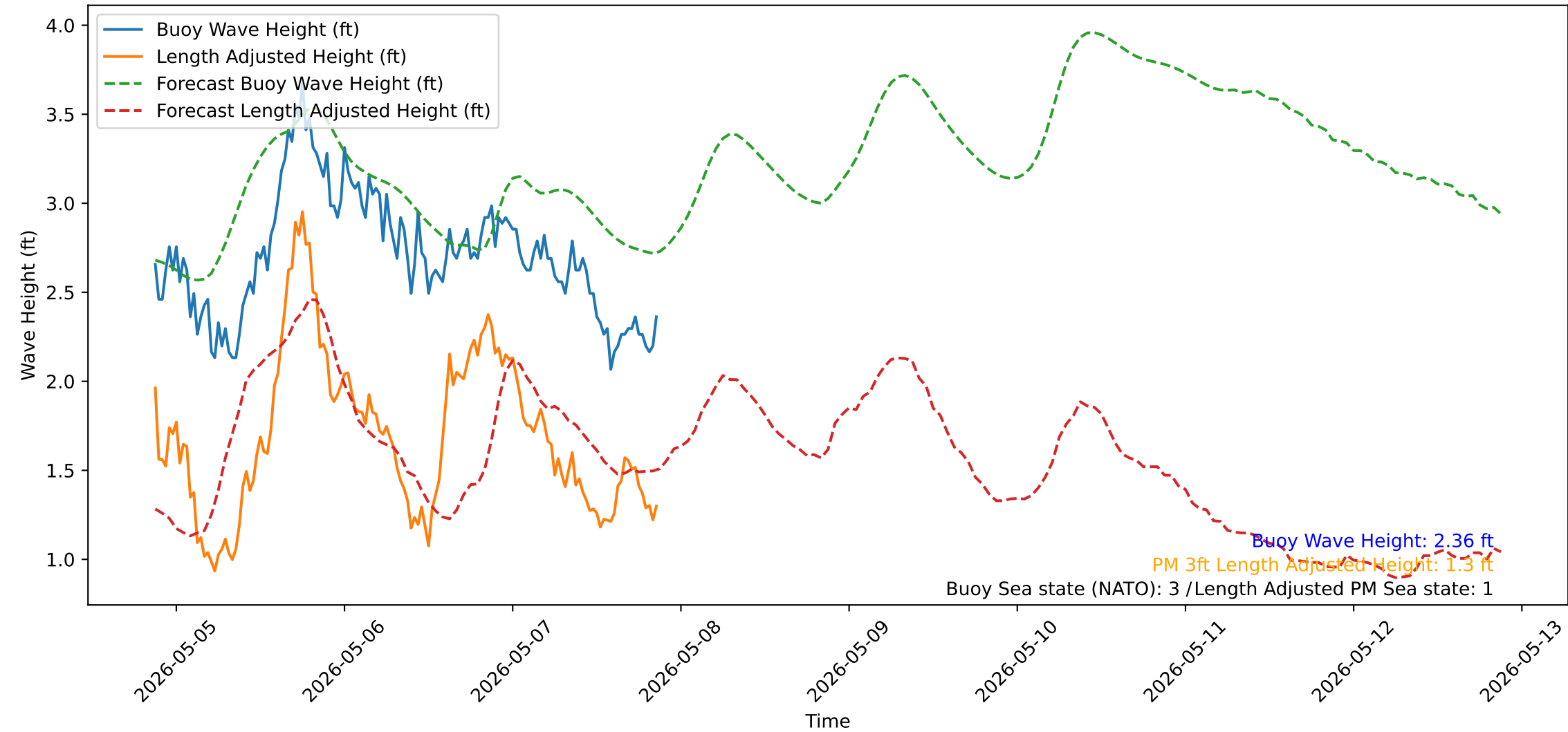
Wave Heights over Time for Green Beach at 2026-05-07 21:11:13
