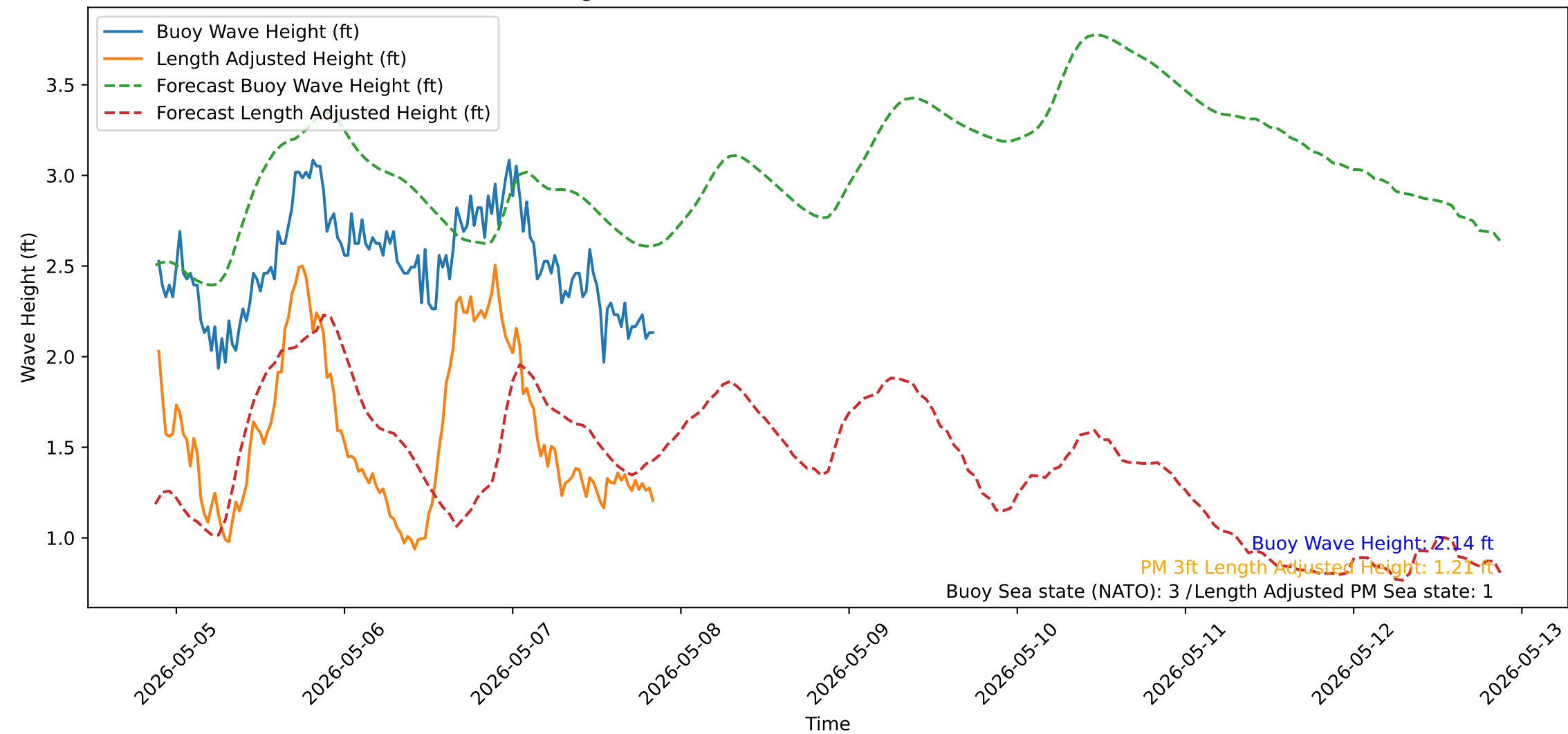
Wave Heights over Time for Red Beach at 2026-05-07 21:10:51
