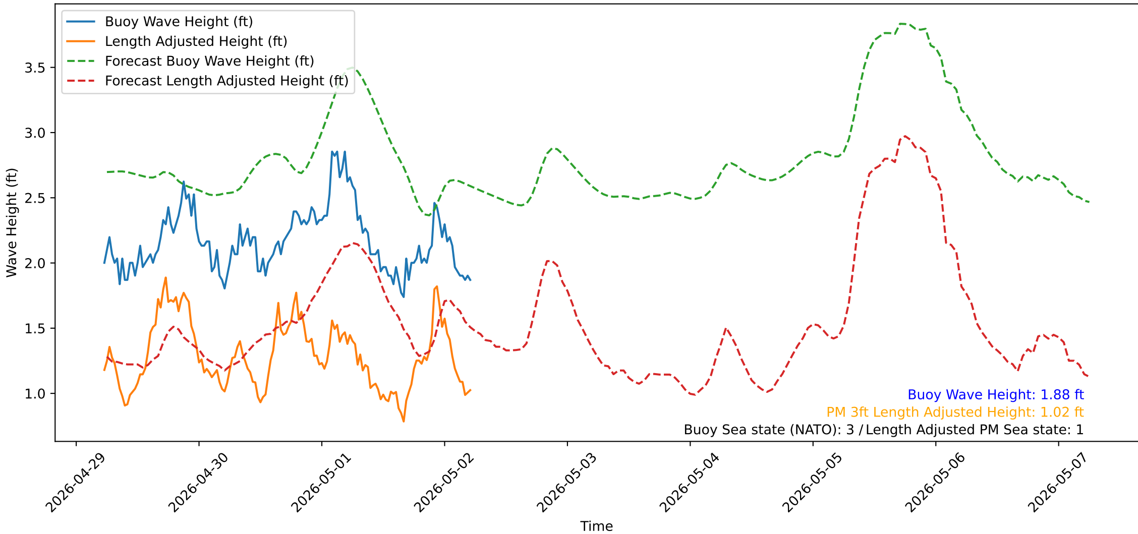
Wave Heights over Time for Green Beach at 2026-05-02 05:41:14
