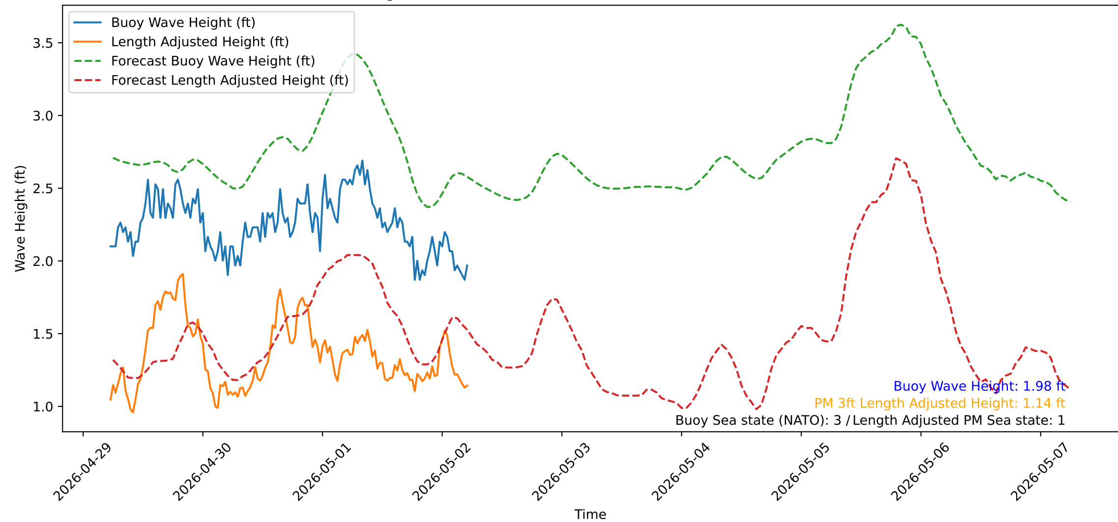
Wave Heights over Time for Oceanside Harbor at 2026-05-02 05:40:32
