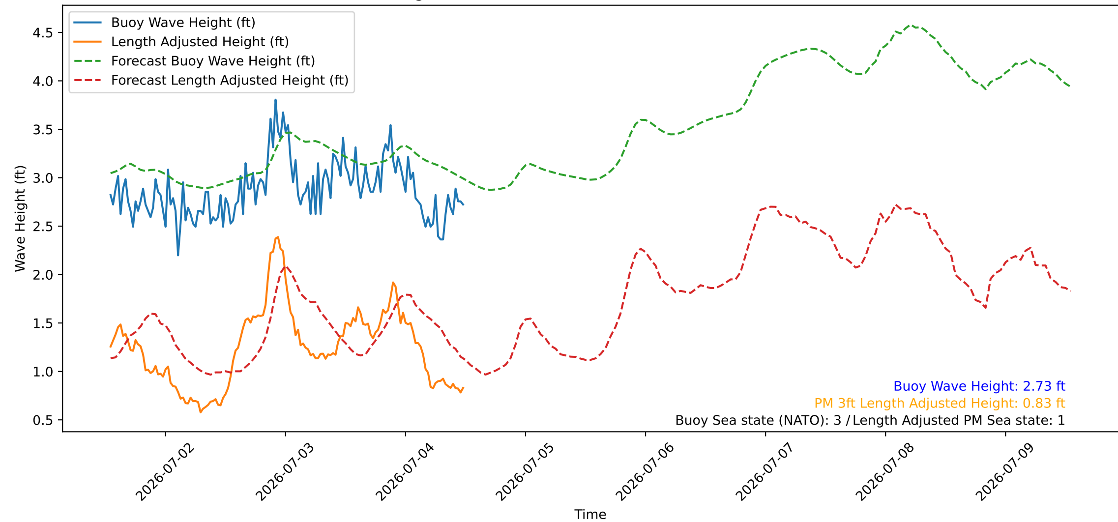
Wave Heights over Time for Red Beach at 2026-07-04 12:40:45
