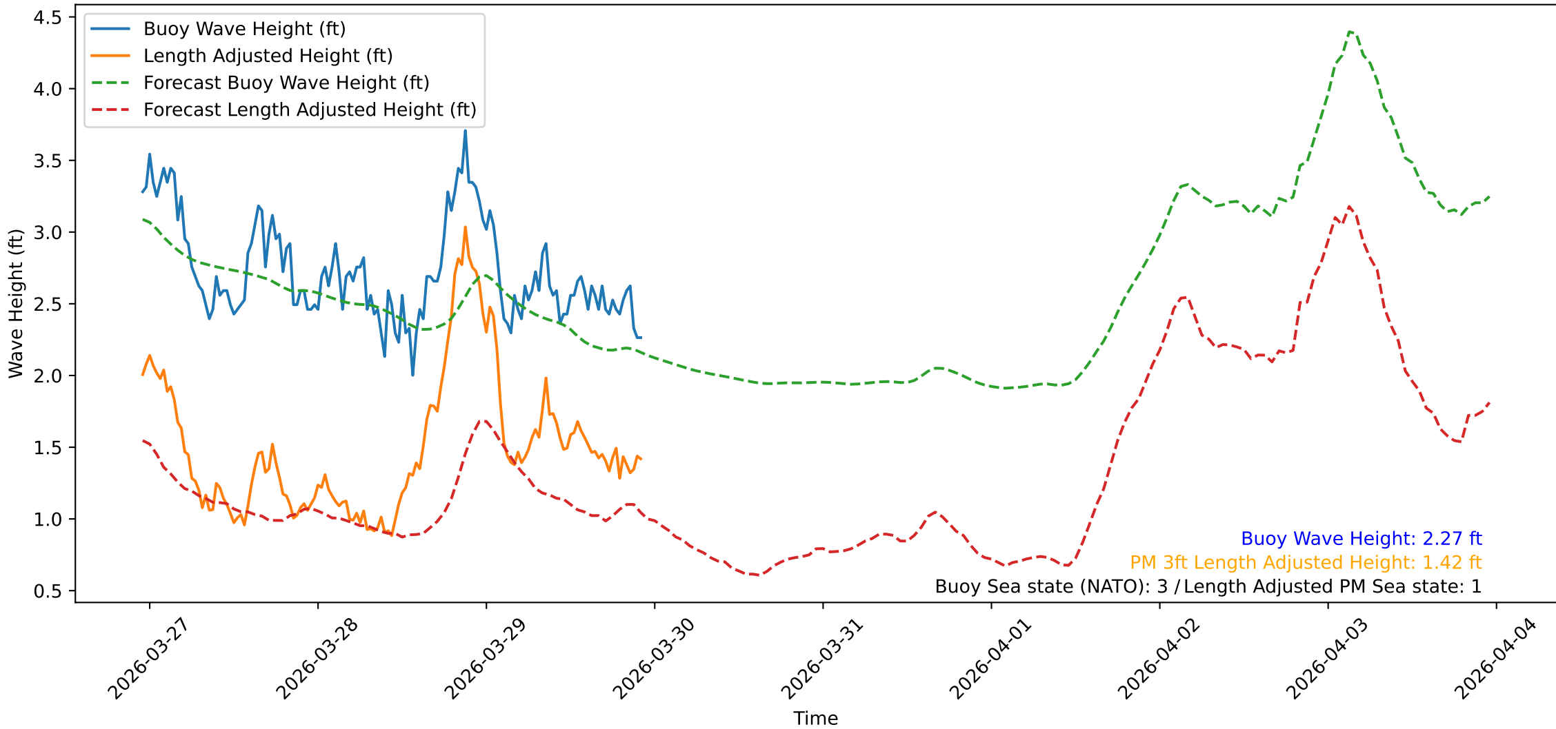
Wave Heights over Time for Green Beach at 2026-03-29 22:51:10
