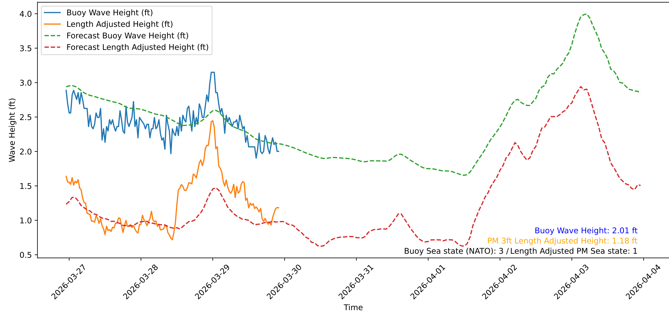
Wave Heights over Time for Oceanside Harbor at 2026-03-29 22:50:31
