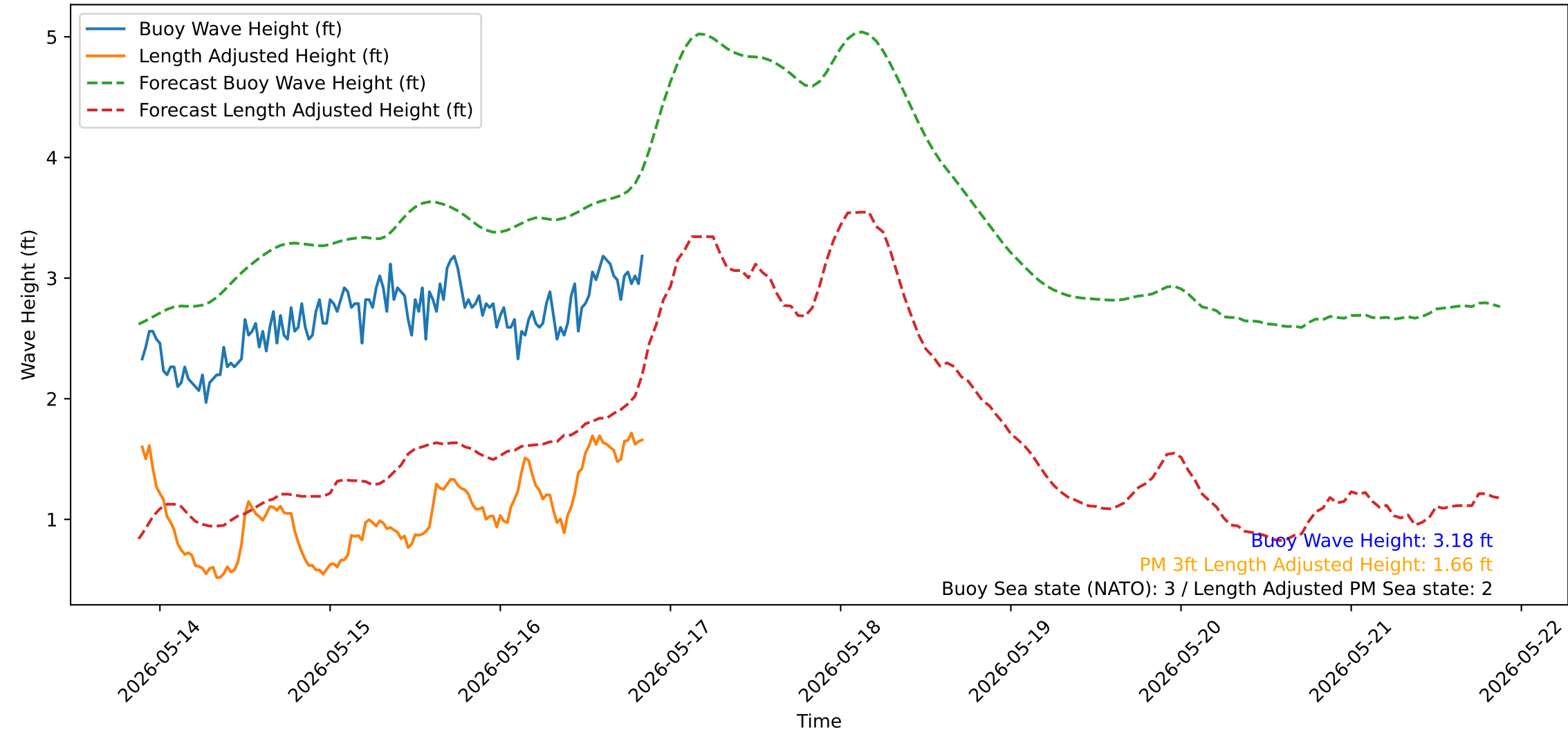
Wave Heights over Time for Red Beach at 2026-05-16 21:00:50
