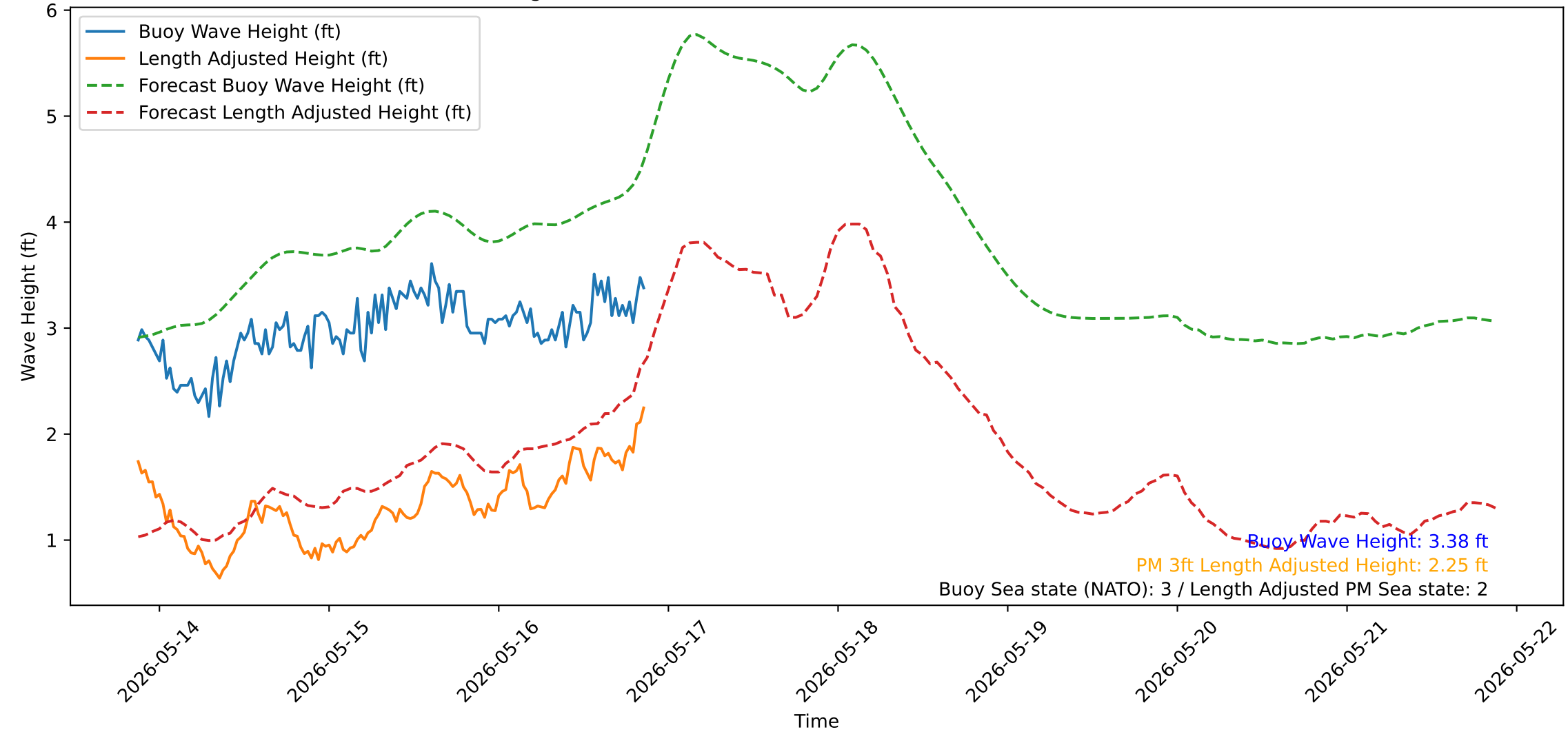
Wave Heights over Time for Oceanside Harbor at 2026-05-16 21:00:31
