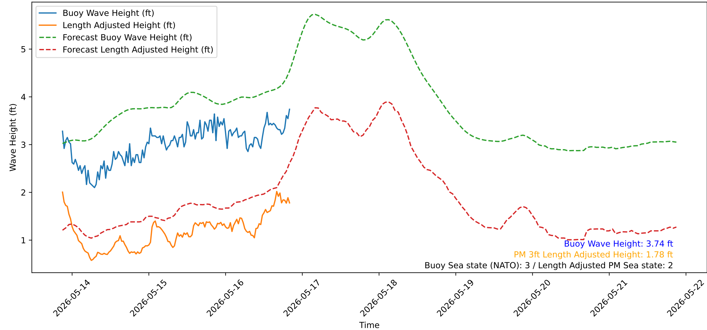
Wave Heights over Time for Green Beach at 2026-05-16 21:01:13
