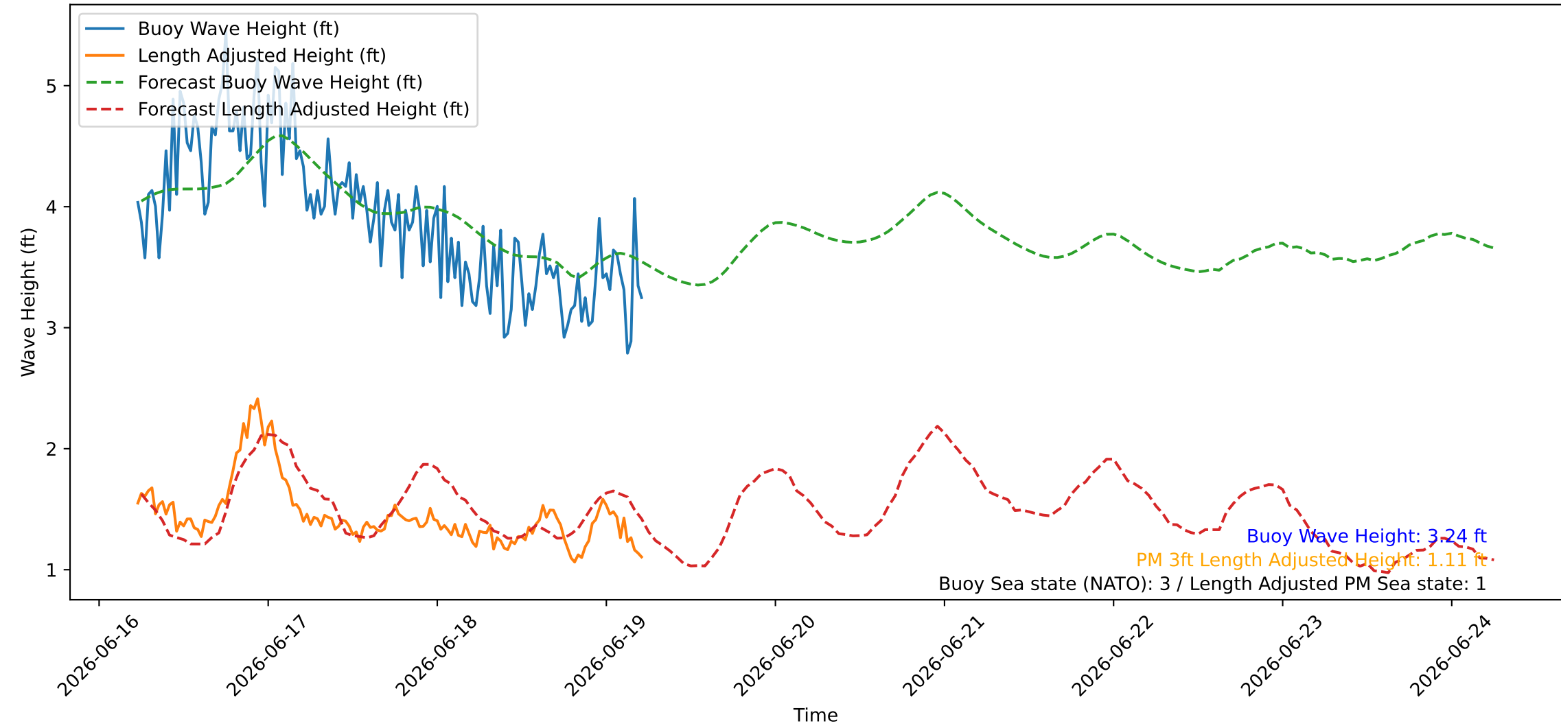
Wave Heights over Time for Oceanside Harbor at 2026-06-19 05:40:26
