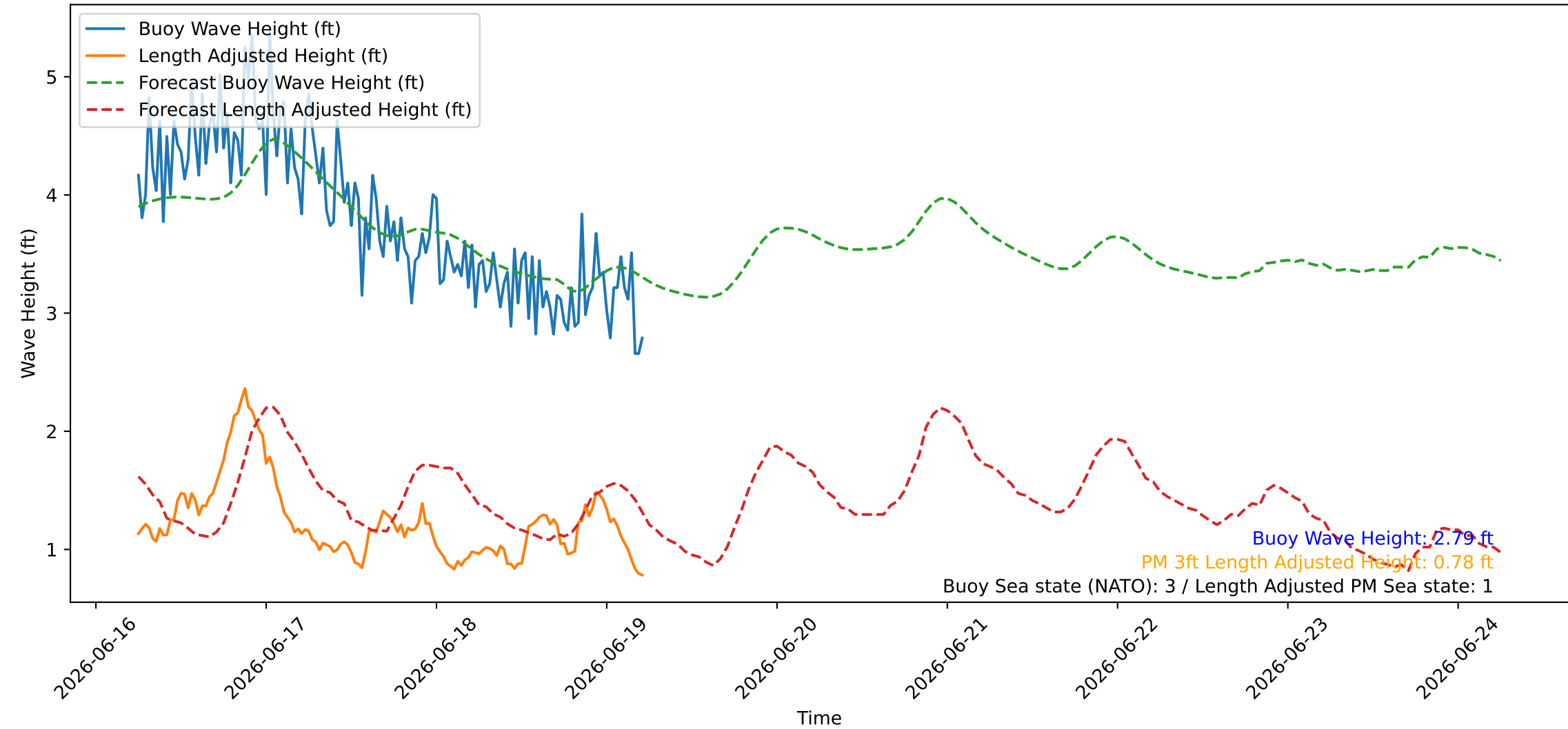
Wave Heights over Time for Red Beach at 2026-06-19 05:40:46
