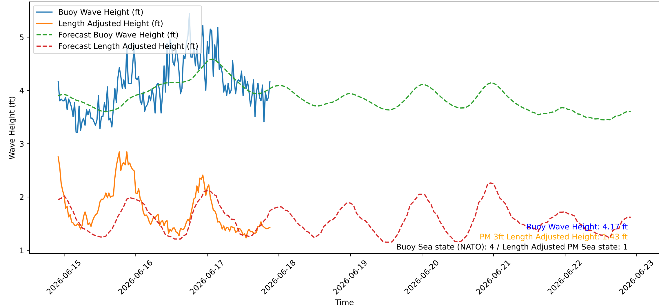
Wave Heights over Time for Oceanside Harbor at 2026-06-17 21:50:26
