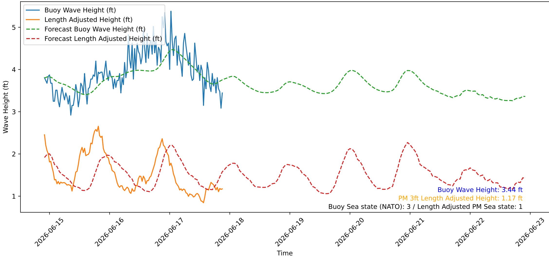
Wave Heights over Time for Red Beach at 2026-06-17 21:50:47
