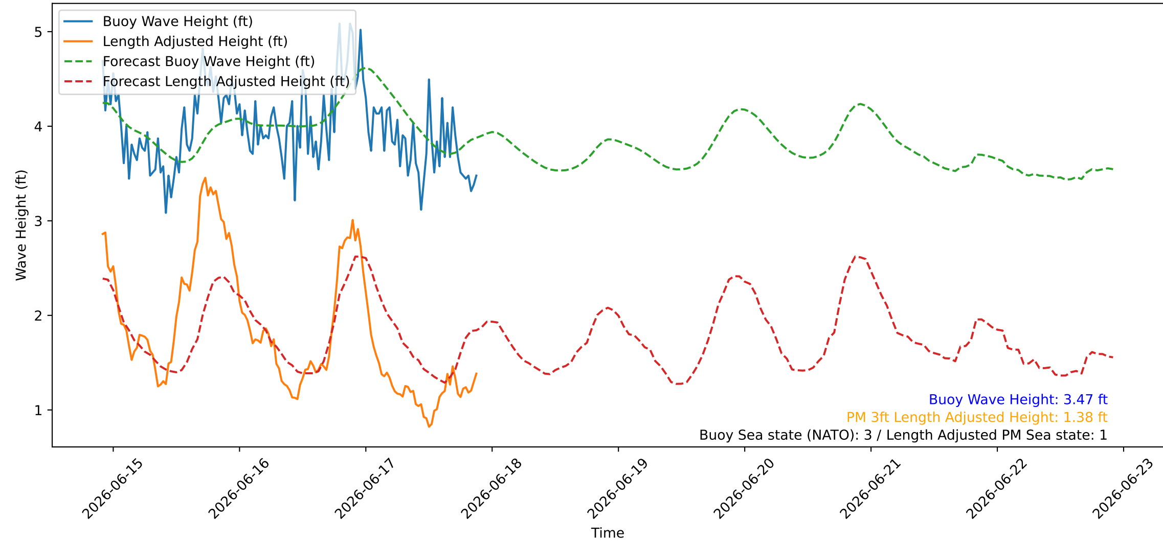
Wave Heights over Time for Green Beach at 2026-06-17 21:51:10
