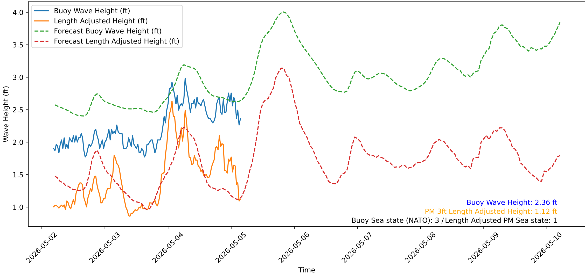
Wave Heights over Time for Green Beach at 2026-05-05 04:31:12
