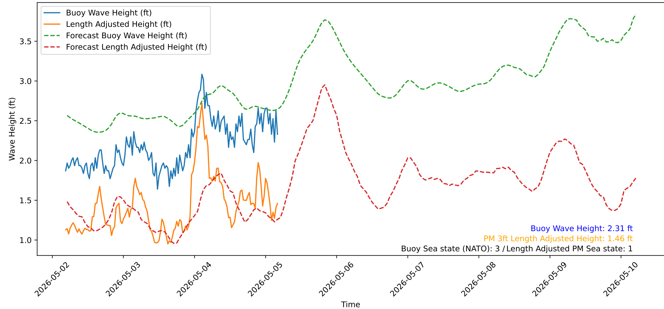
Wave Heights over Time for Oceanside Harbor at 2026-05-05 04:30:31
