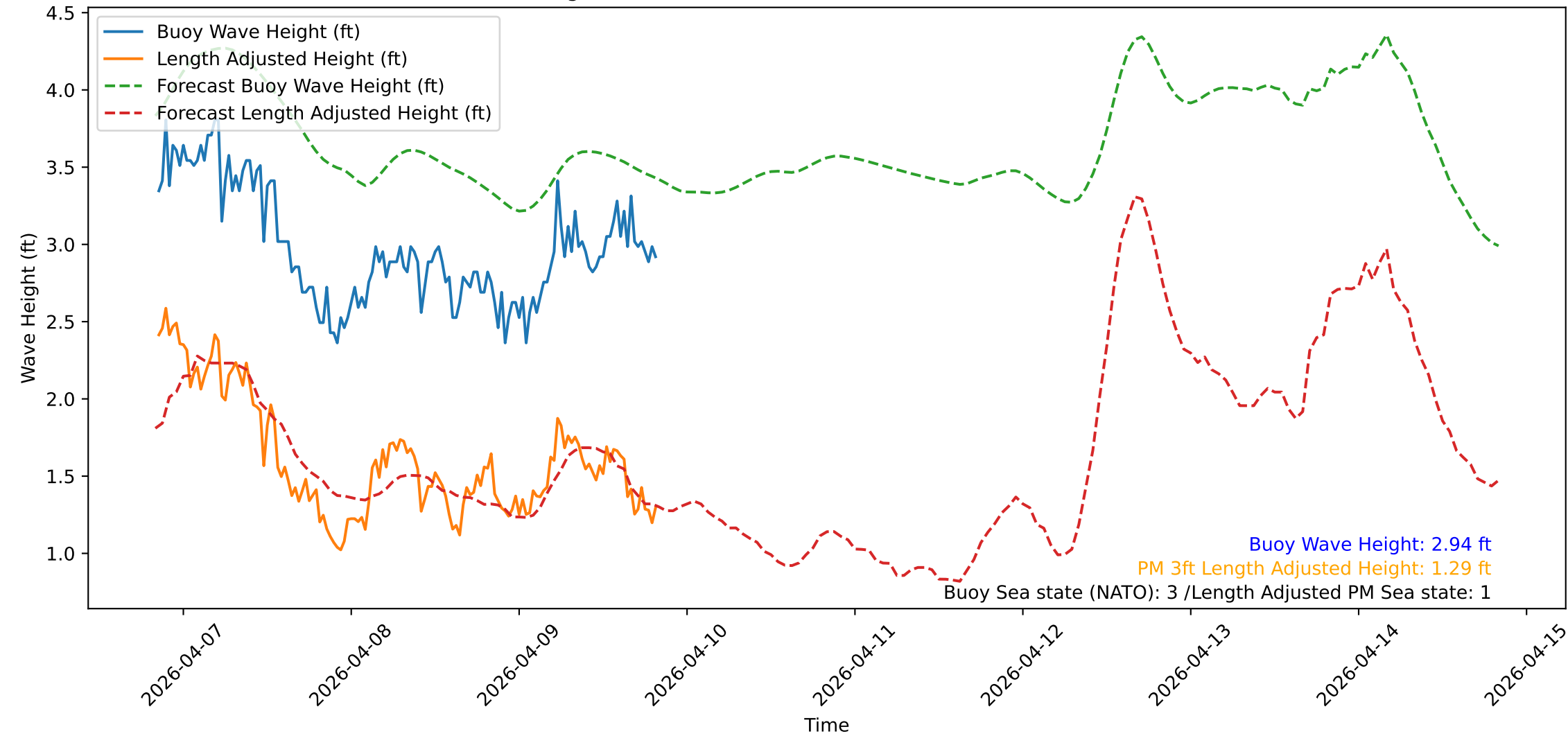
Wave Heights over Time for Green Beach at 2026-04-09 20:21:10
