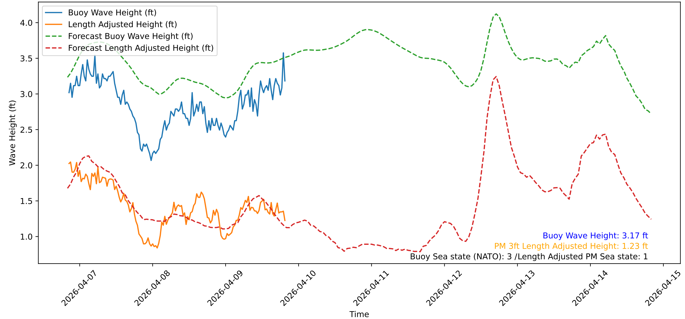
Wave Heights over Time for Red Beach at 2026-04-09 20:20:47
