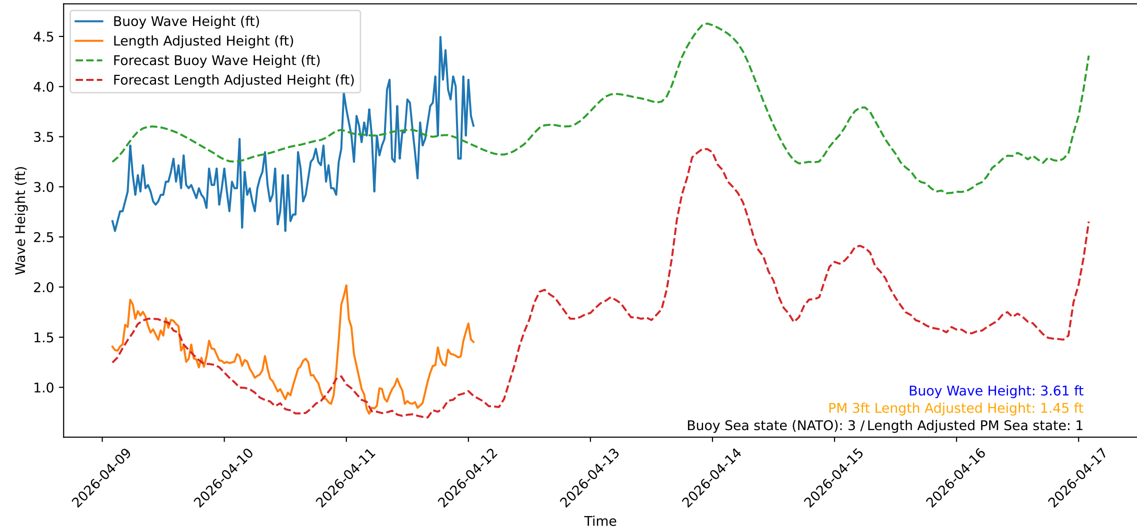
Wave Heights over Time for Green Beach at 2026-04-12 02:01:13
