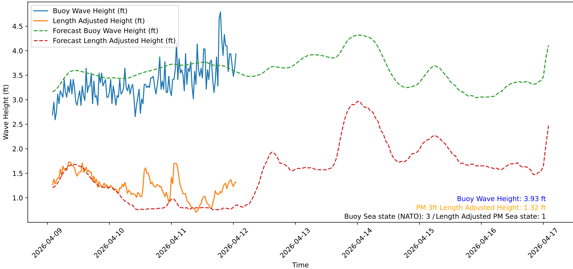
Wave Heights over Time for Oceanside Harbor at 2026-04-12 02:00:31
