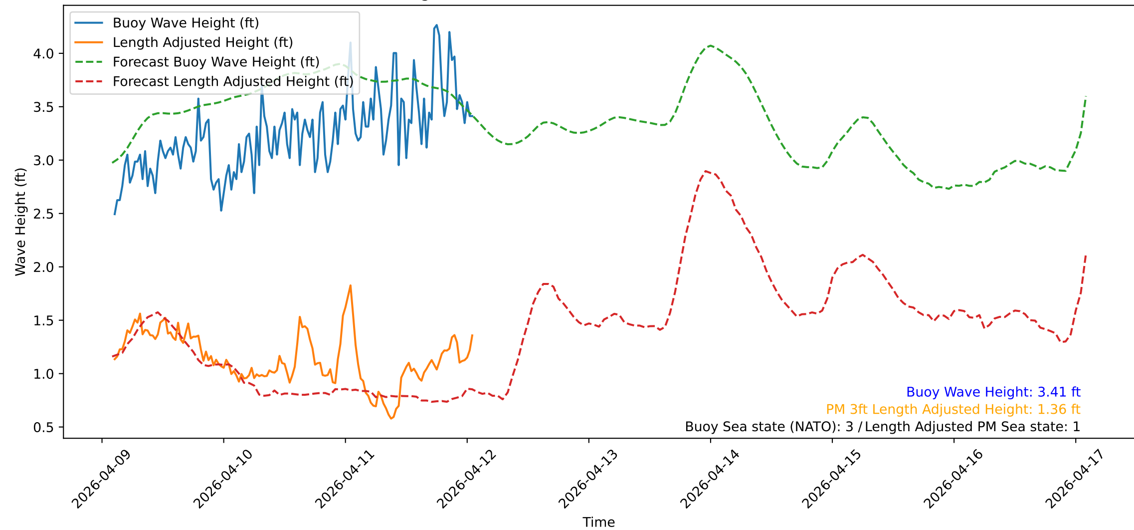
Wave Heights over Time for Red Beach at 2026-04-12 02:00:51
