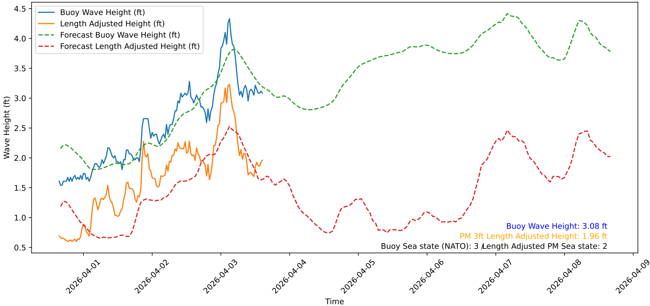
Wave Heights over Time for Green Beach at 2026-04-03 15:31:11
