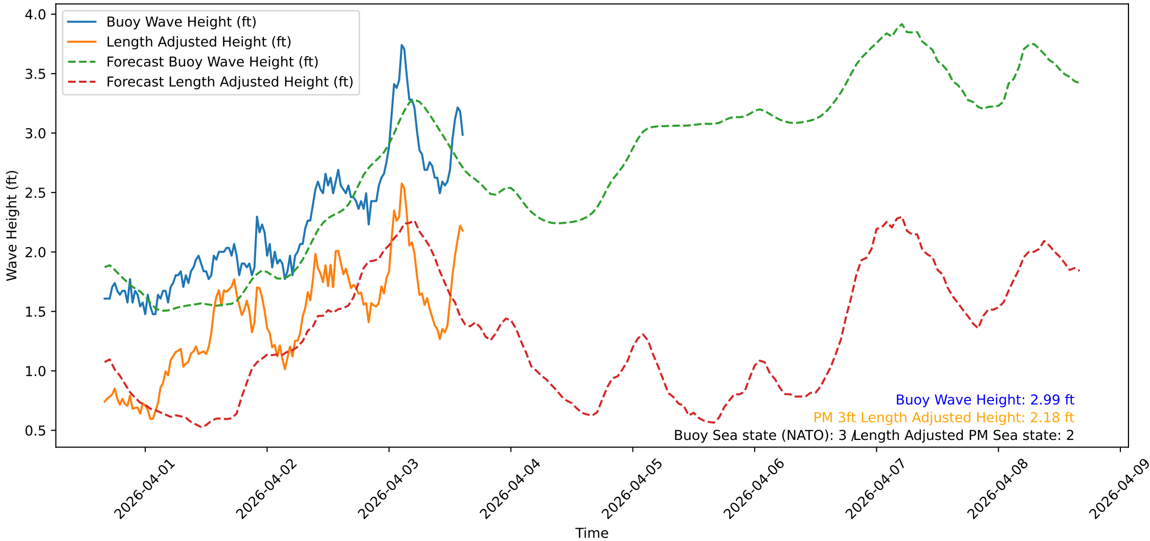
Wave Heights over Time for Red Beach at 2026-04-03 15:30:48
