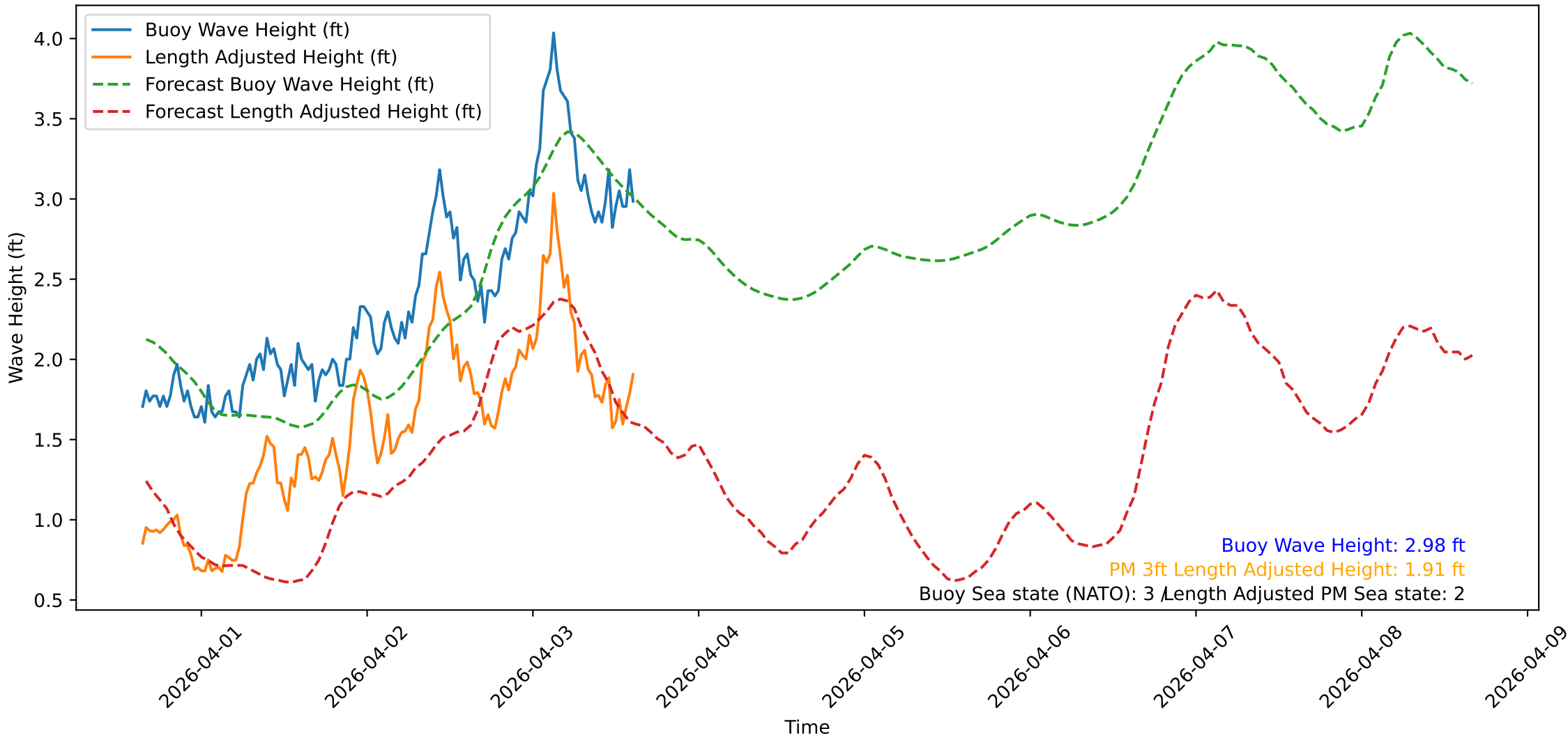
Wave Heights over Time for Oceanside Harbor at 2026-04-03 15:30:32
