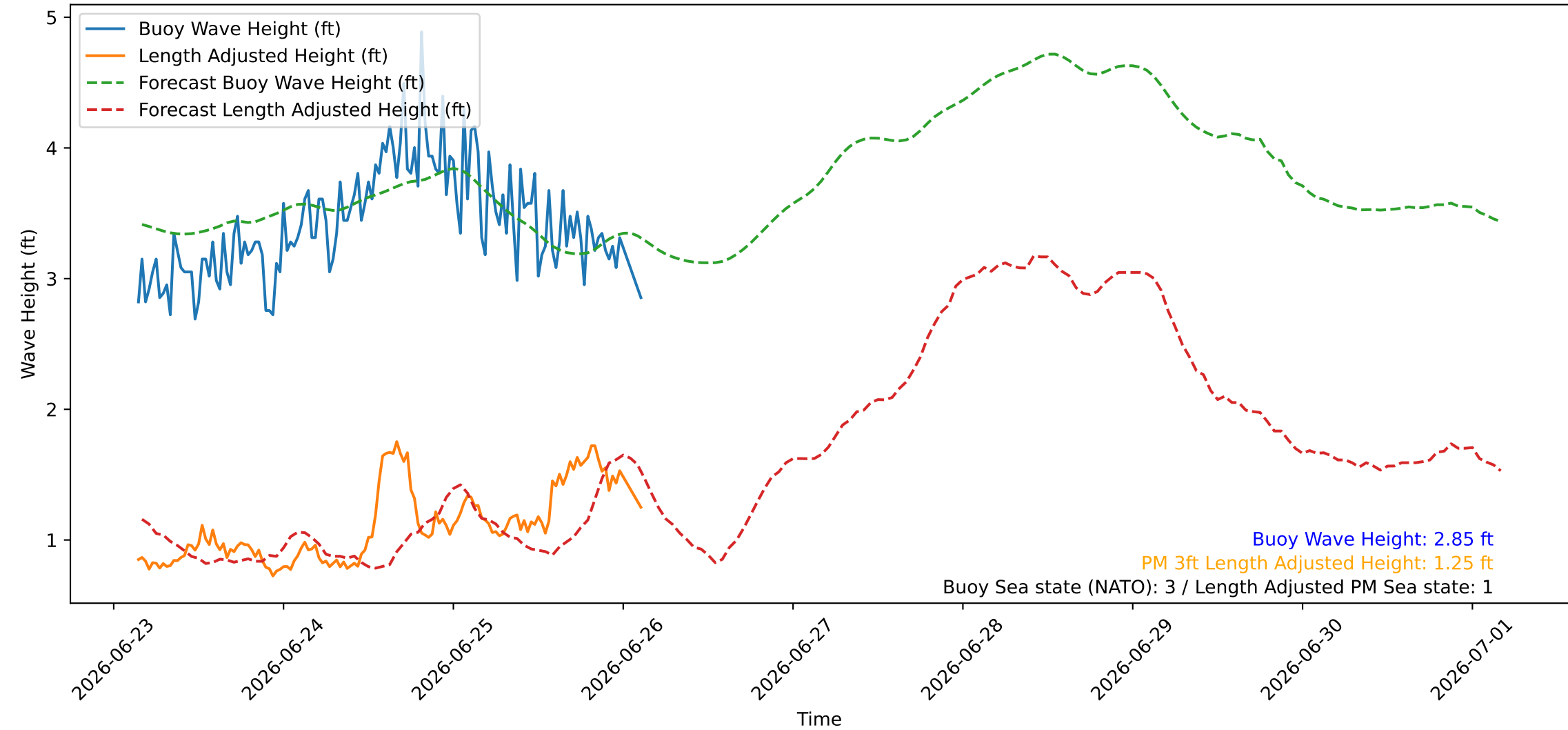
Wave Heights over Time for Oceanside Harbor at 2026-06-26 03:40:26
