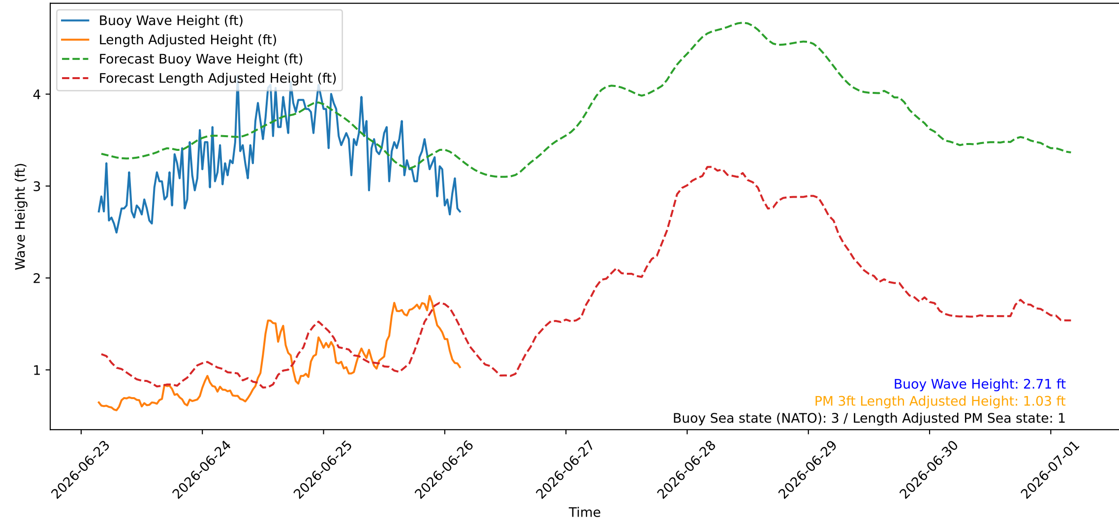
Wave Heights over Time for Green Beach at 2026-06-26 03:41:07
