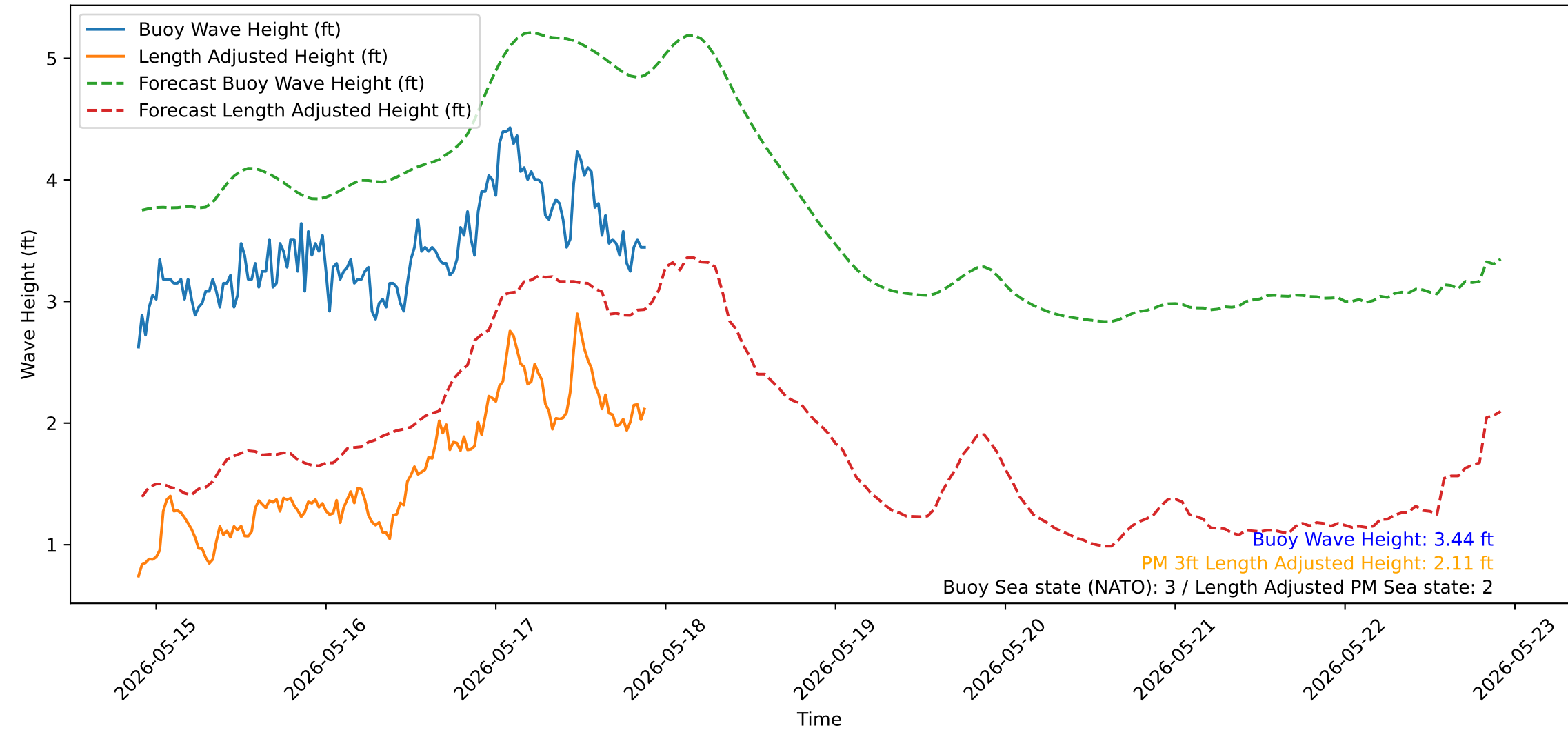
Wave Heights over Time for Green Beach at 2026-05-17 21:41:15
