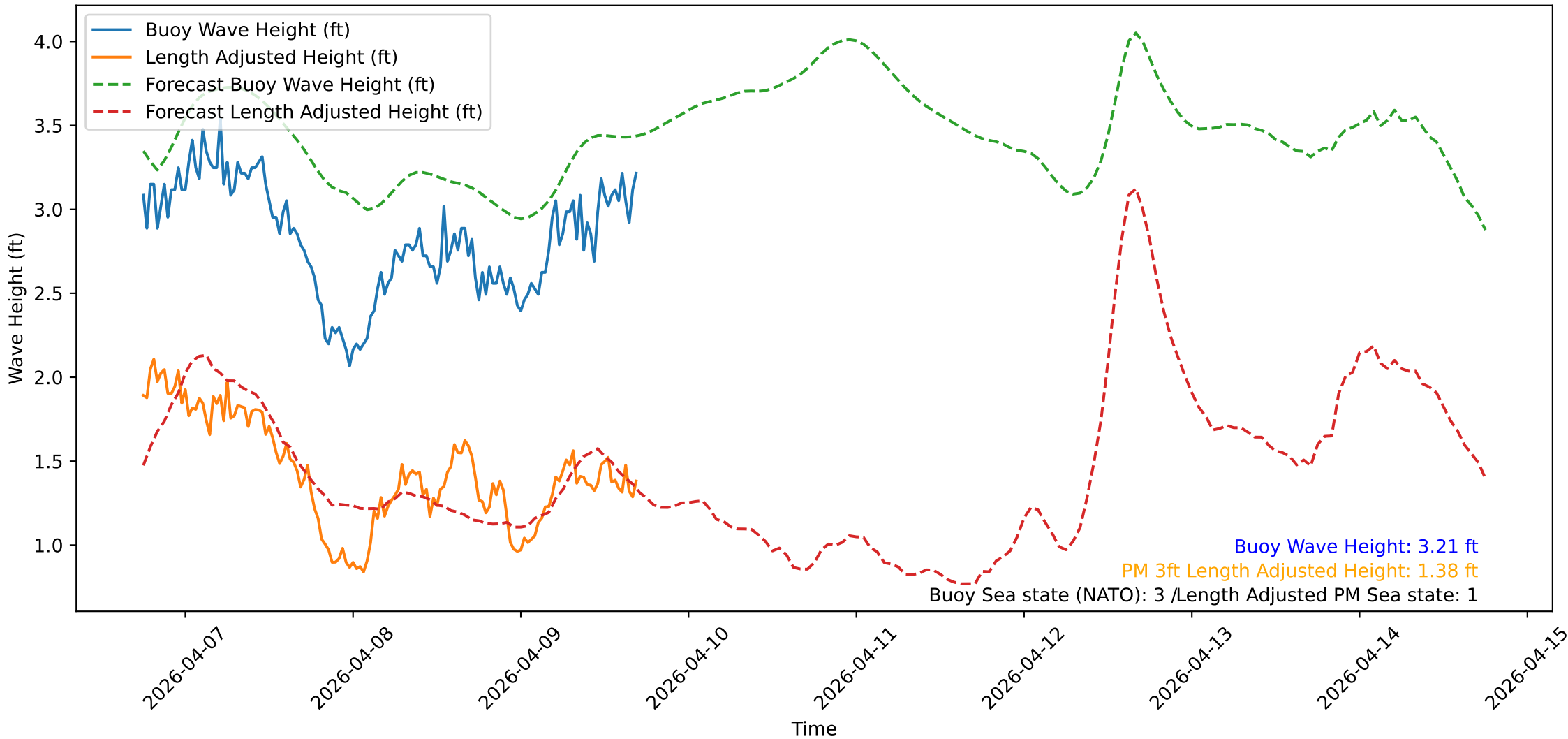
Wave Heights over Time for Red Beach at 2026-04-09 17:30:47
