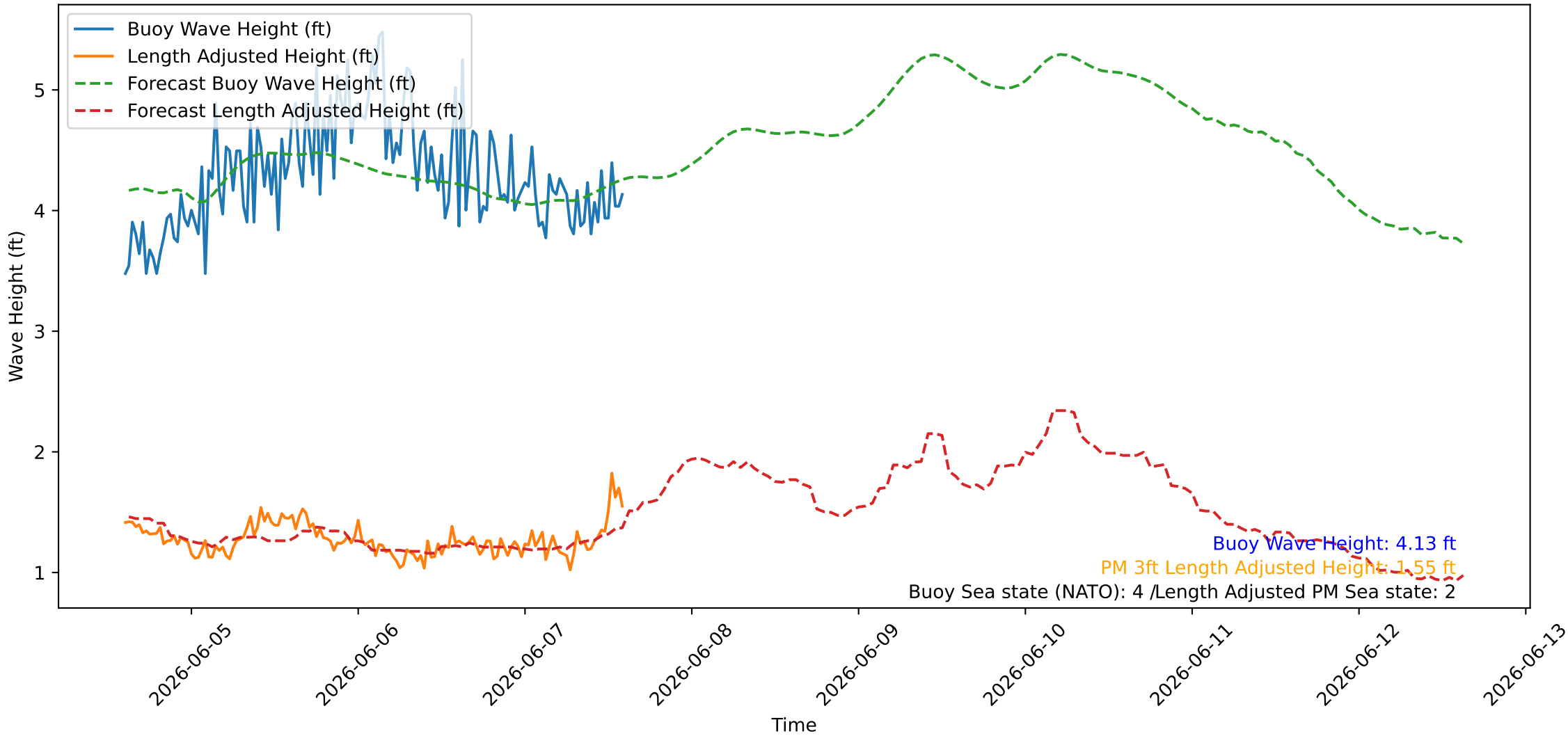
Wave Heights over Time for Oceanside Harbor at 2026-06-07 14:40:26
