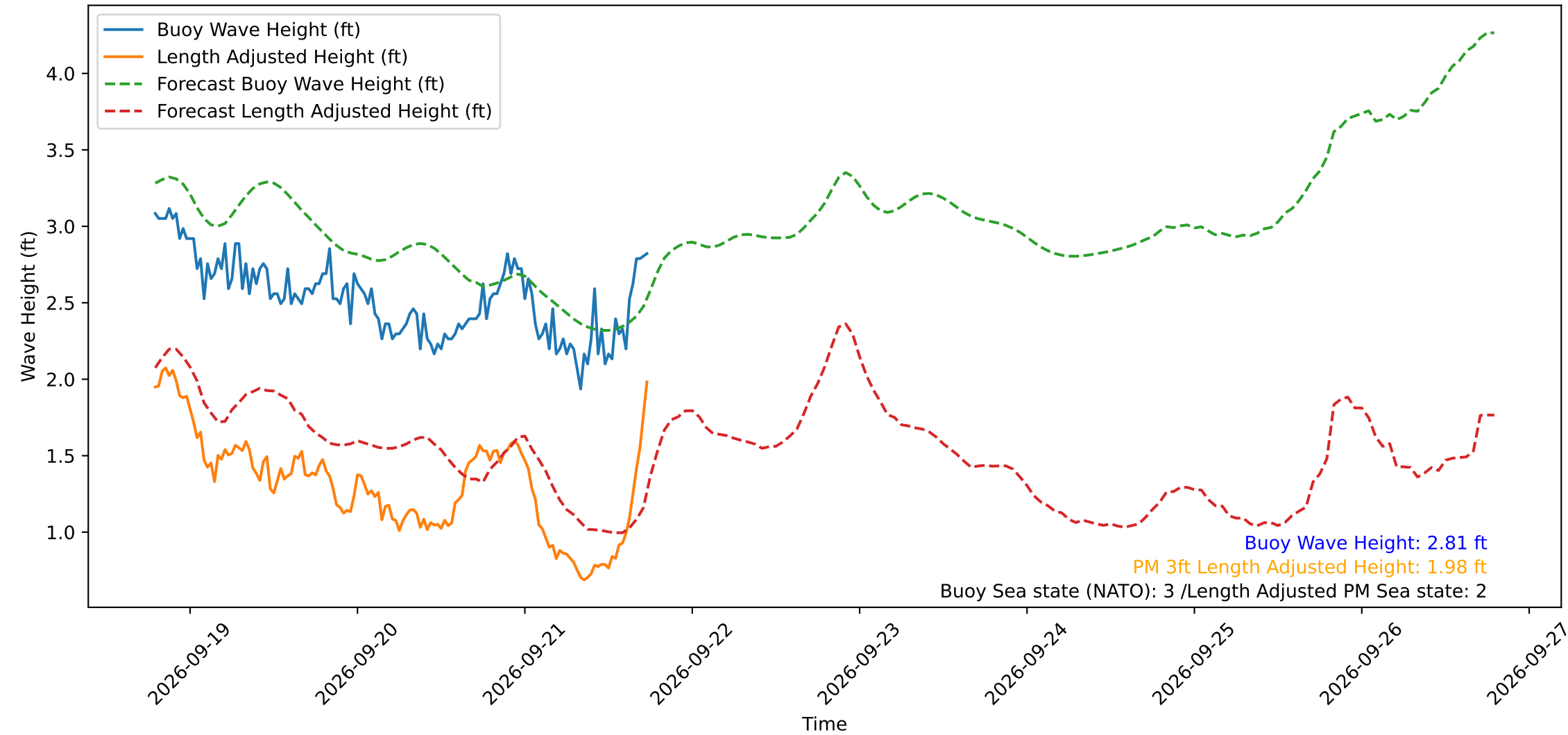
Wave Heights over Time for Green Beach at 2026-09-21 18:31:12
