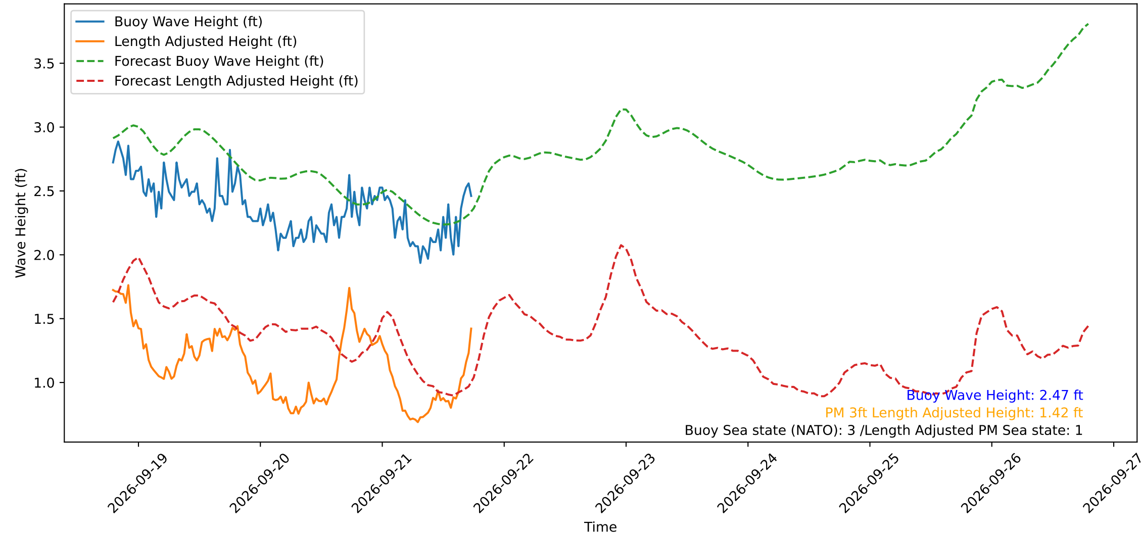
Wave Heights over Time for Red Beach at 2026-09-21 18:30:49
