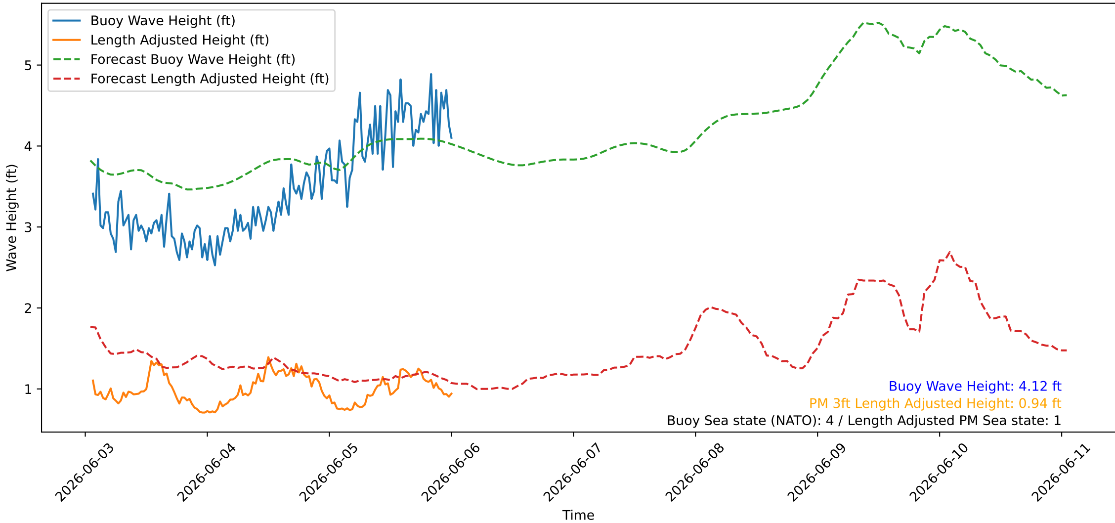
Wave Heights over Time for Red Beach at 2026-06-06 01:00:46
