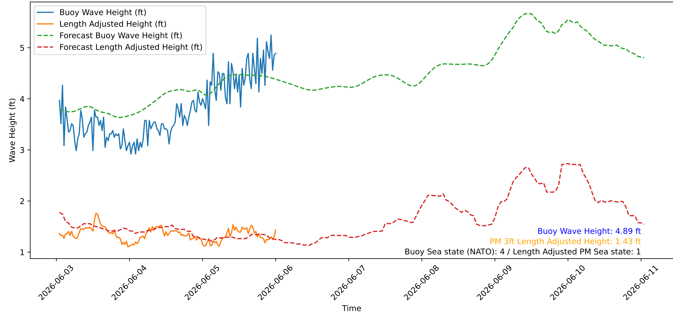
Wave Heights over Time for Oceanside Harbor at 2026-06-06 01:00:26
