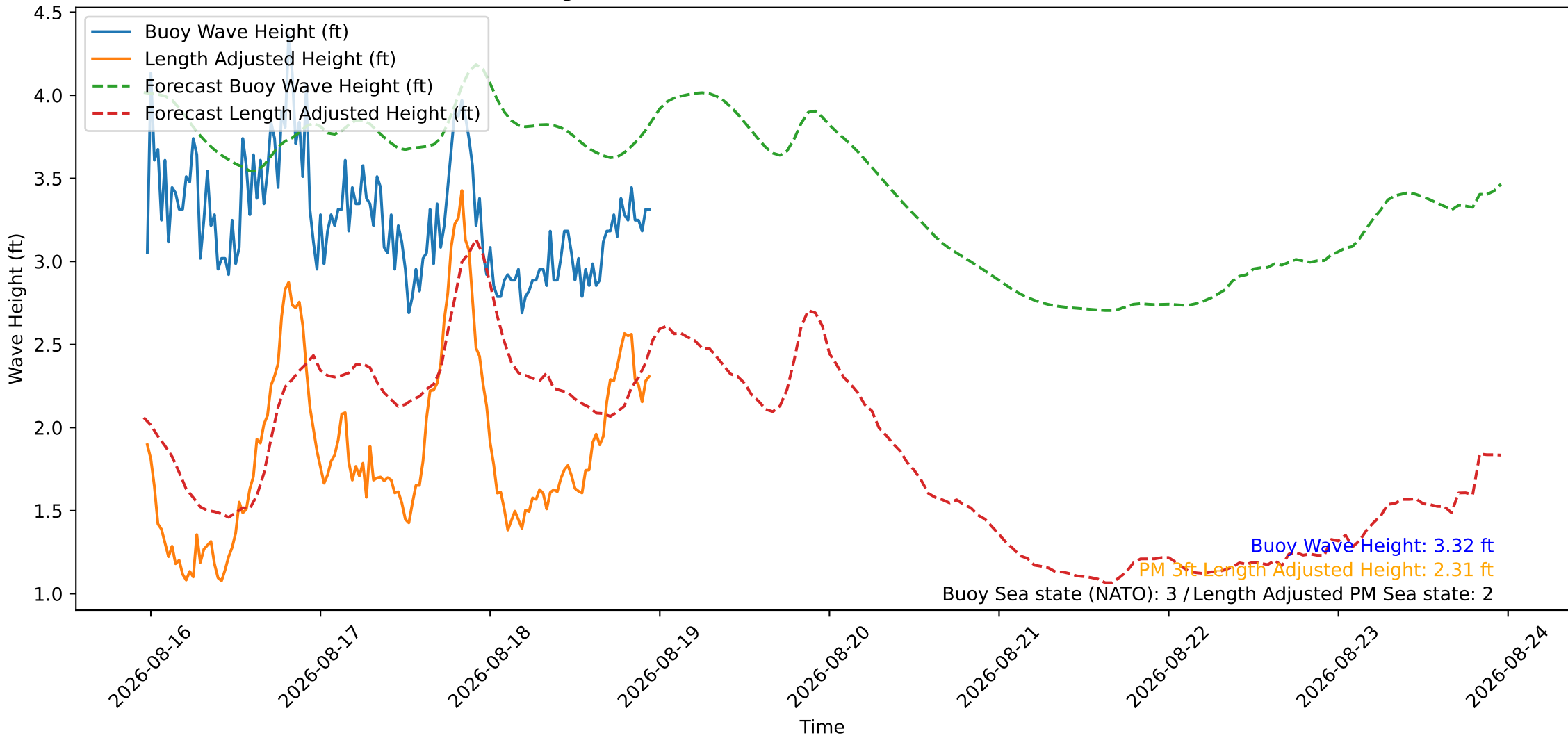
Wave Heights over Time for Green Beach at 2026-08-18 23:21:11
