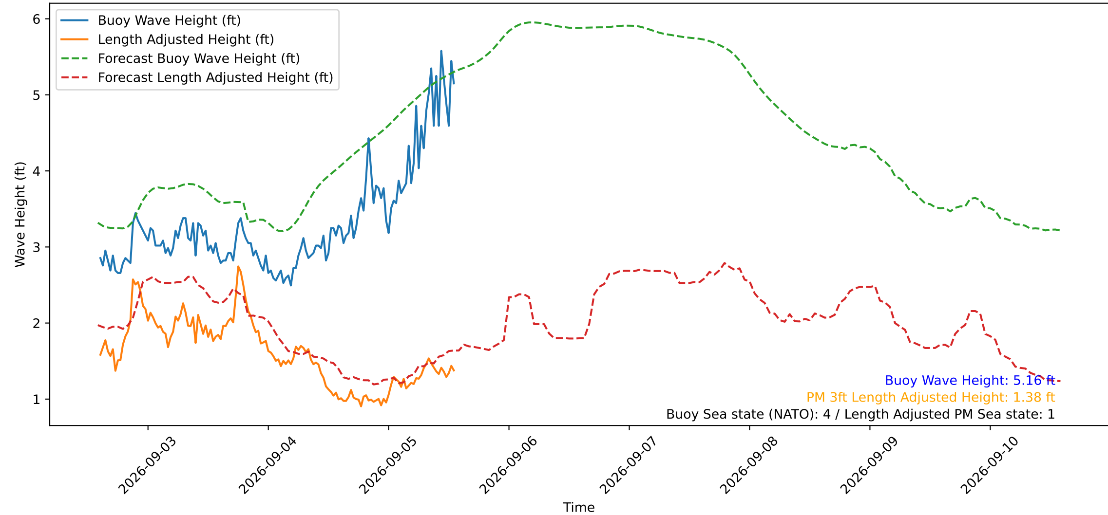
Wave Heights over Time for Green Beach at 2026-09-05 14:01:12
