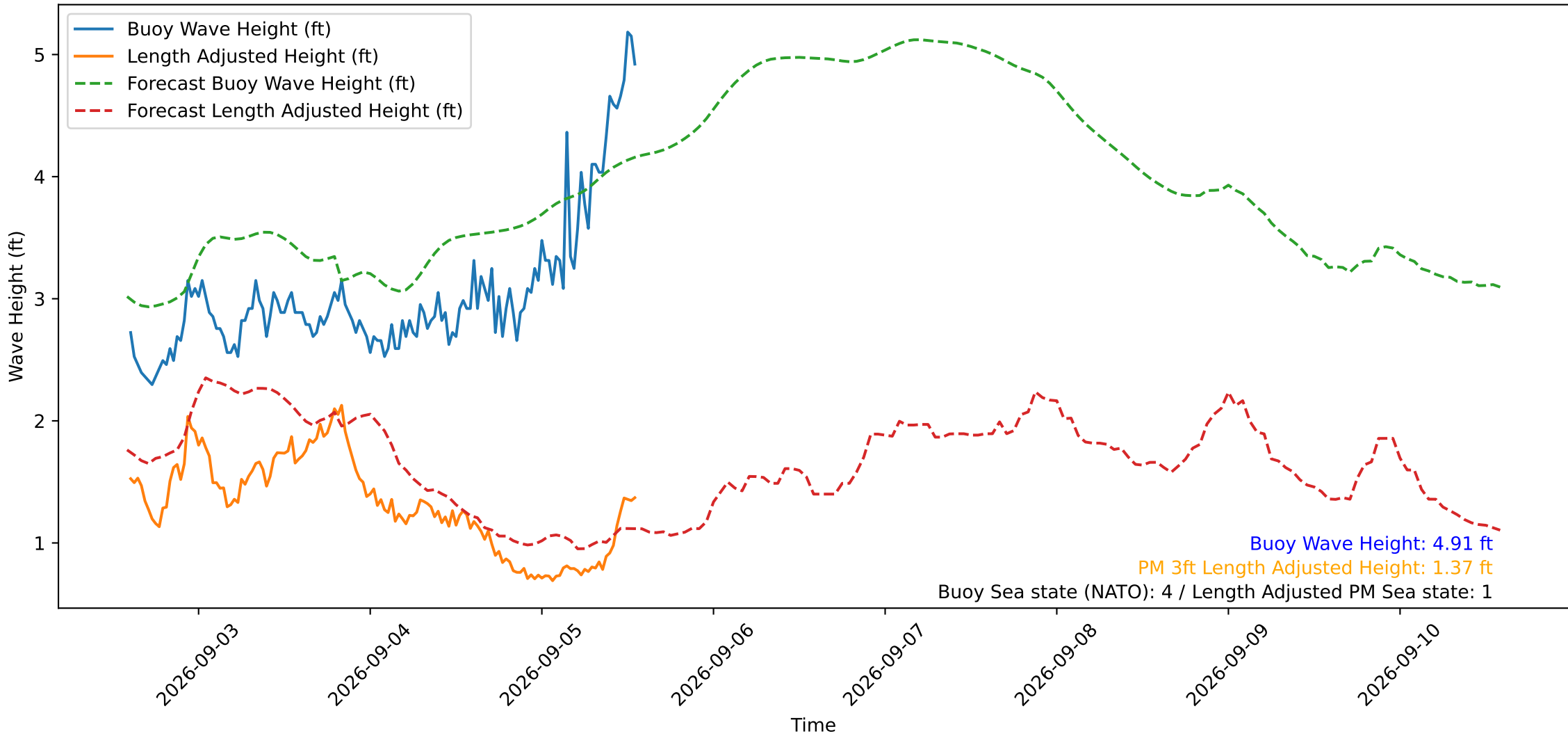
Wave Heights over Time for Red Beach at 2026-09-05 14:00:49
