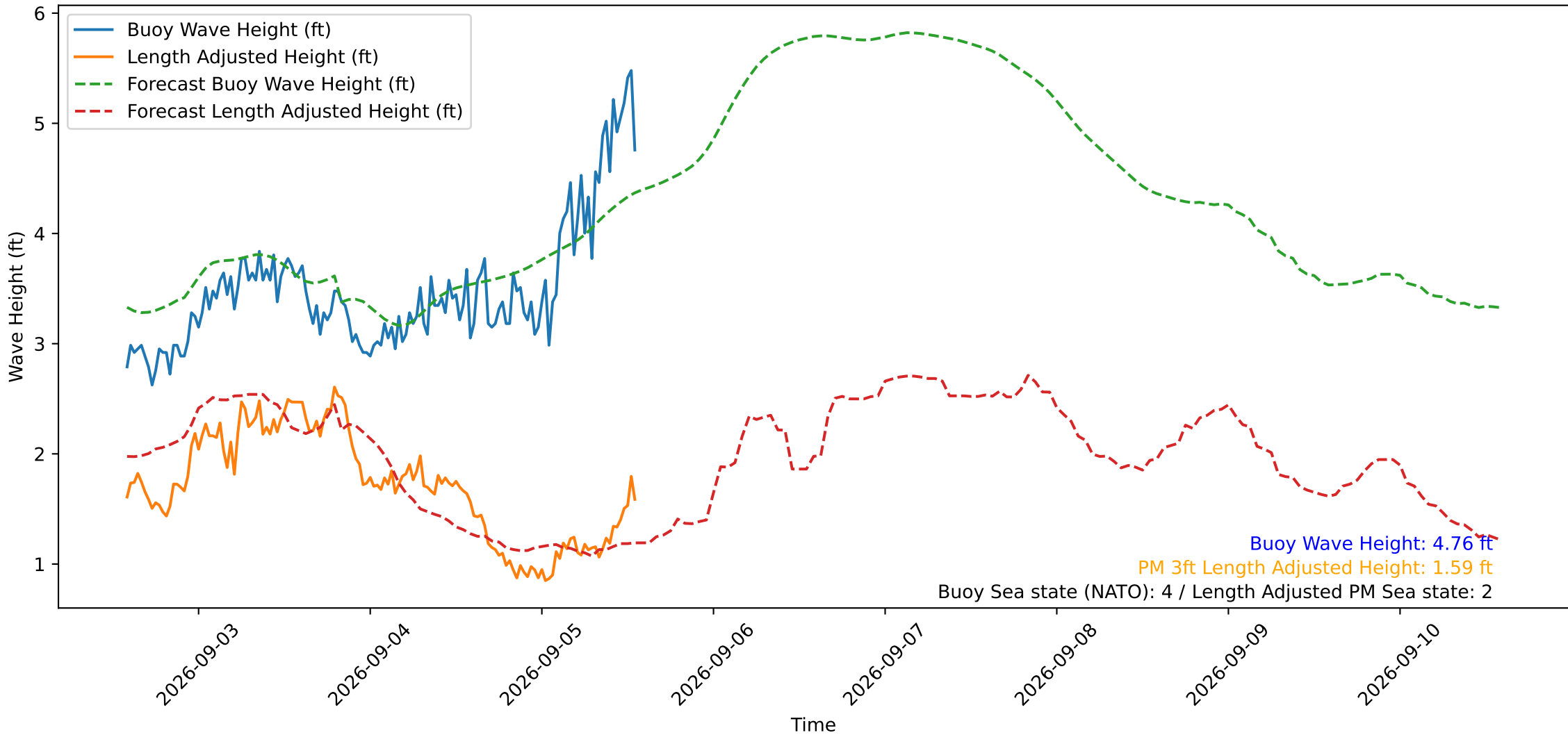
Wave Heights over Time for Oceanside Harbor at 2026-09-05 14:00:29
