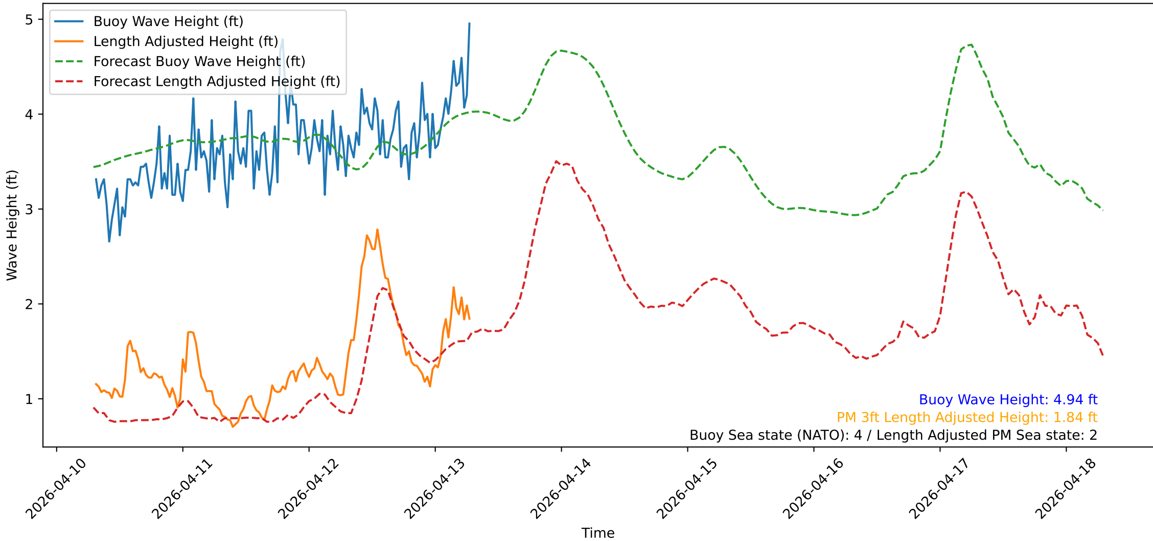
Wave Heights over Time for Oceanside Harbor at 2026-04-13 07:20:32
