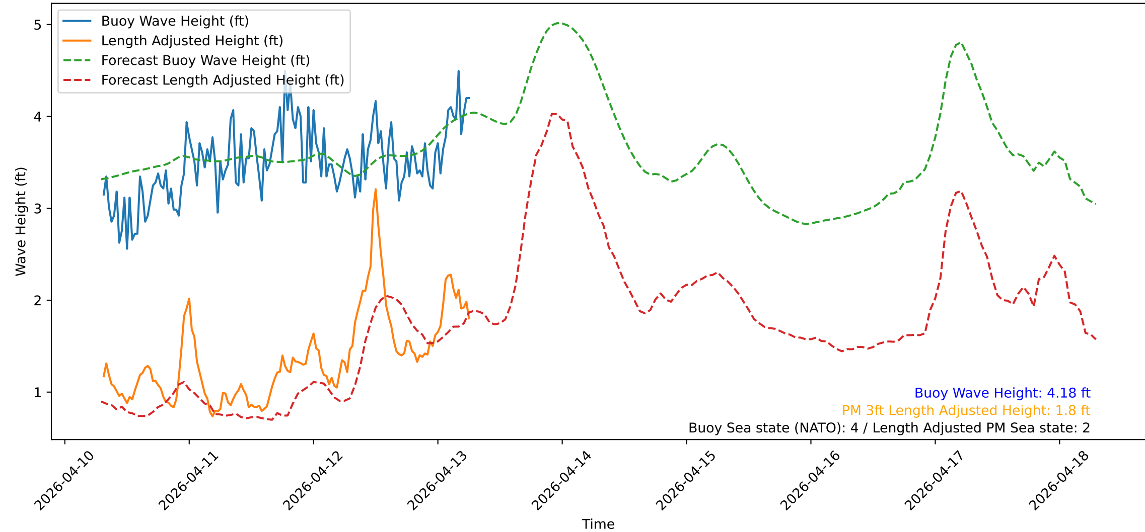
Wave Heights over Time for Green Beach at 2026-04-13 07:21:14
