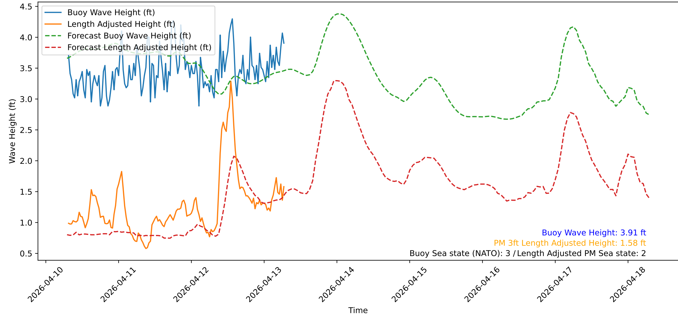
Wave Heights over Time for Red Beach at 2026-04-13 07:20:52
