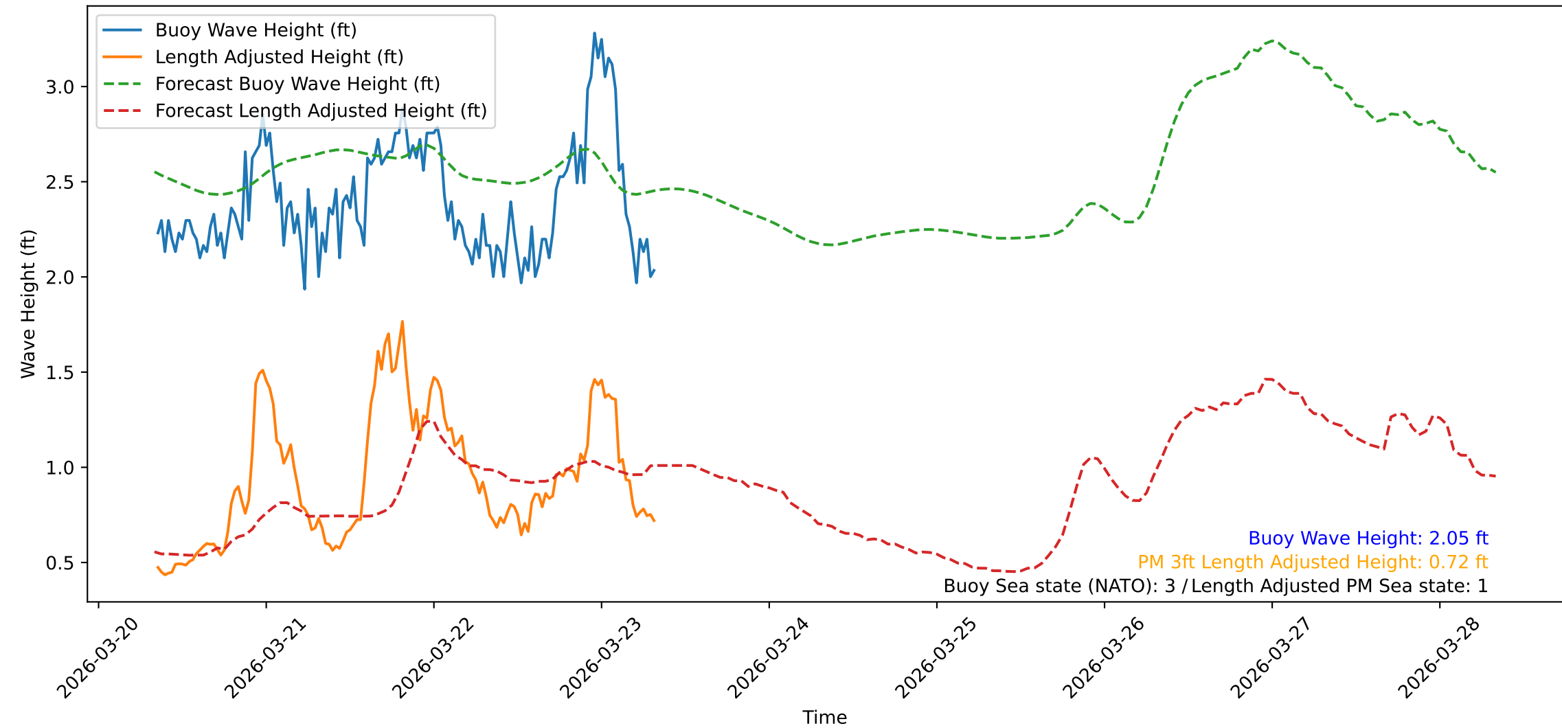
Wave Heights over Time for Green Beach at 2026-03-23 08:21:09
