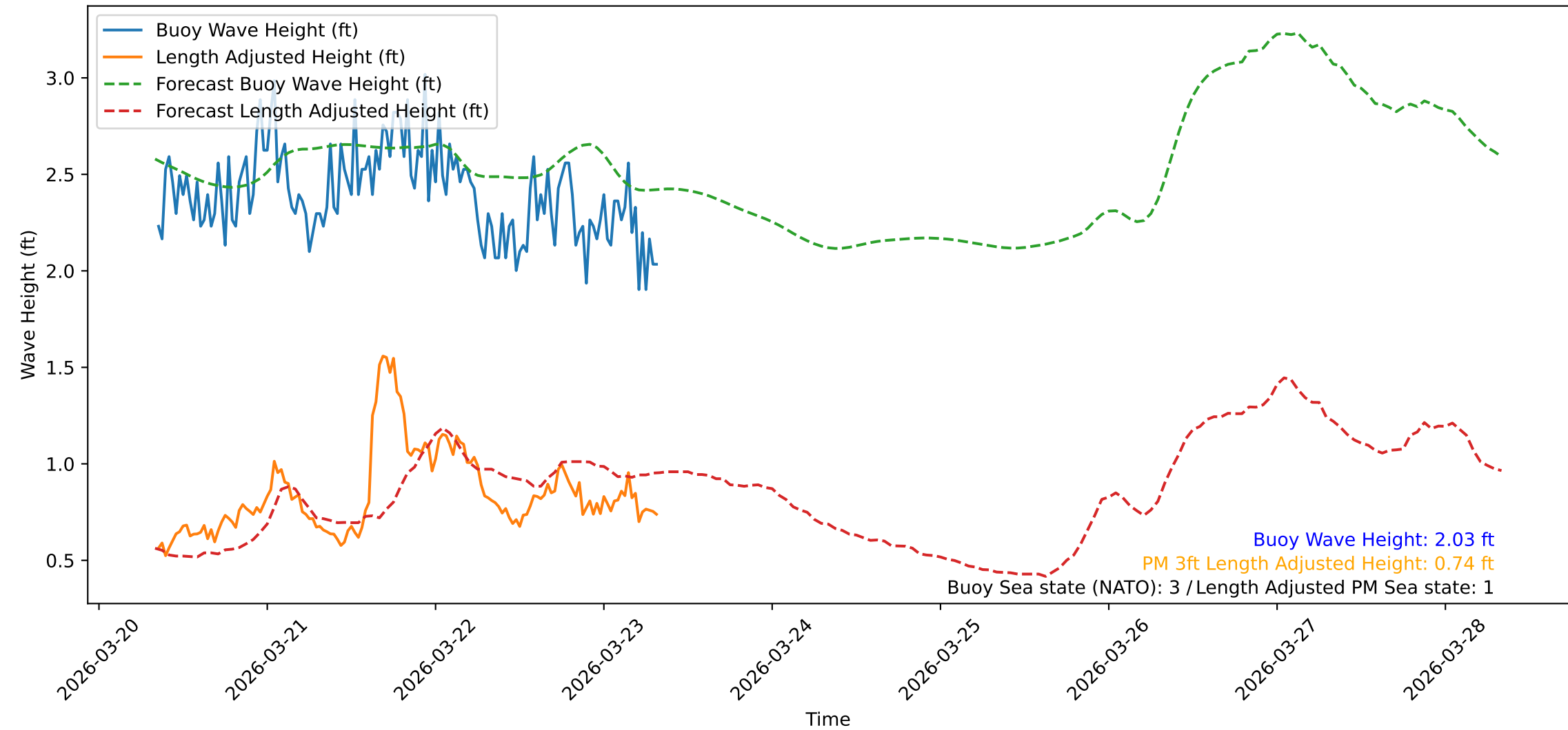
Wave Heights over Time for Oceanside Harbor at 2026-03-23 08:20:31
