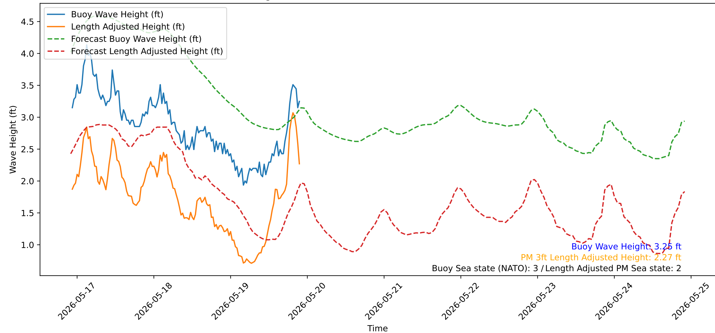
Wave Heights over Time for Red Beach at 2026-05-19 22:10:51
