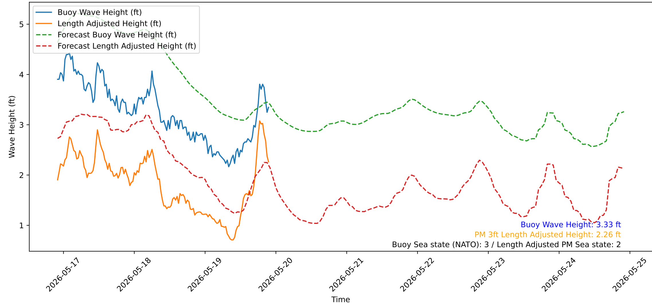
Wave Heights over Time for Green Beach at 2026-05-19 22:11:13
