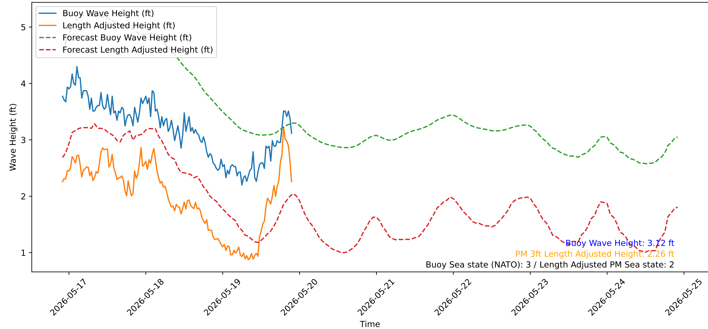
Wave Heights over Time for Oceanside Harbor at 2026-05-19 22:10:31
