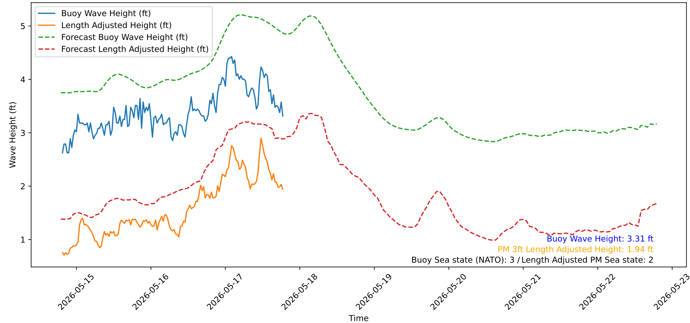
Wave Heights over Time for Green Beach at 2026-05-17 19:21:13
