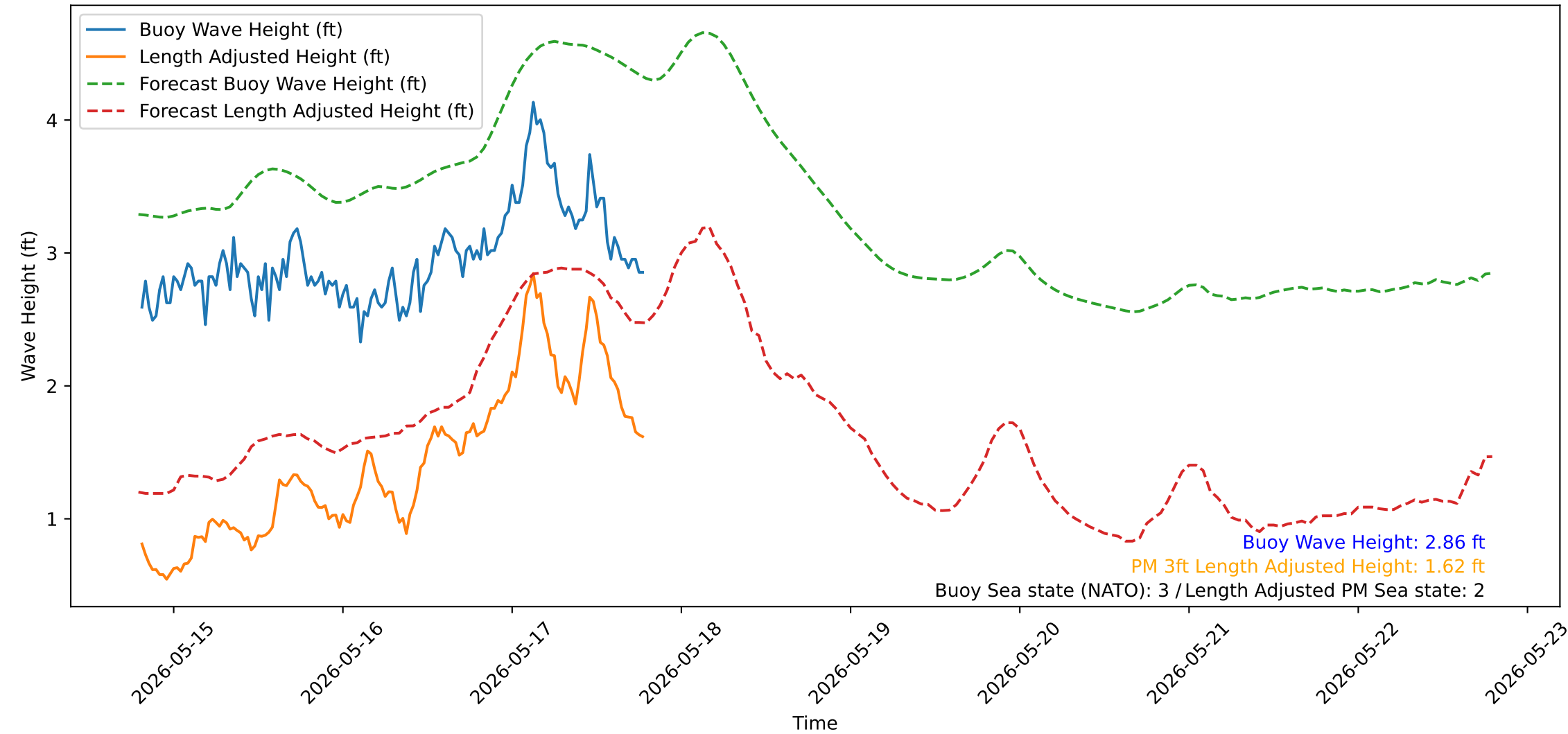
Wave Heights over Time for Red Beach at 2026-05-17 19:20:51
