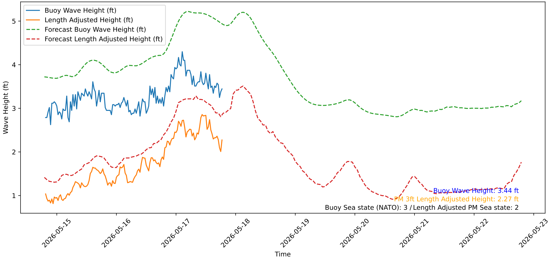
Wave Heights over Time for Oceanside Harbor at 2026-05-17 19:20:31
