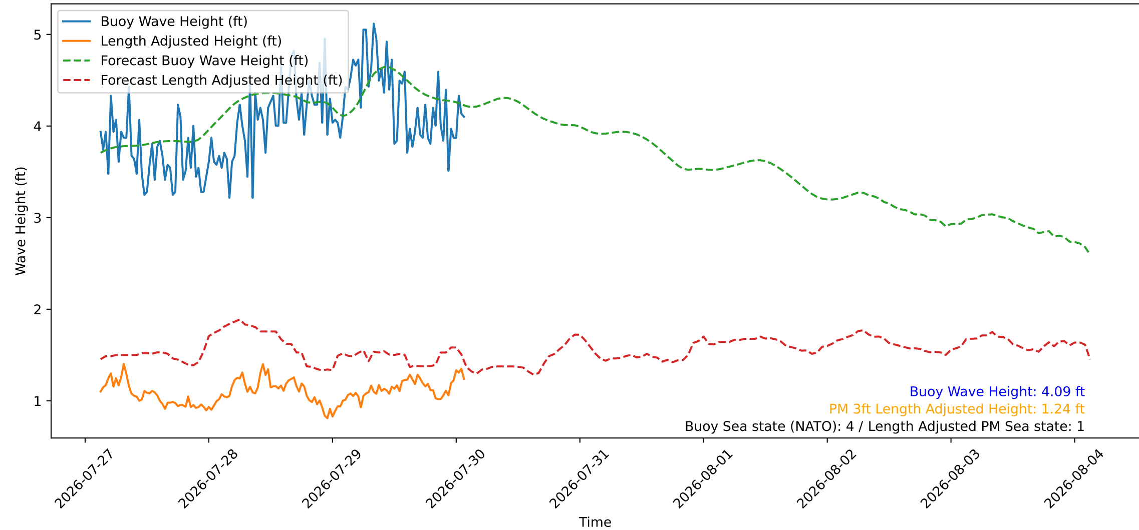
Wave Heights over Time for Red Beach at 2026-07-30 02:30:46
