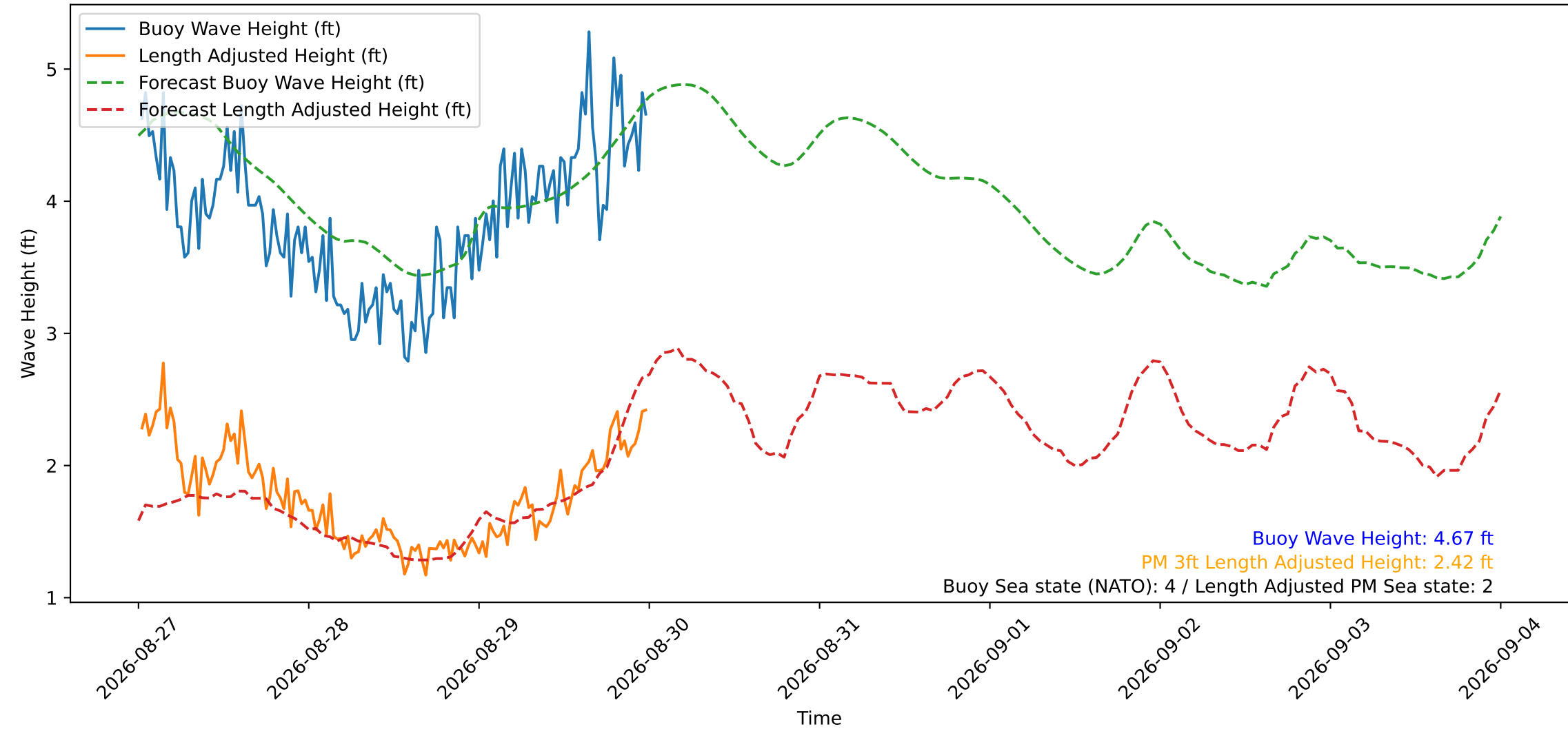
Wave Heights over Time for Oceanside Harbor at 2026-08-30 00:20:30
