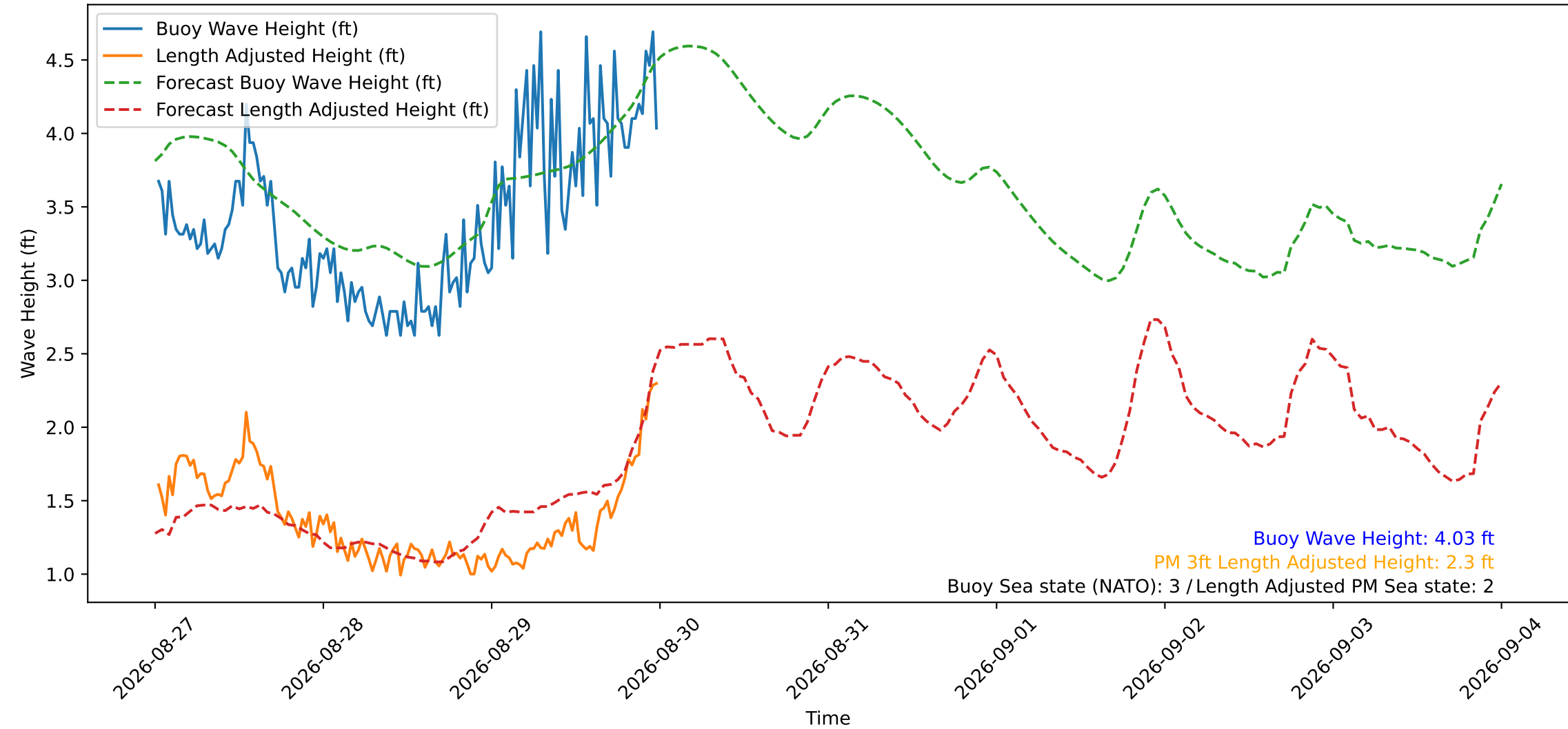
Wave Heights over Time for Red Beach at 2026-08-30 00:20:51
