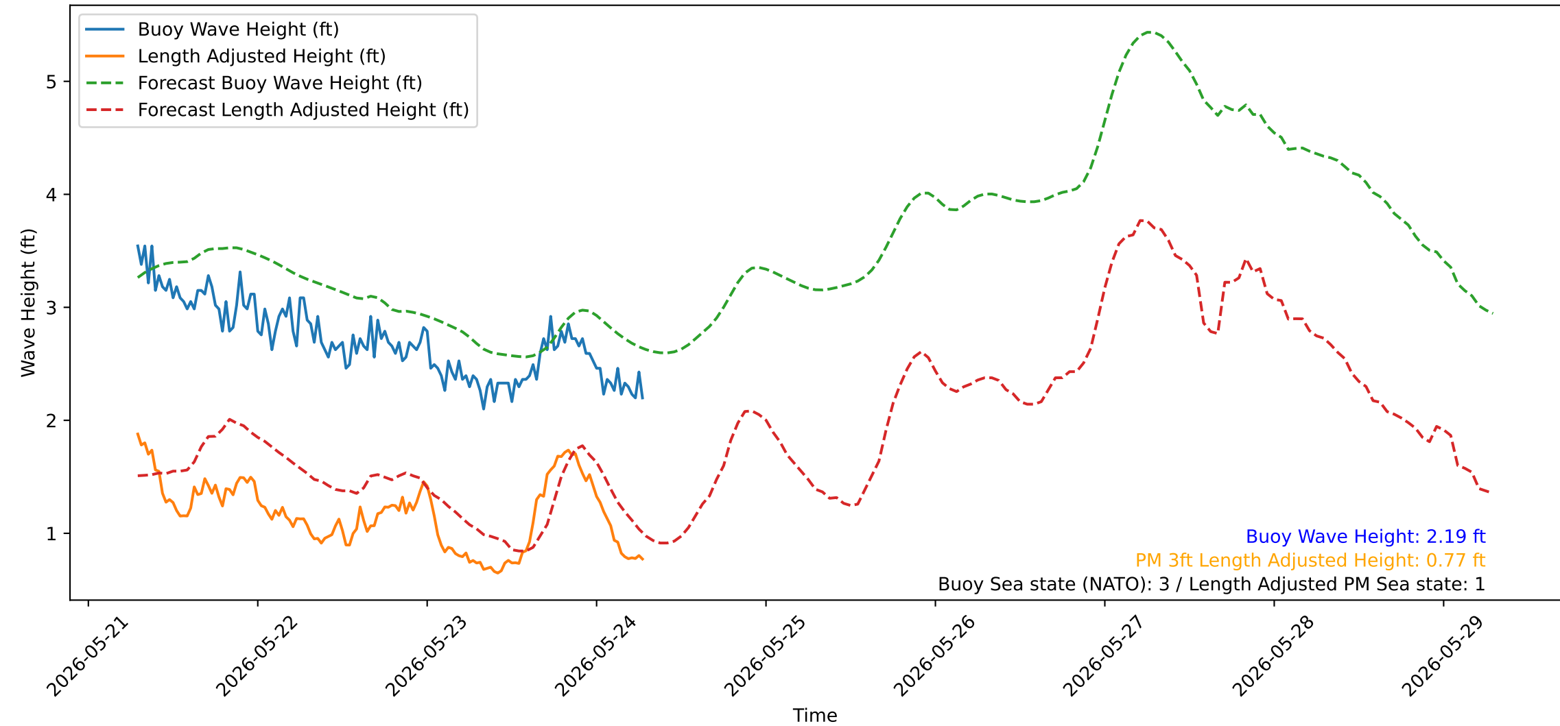
Wave Heights over Time for Green Beach at 2026-05-24 07:11:14
