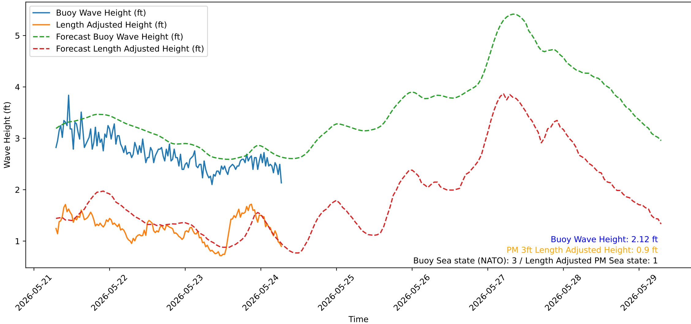
Wave Heights over Time for Oceanside Harbor at 2026-05-24 07:10:32
