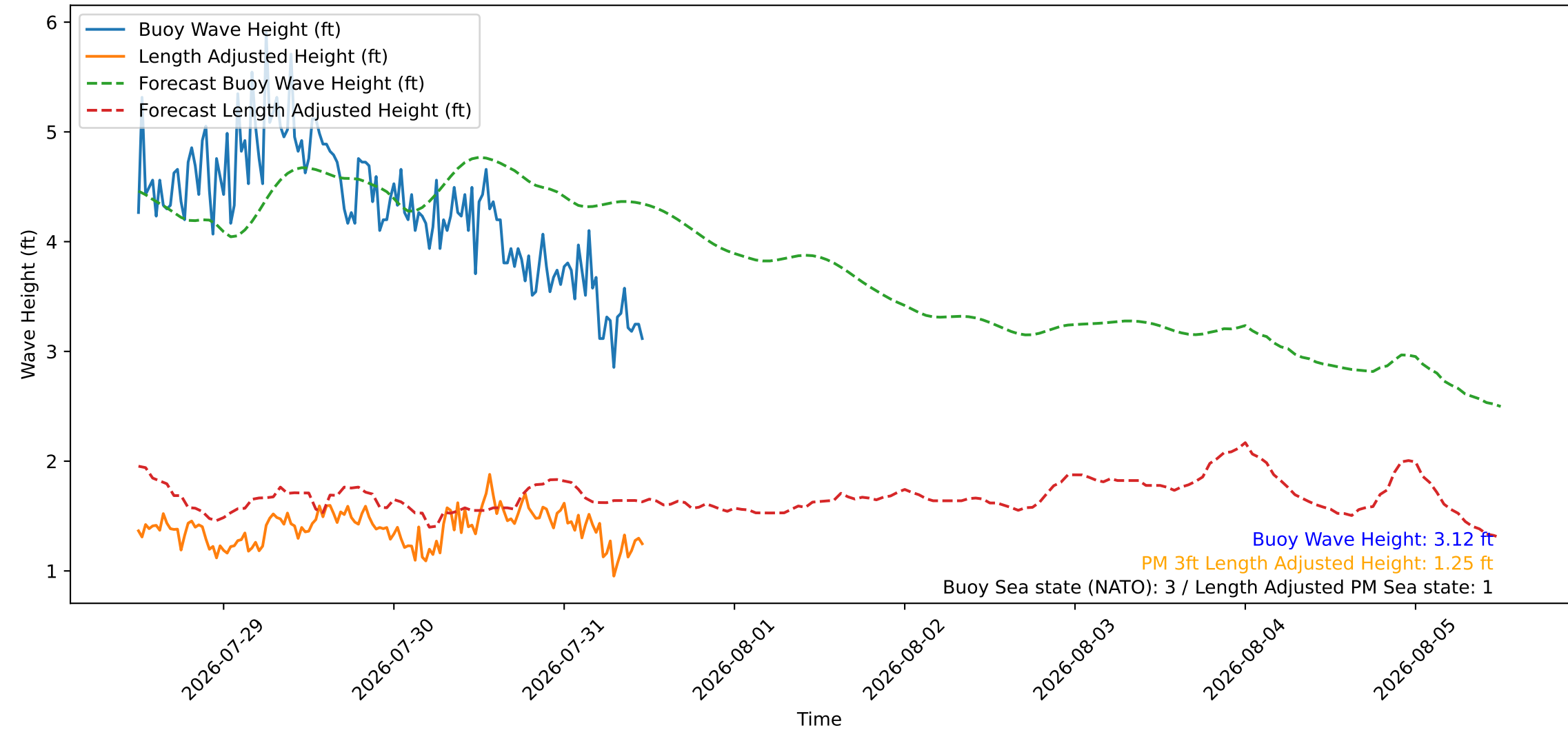
Wave Heights over Time for Oceanside Harbor at 2026-07-31 11:50:26
