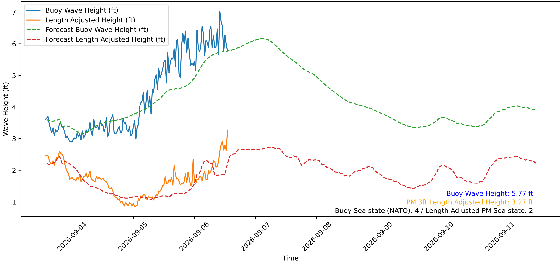
Wave Heights over Time for Oceanside Harbor at 2026-09-06 13:40:30
