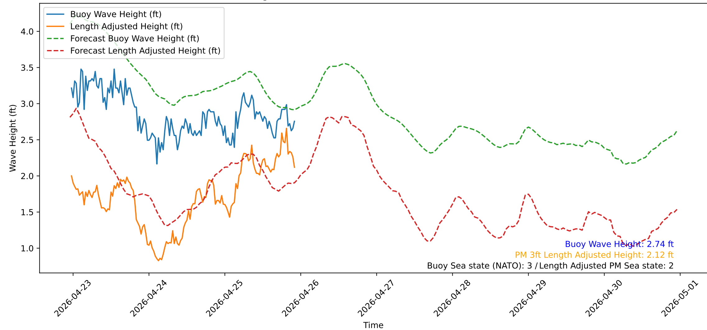
Wave Heights over Time for Red Beach at 2026-04-25 23:00:50
