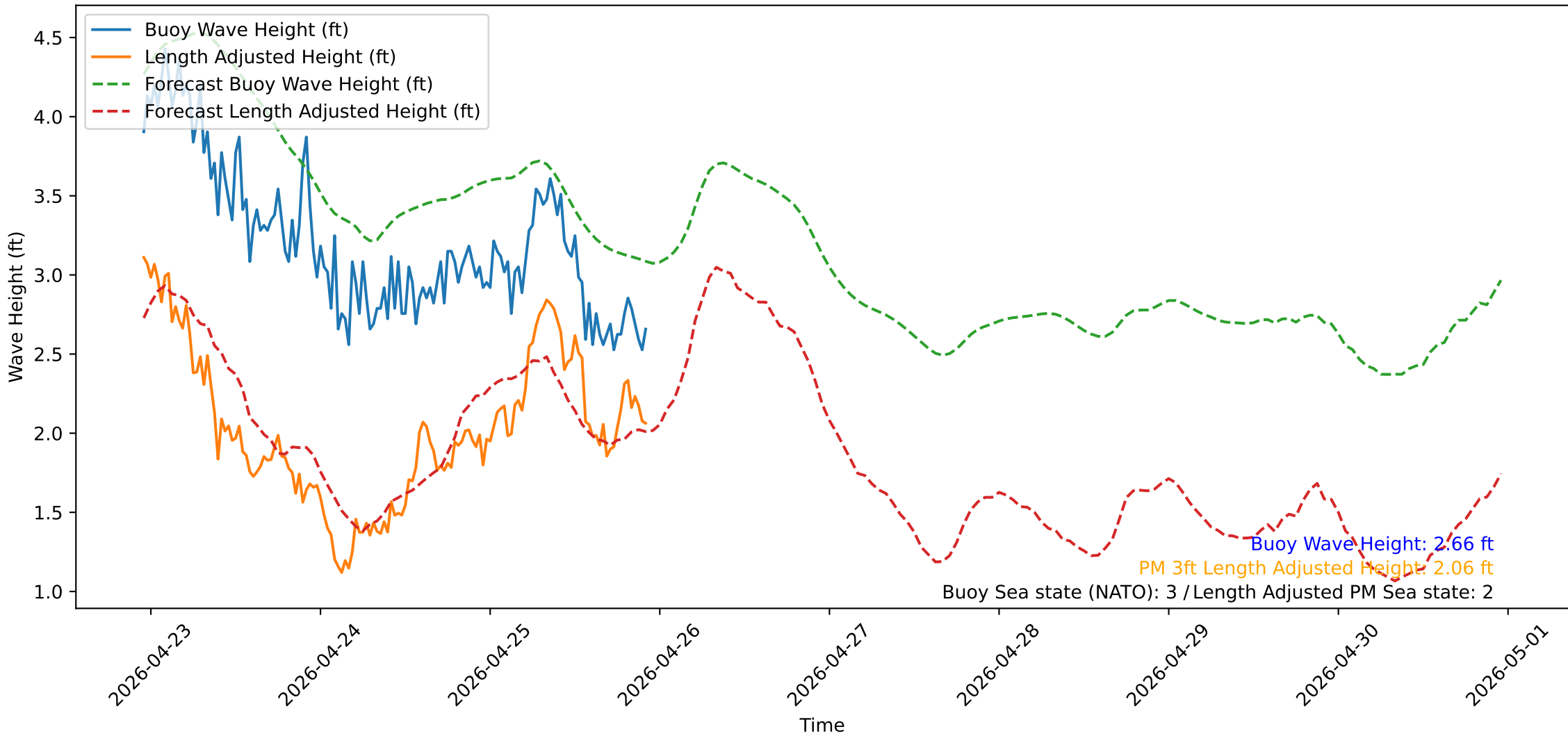
Wave Heights over Time for Oceanside Harbor at 2026-04-25 23:00:31
