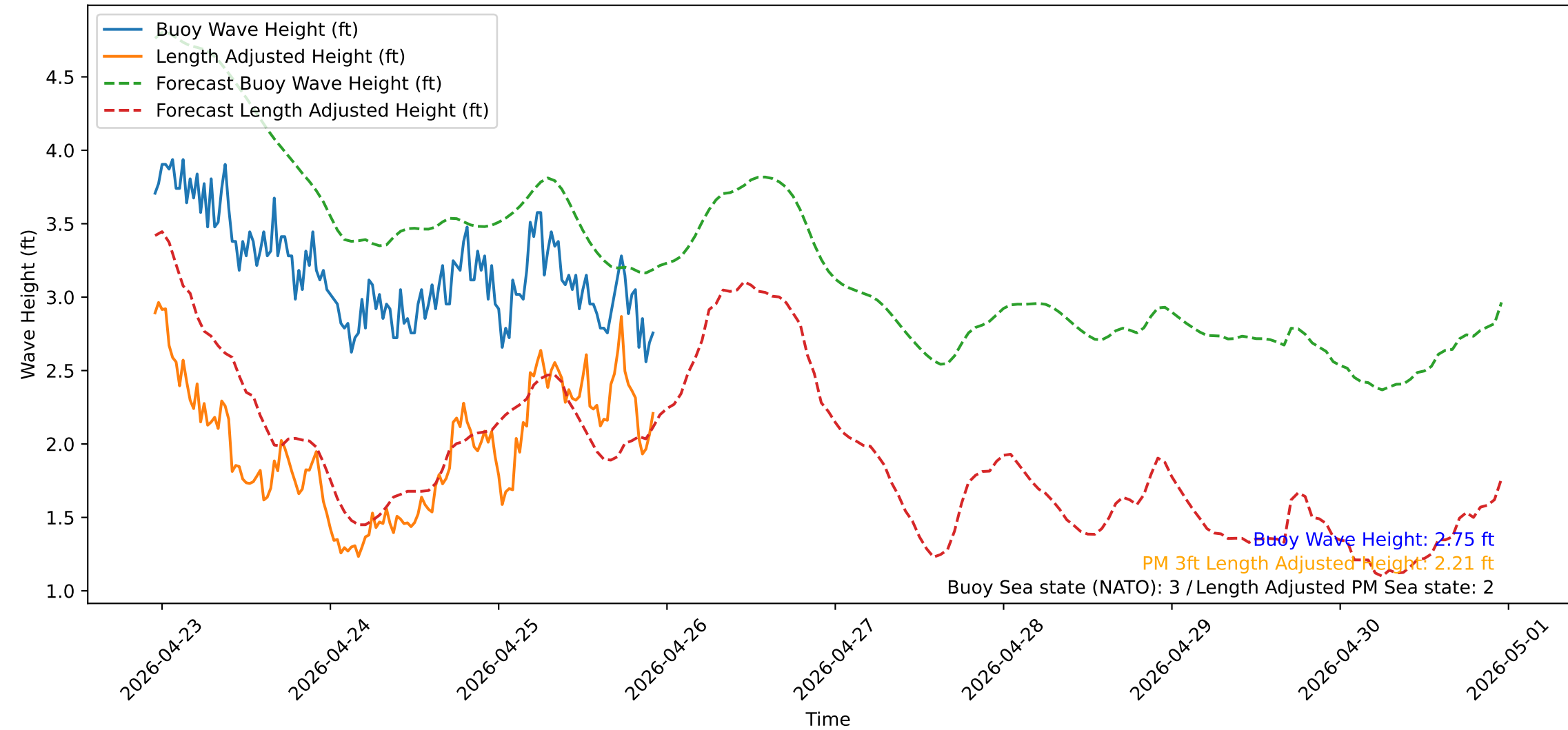
Wave Heights over Time for Green Beach at 2026-04-25 23:01:12
