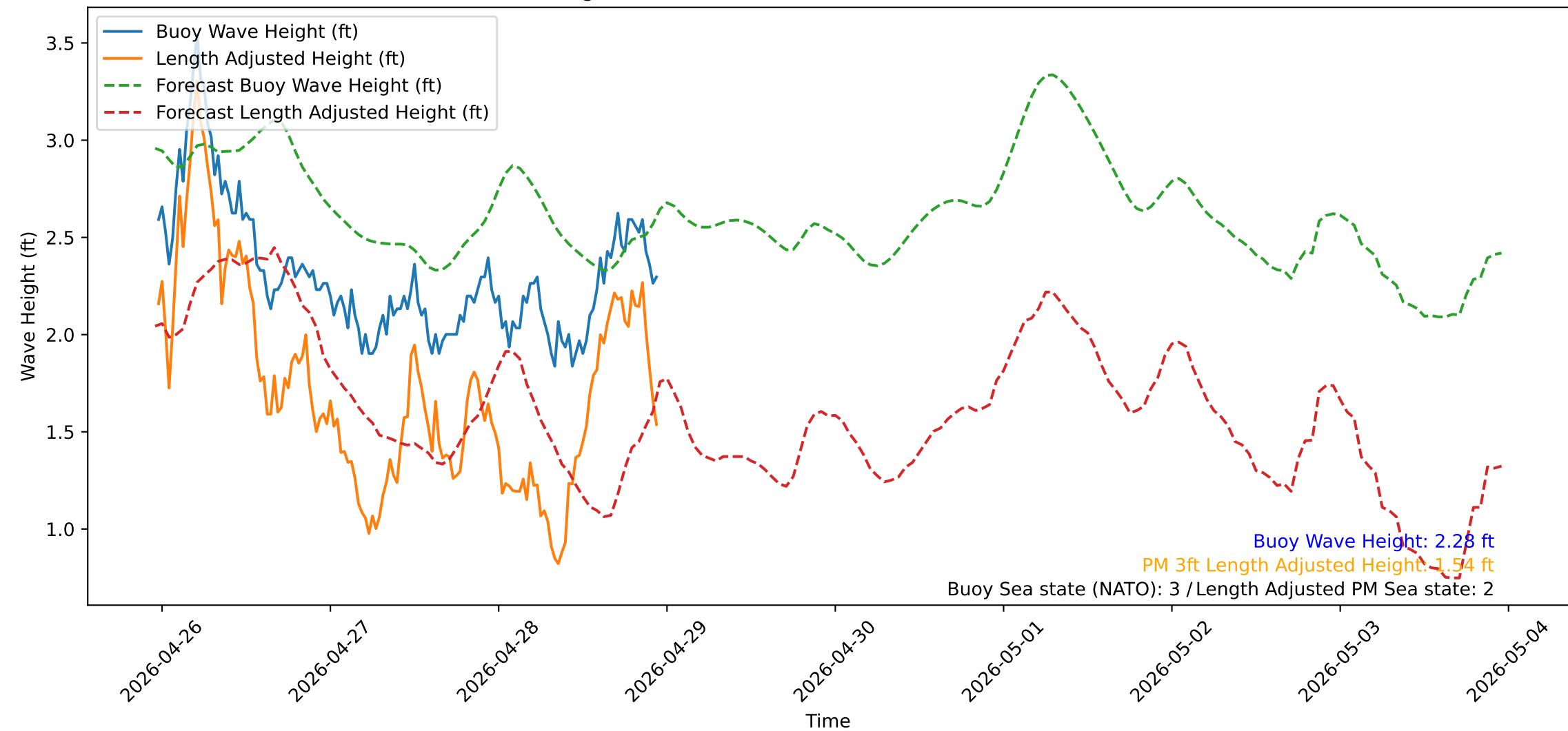
Wave Heights over Time for Red Beach at 2026-04-28 23:10:50
