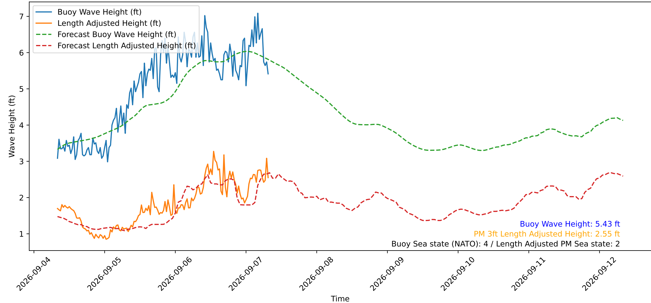
Wave Heights over Time for Oceanside Harbor at 2026-09-07 08:10:29
