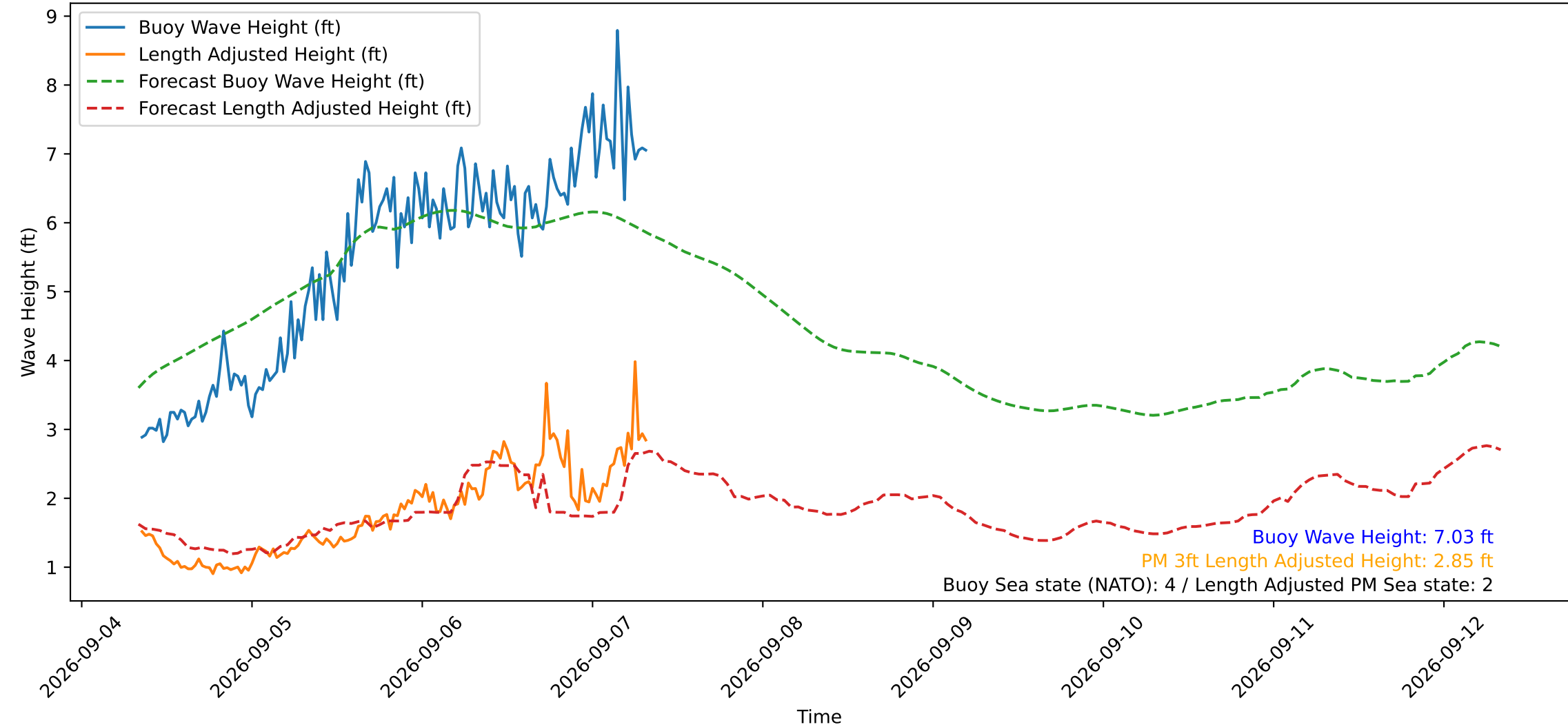
Wave Heights over Time for Green Beach at 2026-09-07 08:11:12
