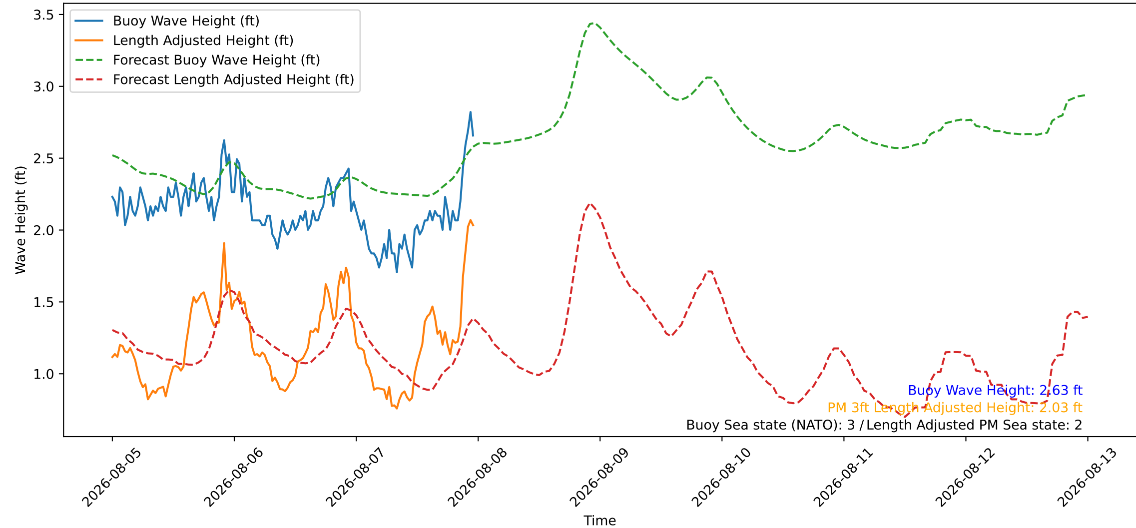
Wave Heights over Time for Green Beach at 2026-08-07 23:51:08
