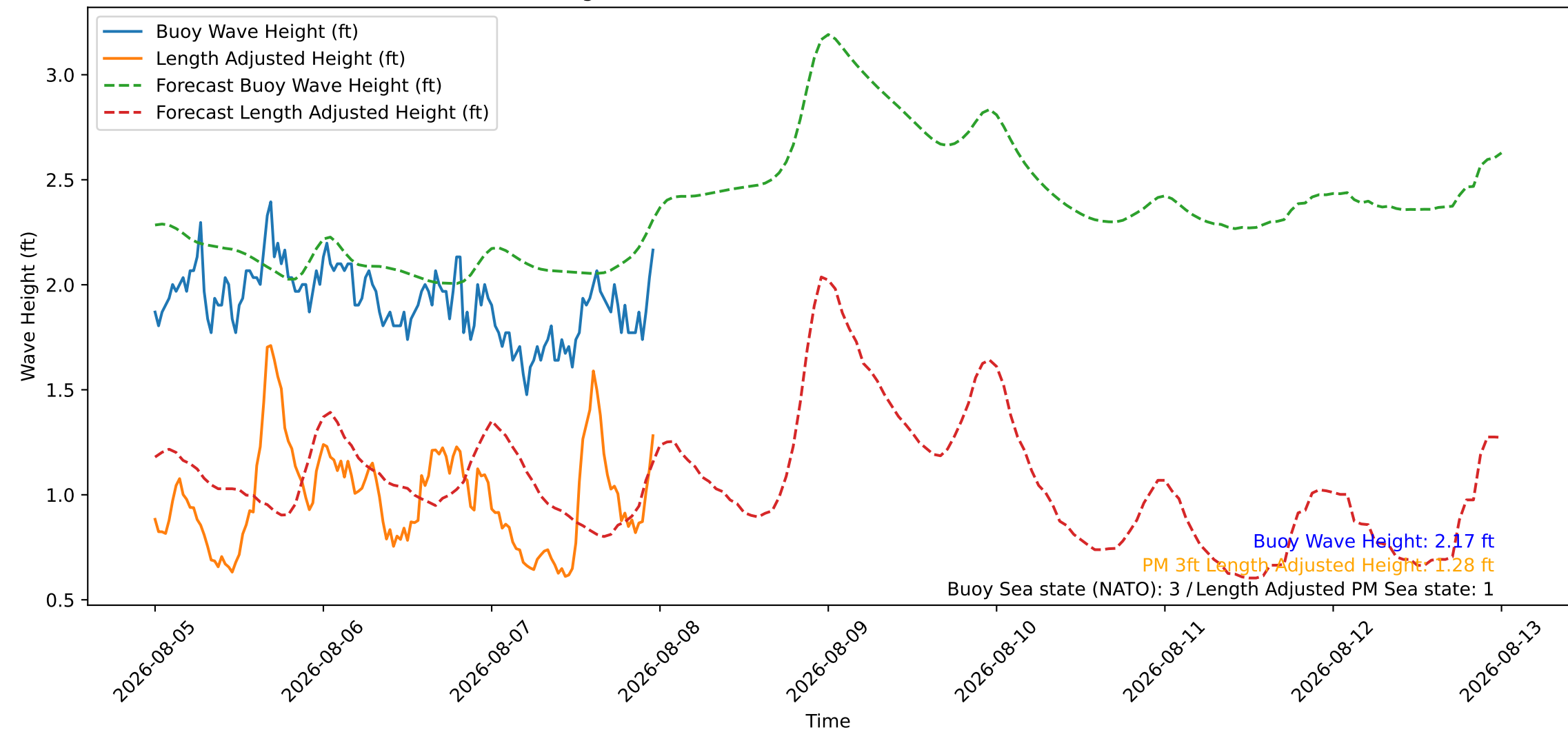
Wave Heights over Time for Red Beach at 2026-08-07 23:50:46
