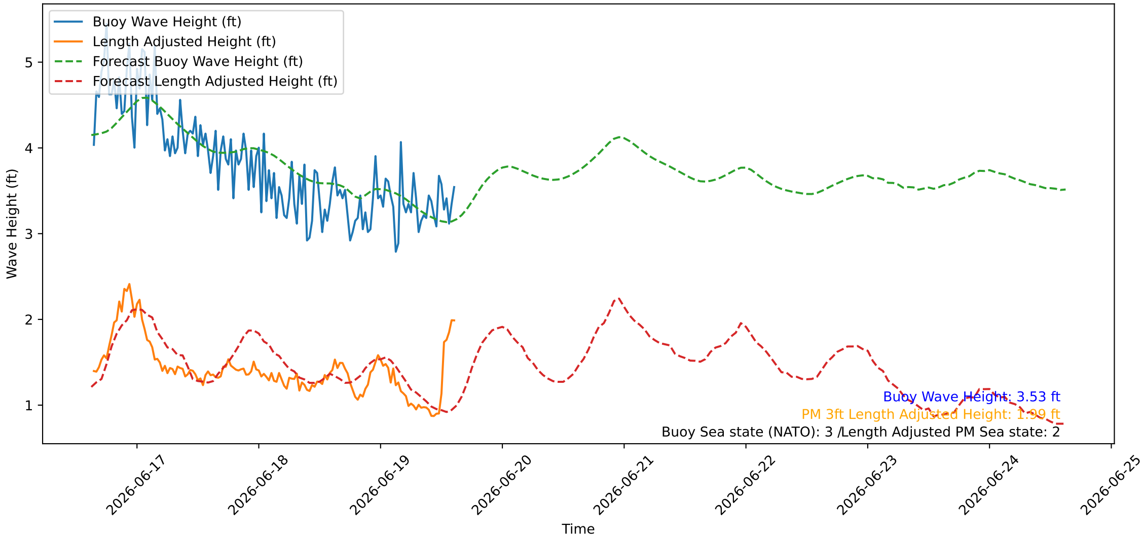
Wave Heights over Time for Oceanside Harbor at 2026-06-19 15:20:26
