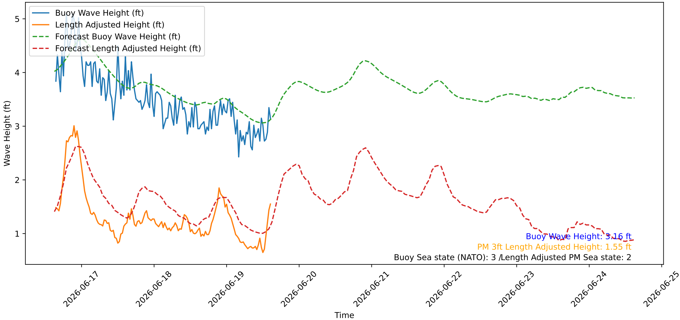
Wave Heights over Time for Green Beach at 2026-06-19 15:21:09
