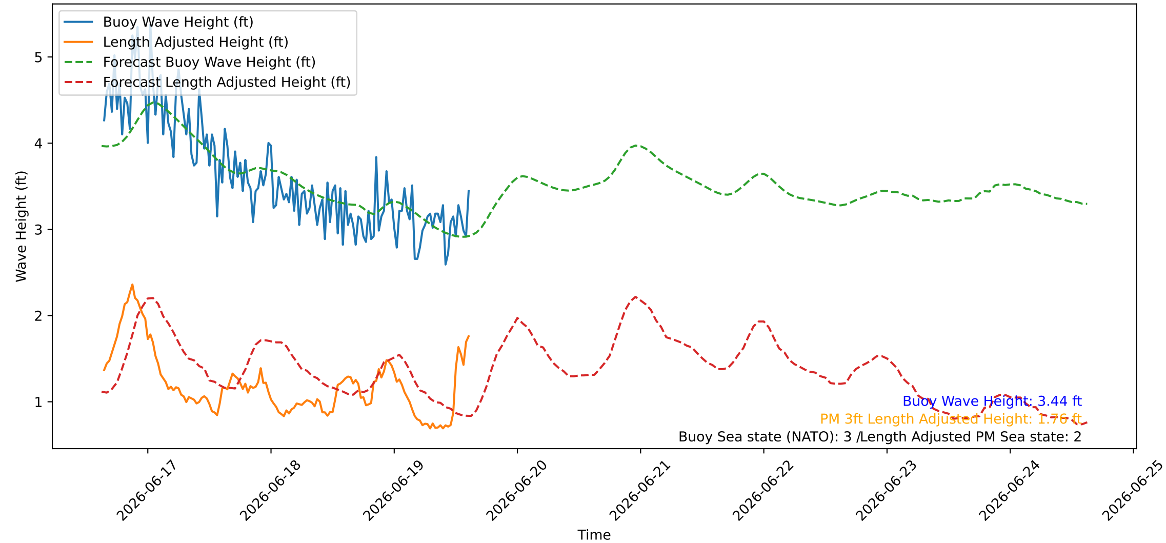
Wave Heights over Time for Red Beach at 2026-06-19 15:20:46
