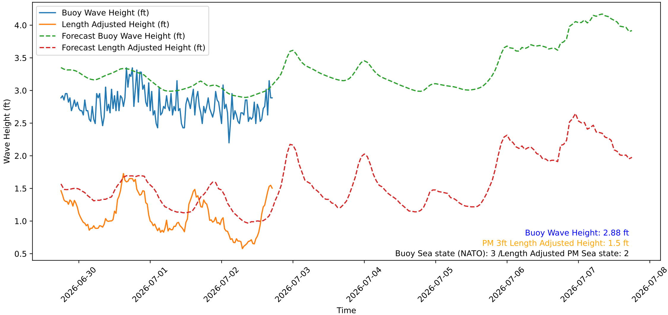
Wave Heights over Time for Red Beach at 2026-07-02 17:50:47
