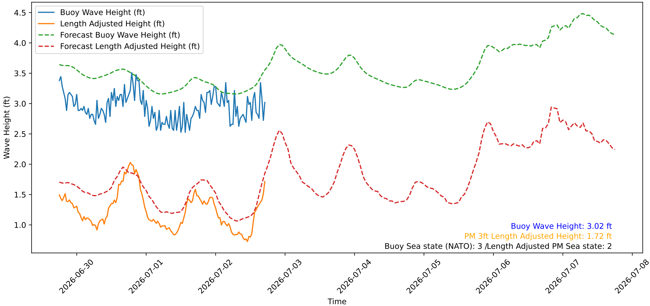
Wave Heights over Time for Green Beach at 2026-07-02 17:51:09
