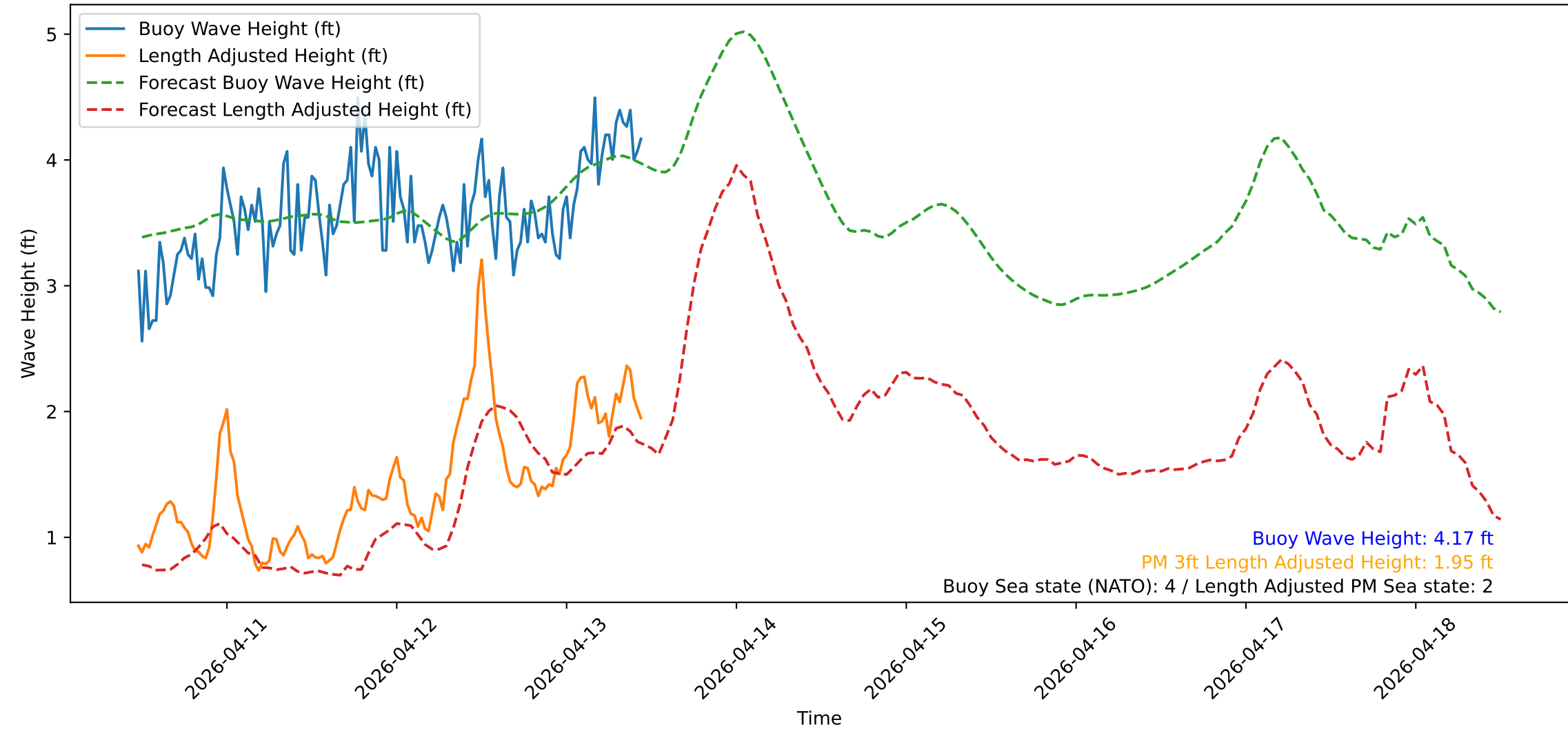
Wave Heights over Time for Green Beach at 2026-04-13 11:31:13
