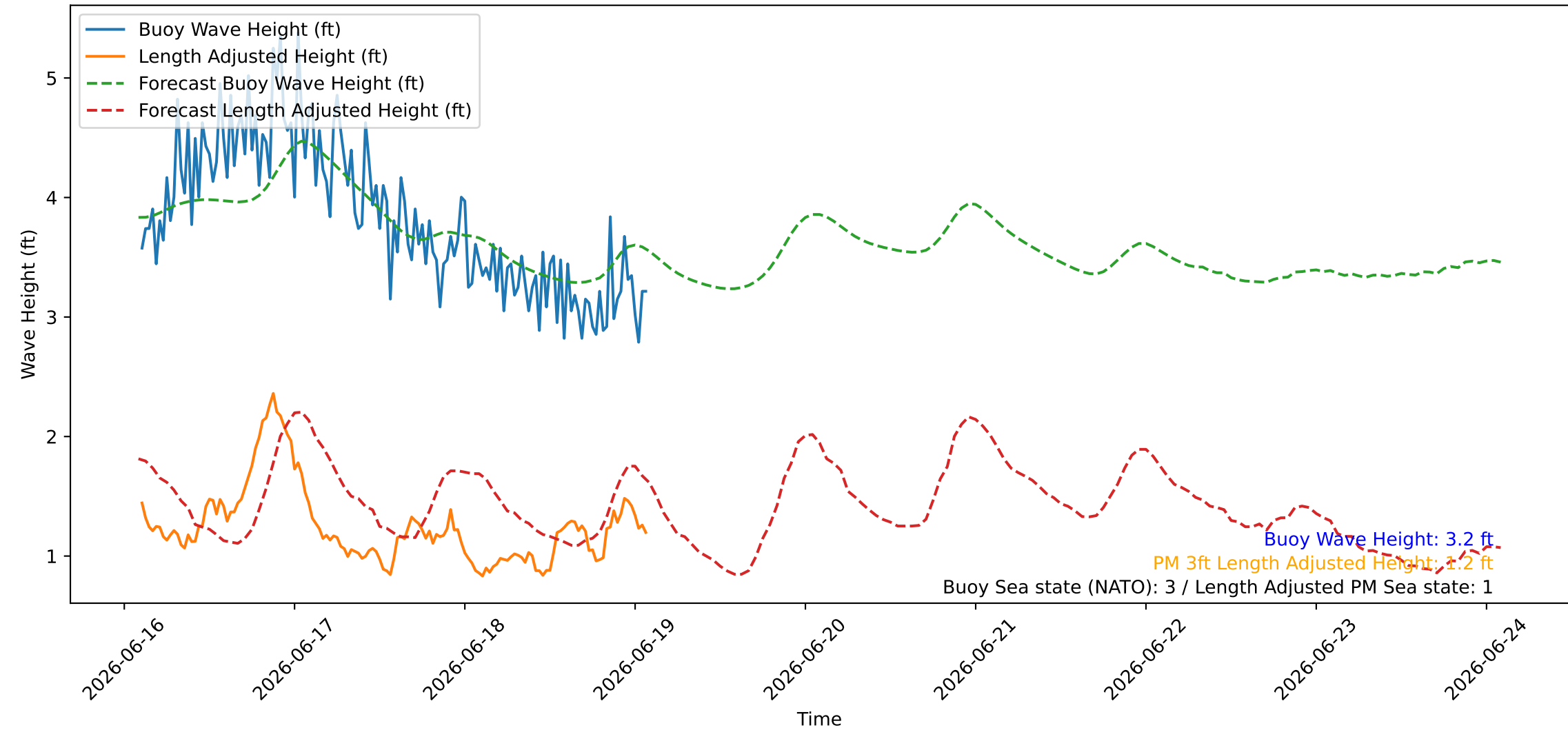
Wave Heights over Time for Red Beach at 2026-06-19 02:20:45
