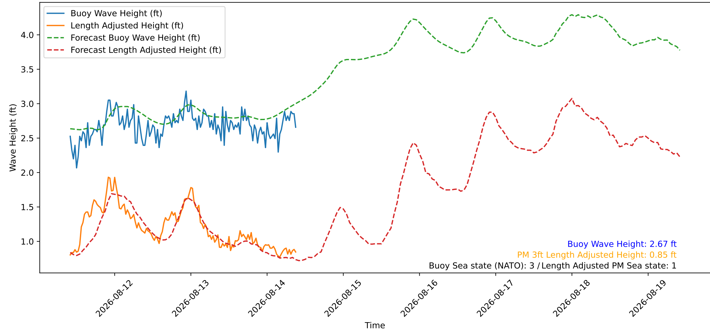
Wave Heights over Time for Oceanside Harbor at 2026-08-14 09:50:27
