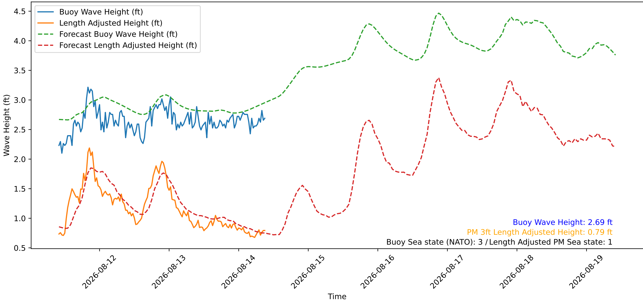
Wave Heights over Time for Green Beach at 2026-08-14 09:51:09
