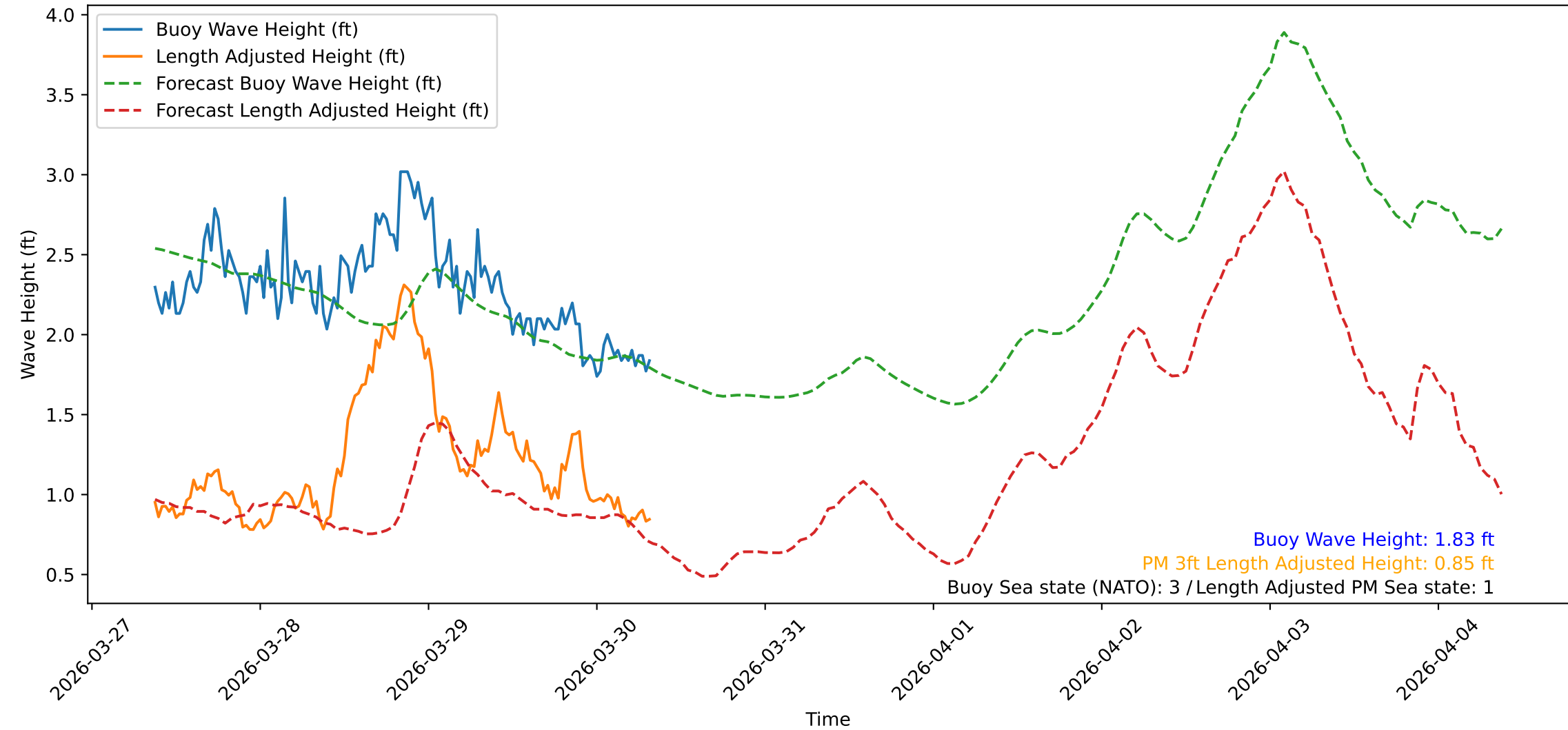
Wave Heights over Time for Red Beach at 2026-03-30 08:30:47
