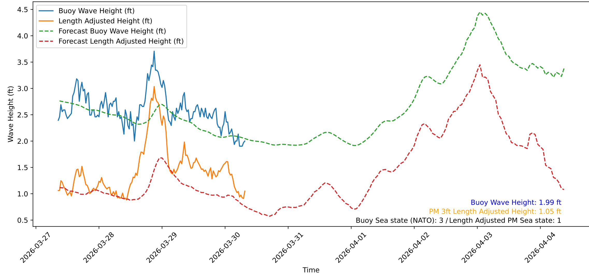
Wave Heights over Time for Green Beach at 2026-03-30 08:31:09
