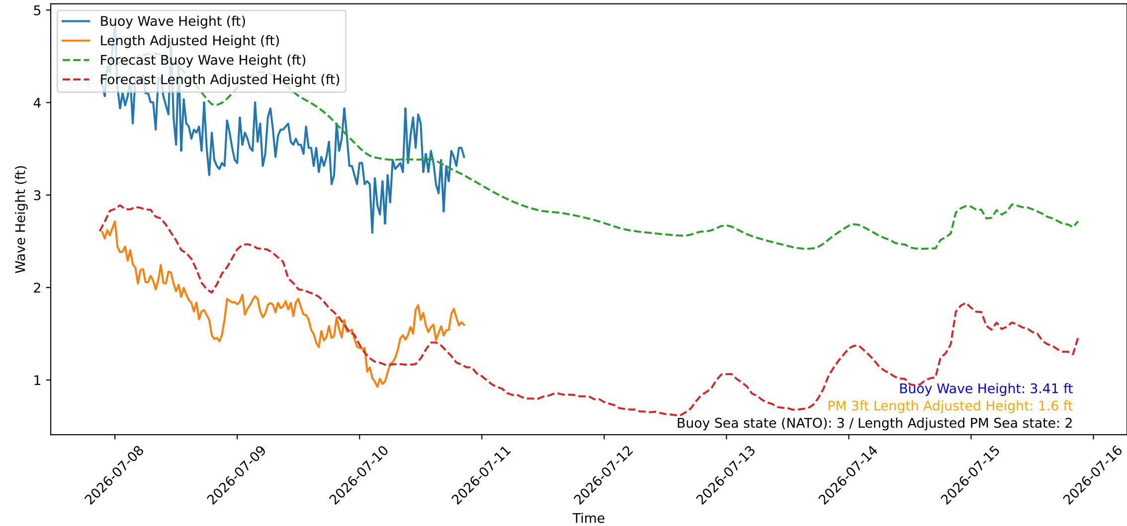
Wave Heights over Time for Red Beach at 2026-07-10 21:20:48
