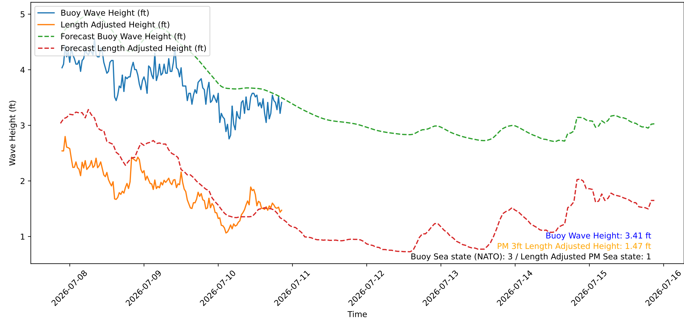
Wave Heights over Time for Green Beach at 2026-07-10 21:21:10
