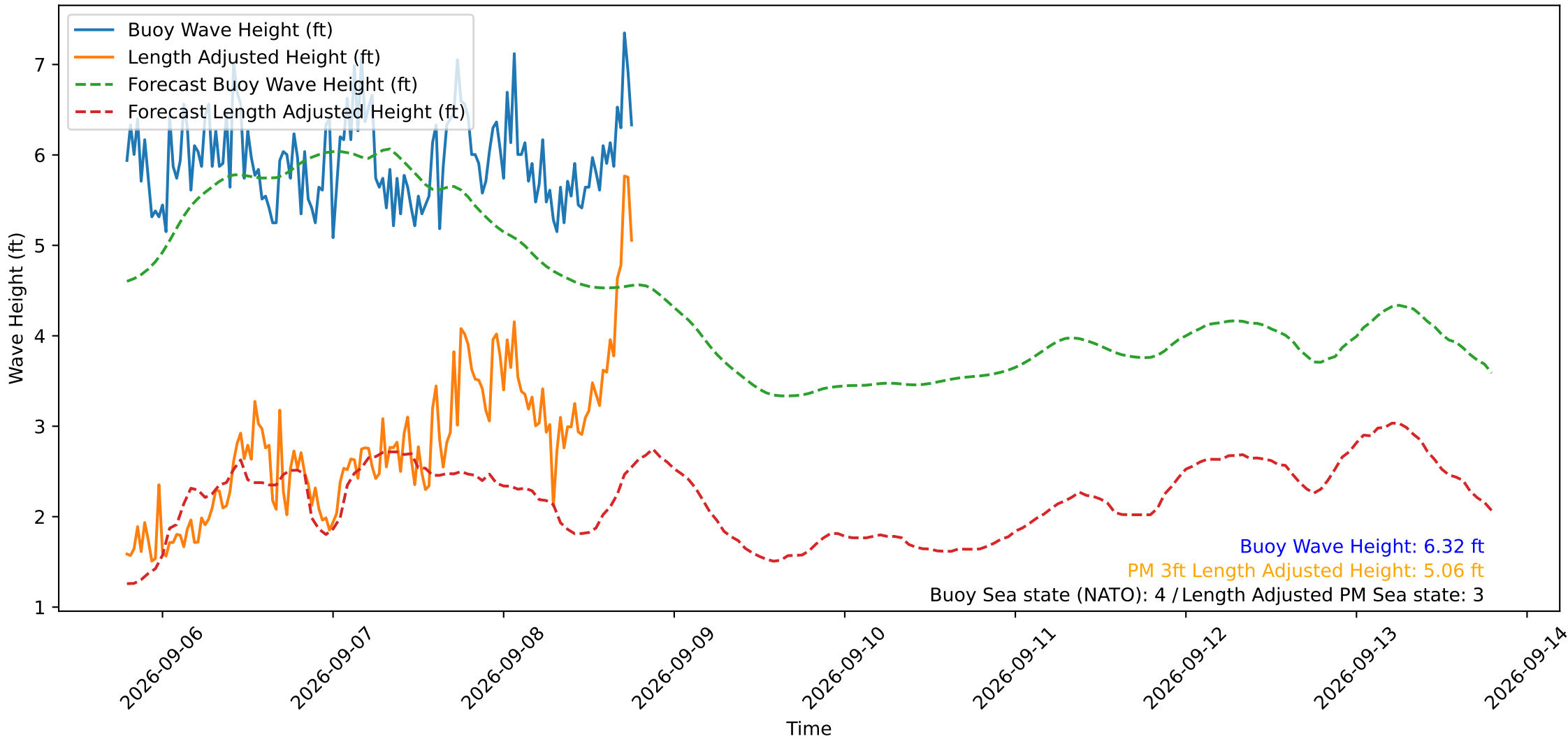
Wave Heights over Time for Oceanside Harbor at 2026-09-08 18:50:30
