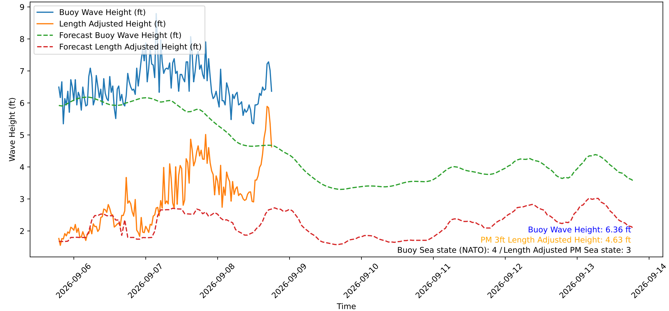
Wave Heights over Time for Green Beach at 2026-09-08 18:51:14
