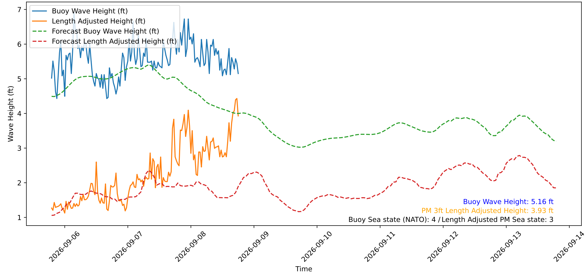
Wave Heights over Time for Red Beach at 2026-09-08 18:50:50
