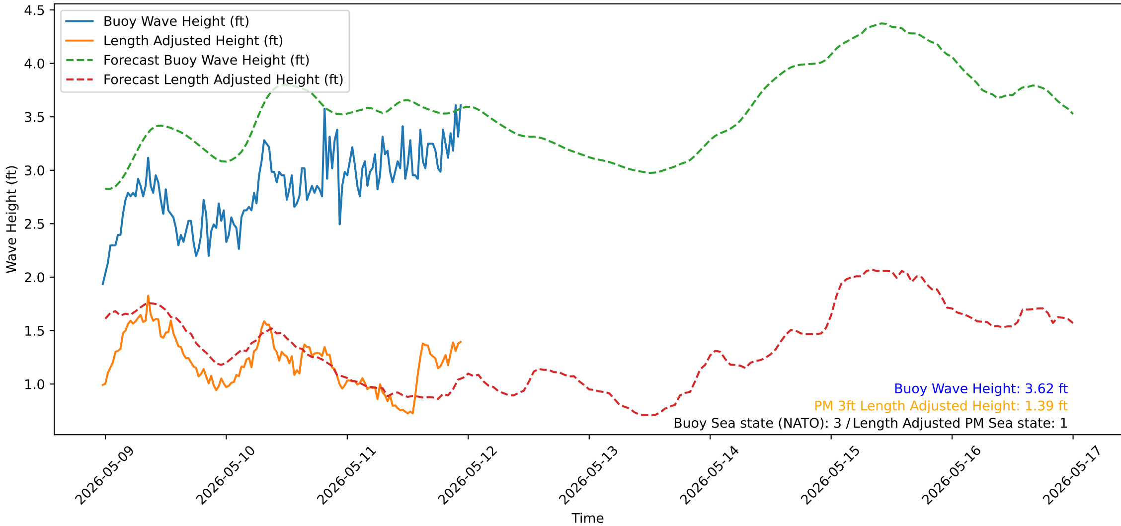
Wave Heights over Time for Oceanside Harbor at 2026-05-11 23:30:31
