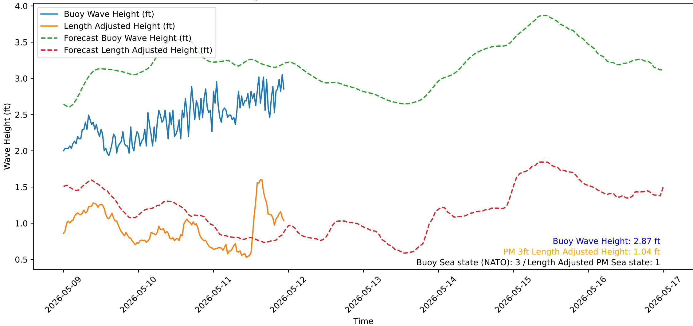
Wave Heights over Time for Red Beach at 2026-05-11 23:30:50
