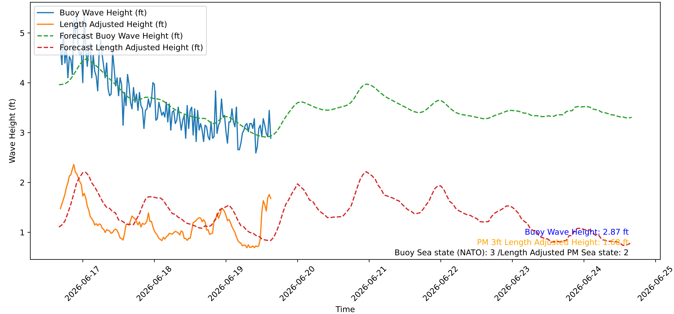
Wave Heights over Time for Red Beach at 2026-06-19 16:00:54
