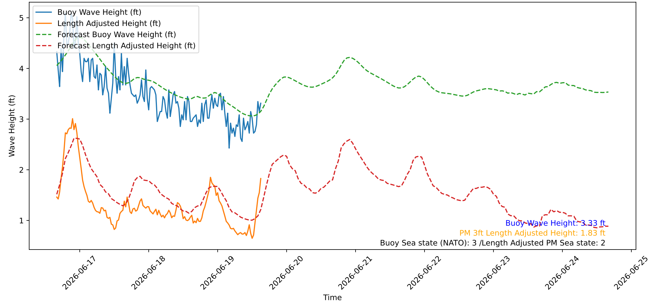
Wave Heights over Time for Green Beach at 2026-06-19 16:01:16
