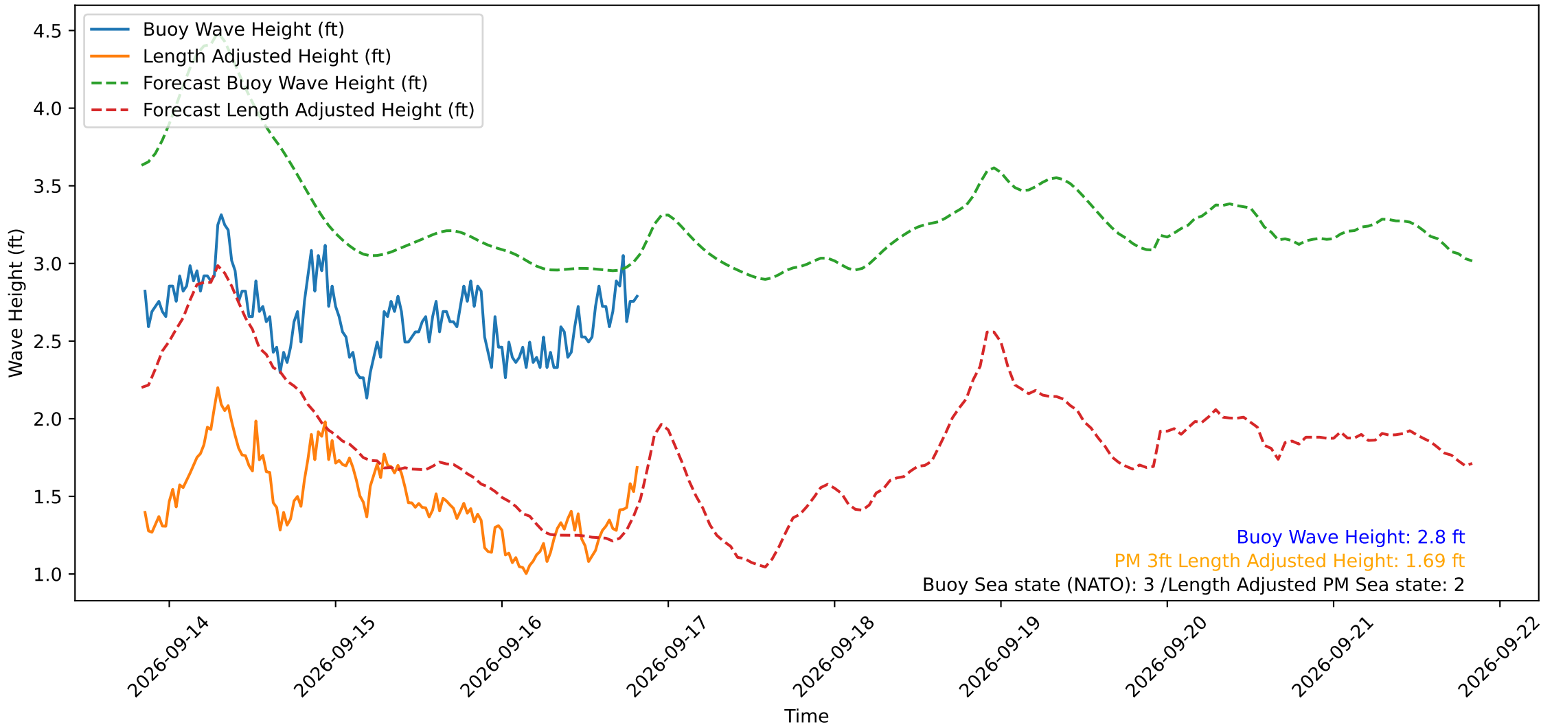
Wave Heights over Time for Green Beach at 2026-09-16 20:21:14
