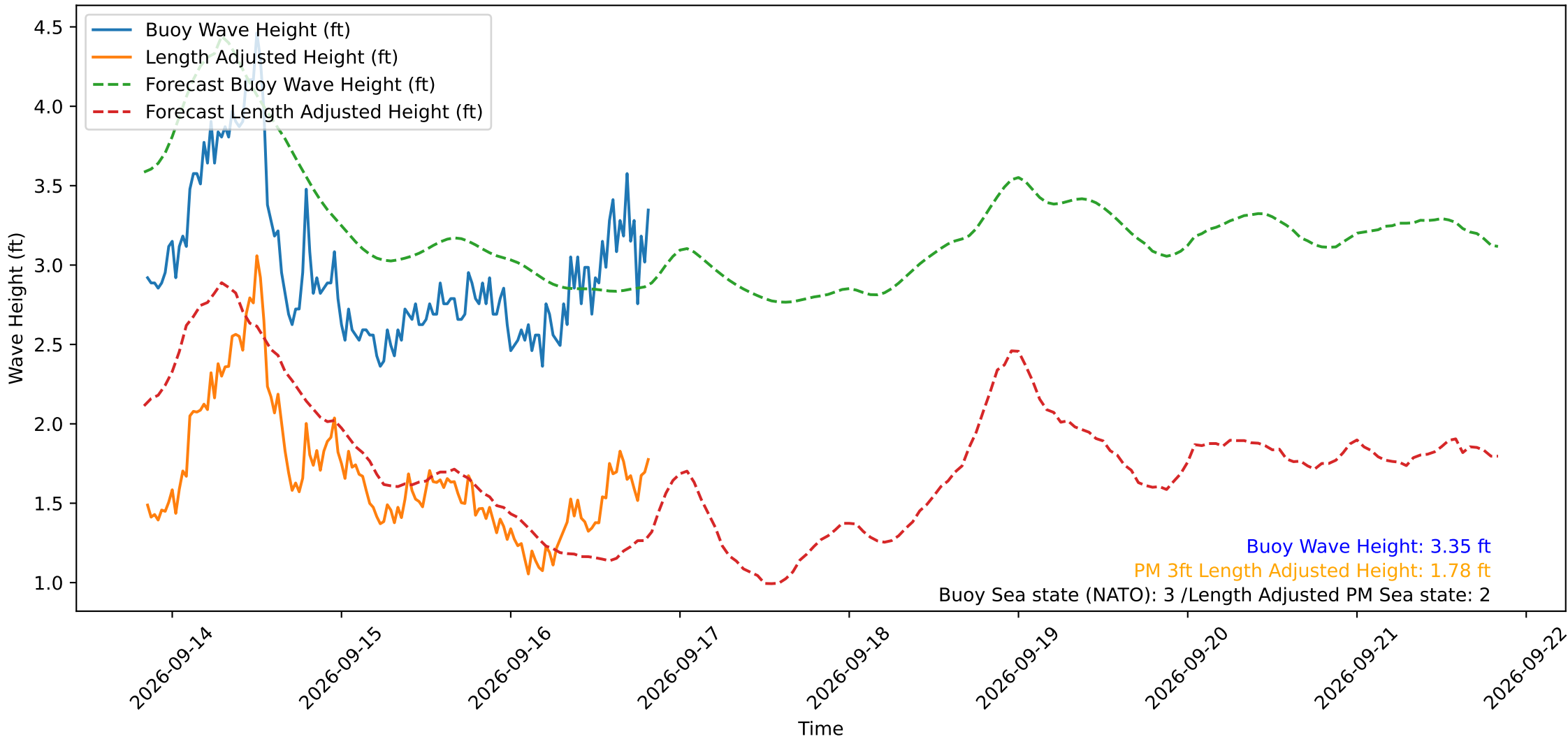
Wave Heights over Time for Oceanside Harbor at 2026-09-16 20:20:29
