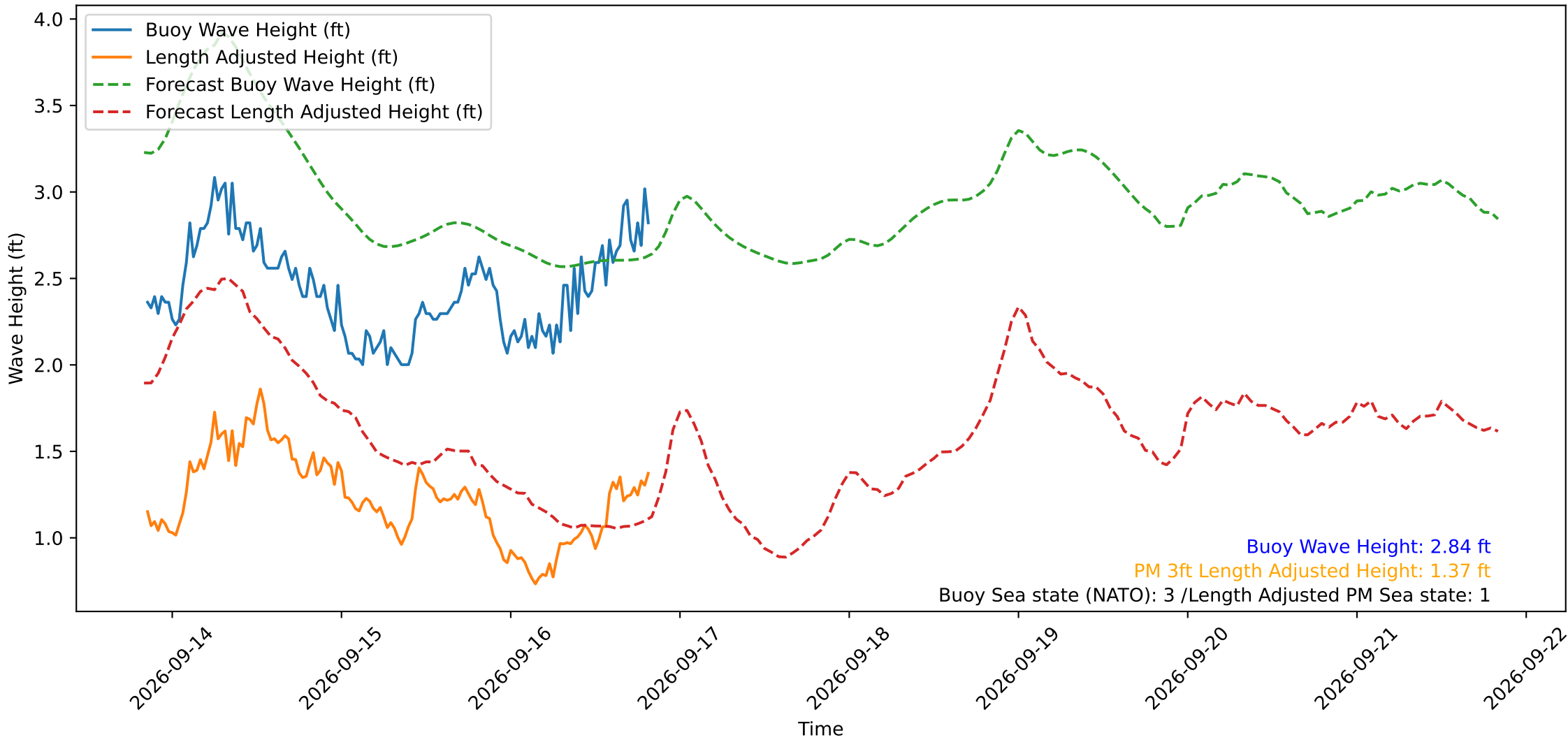
Wave Heights over Time for Red Beach at 2026-09-16 20:20:50
