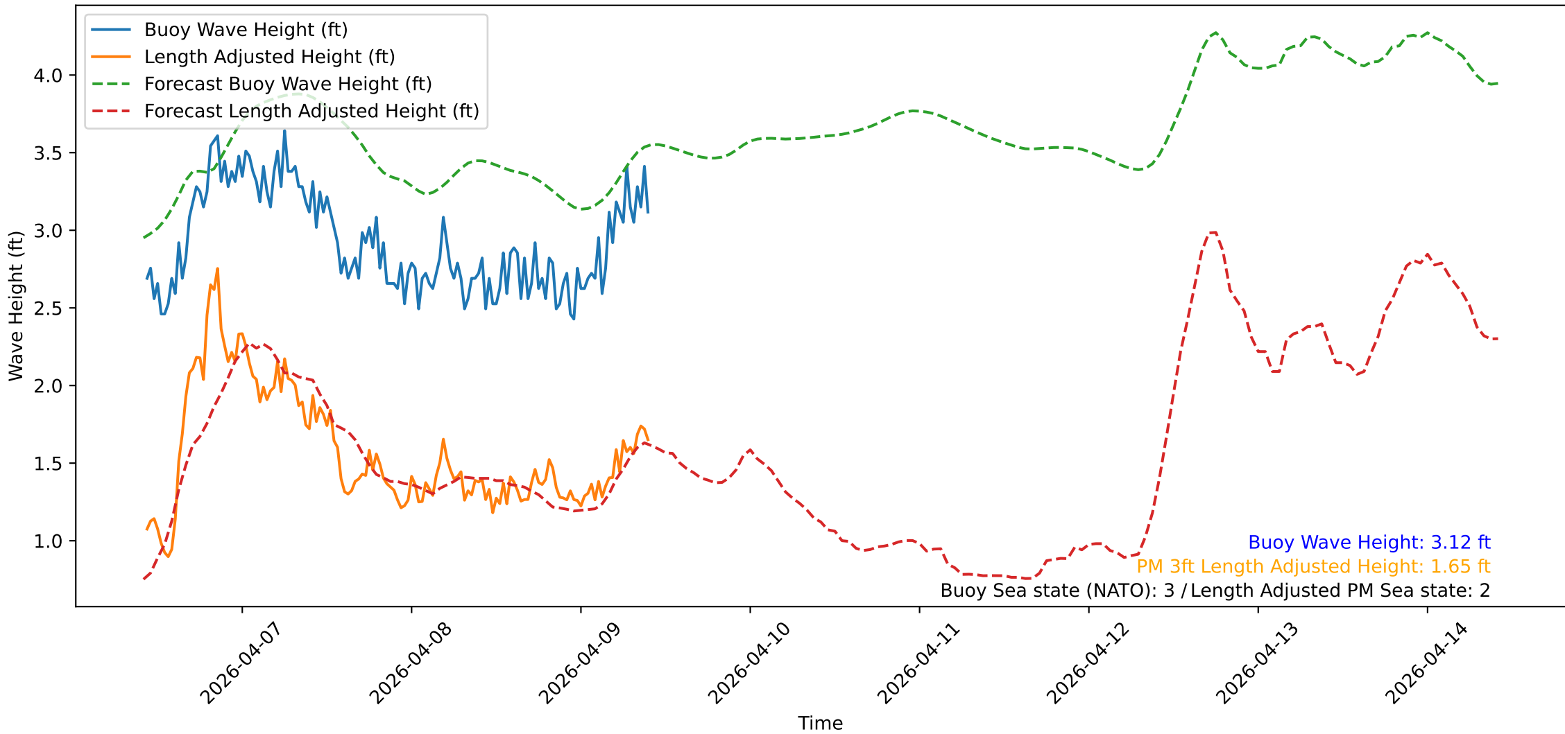
Wave Heights over Time for Oceanside Harbor at 2026-04-09 10:20:31
