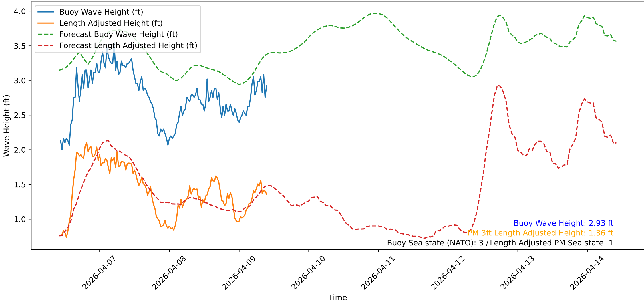
Wave Heights over Time for Red Beach at 2026-04-09 10:20:48
