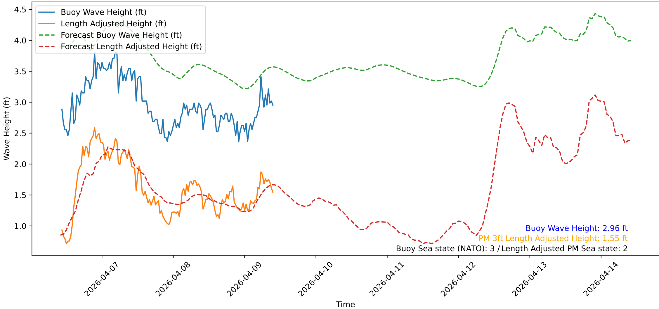
Wave Heights over Time for Green Beach at 2026-04-09 10:21:09
