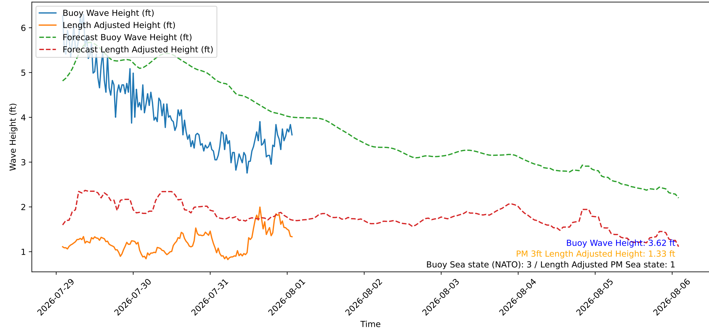
Wave Heights over Time for Green Beach at 2026-08-01 02:11:09
