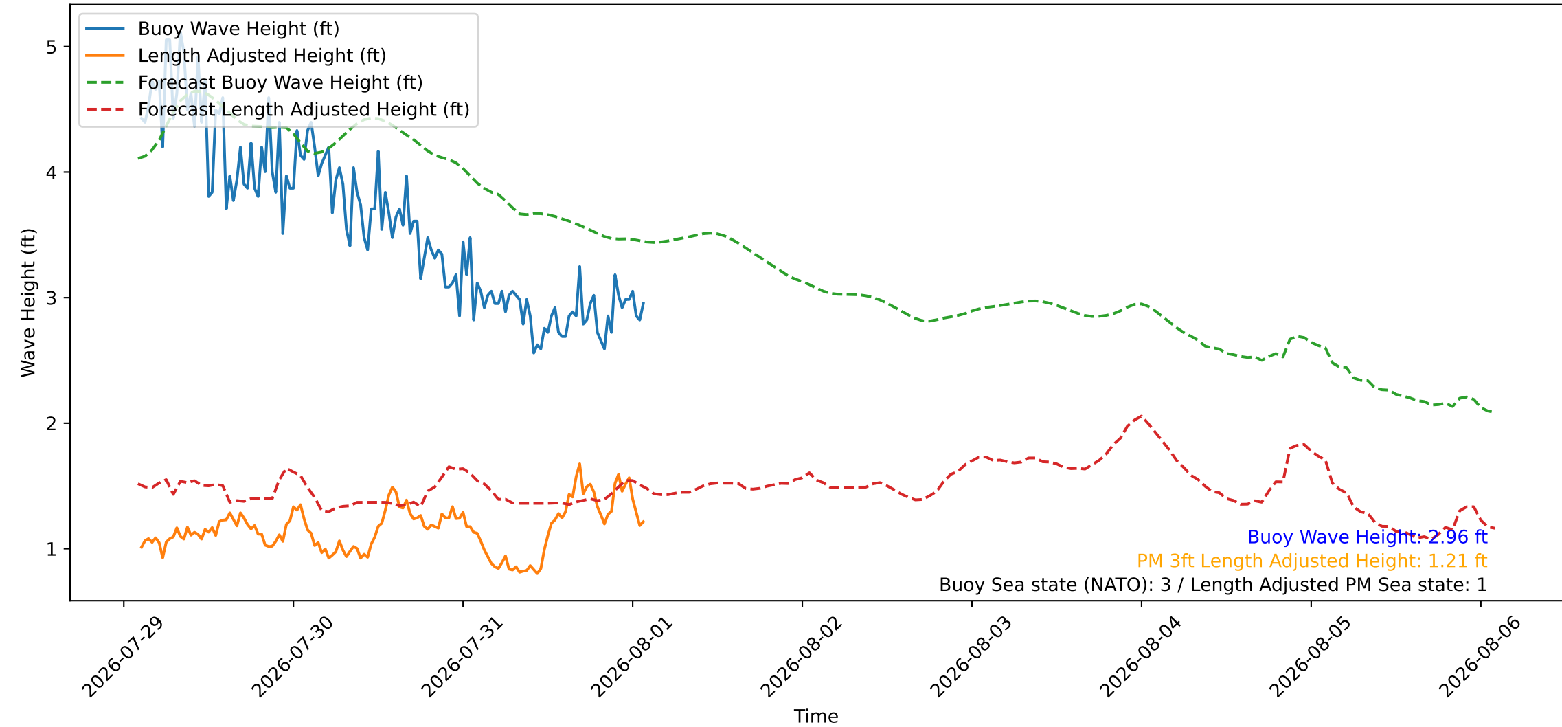
Wave Heights over Time for Red Beach at 2026-08-01 02:10:46
