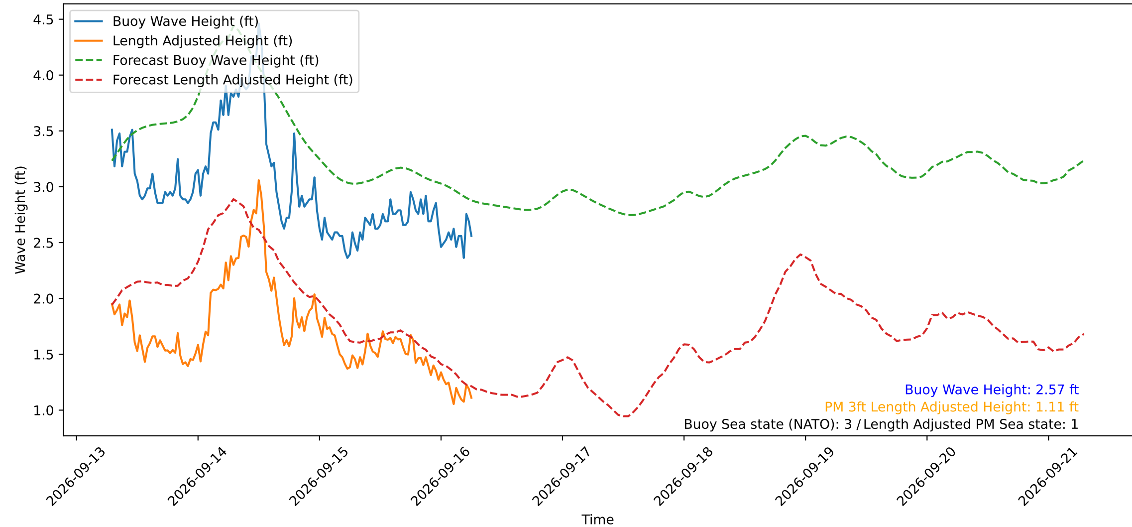
Wave Heights over Time for Oceanside Harbor at 2026-09-16 07:00:30
