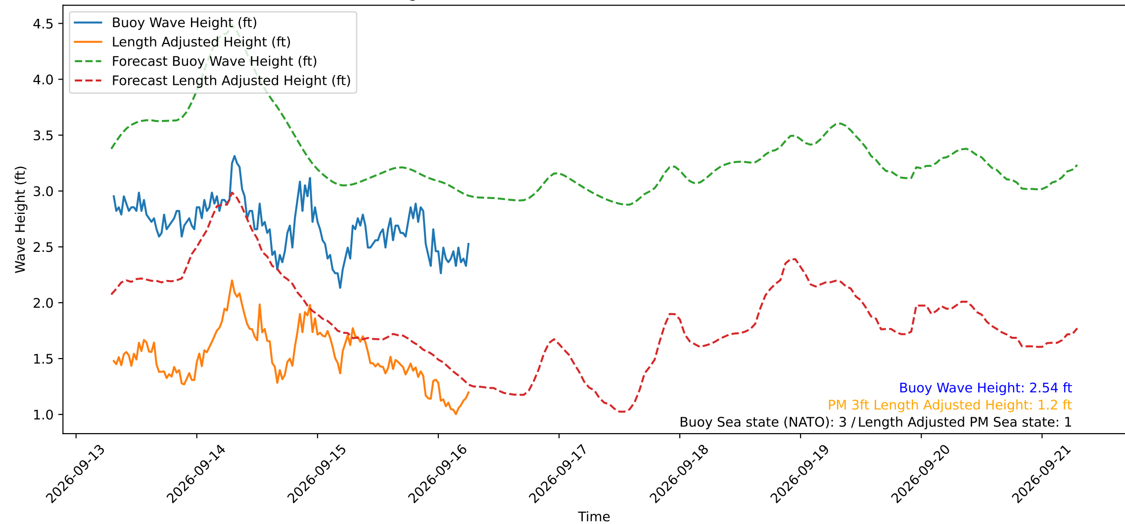
Wave Heights over Time for Green Beach at 2026-09-16 07:01:12
