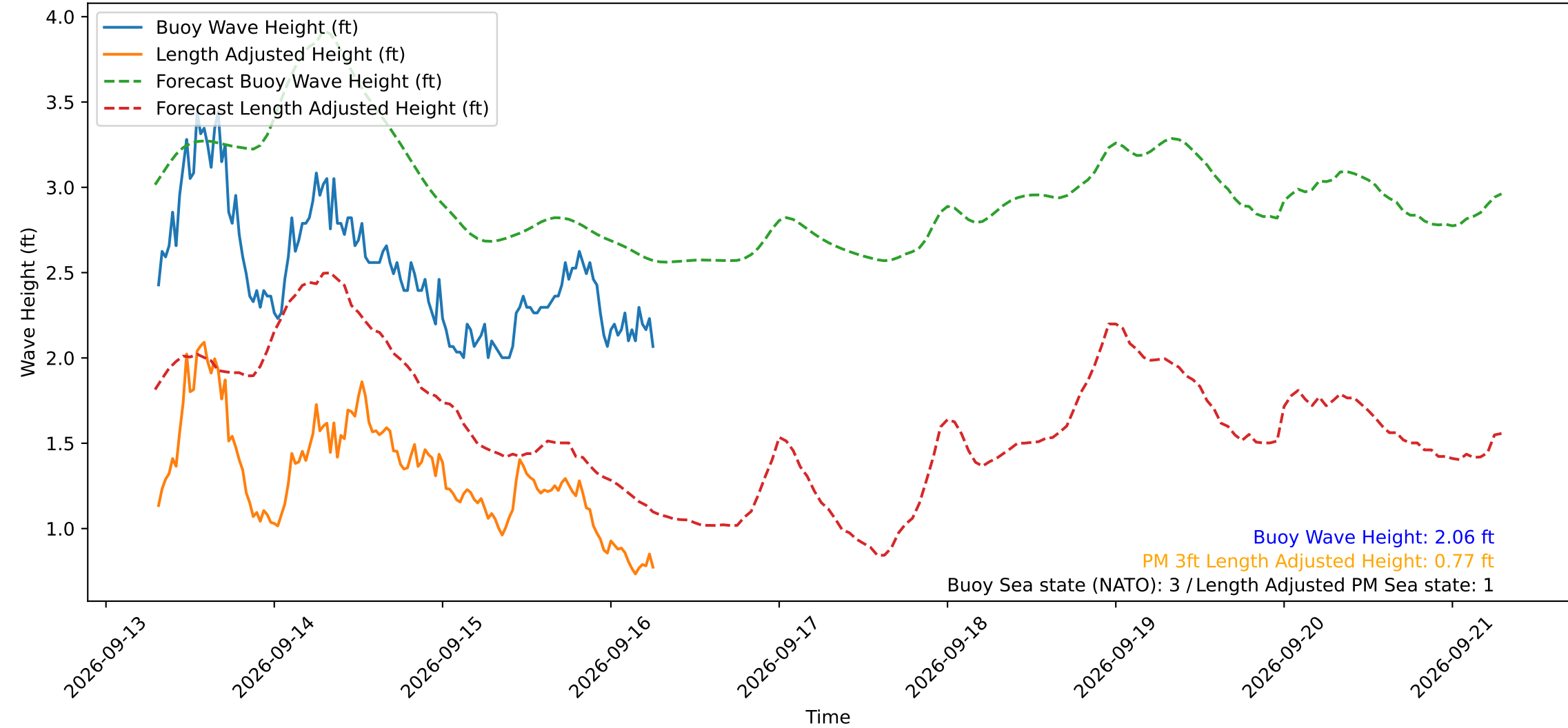
Wave Heights over Time for Red Beach at 2026-09-16 07:00:49
