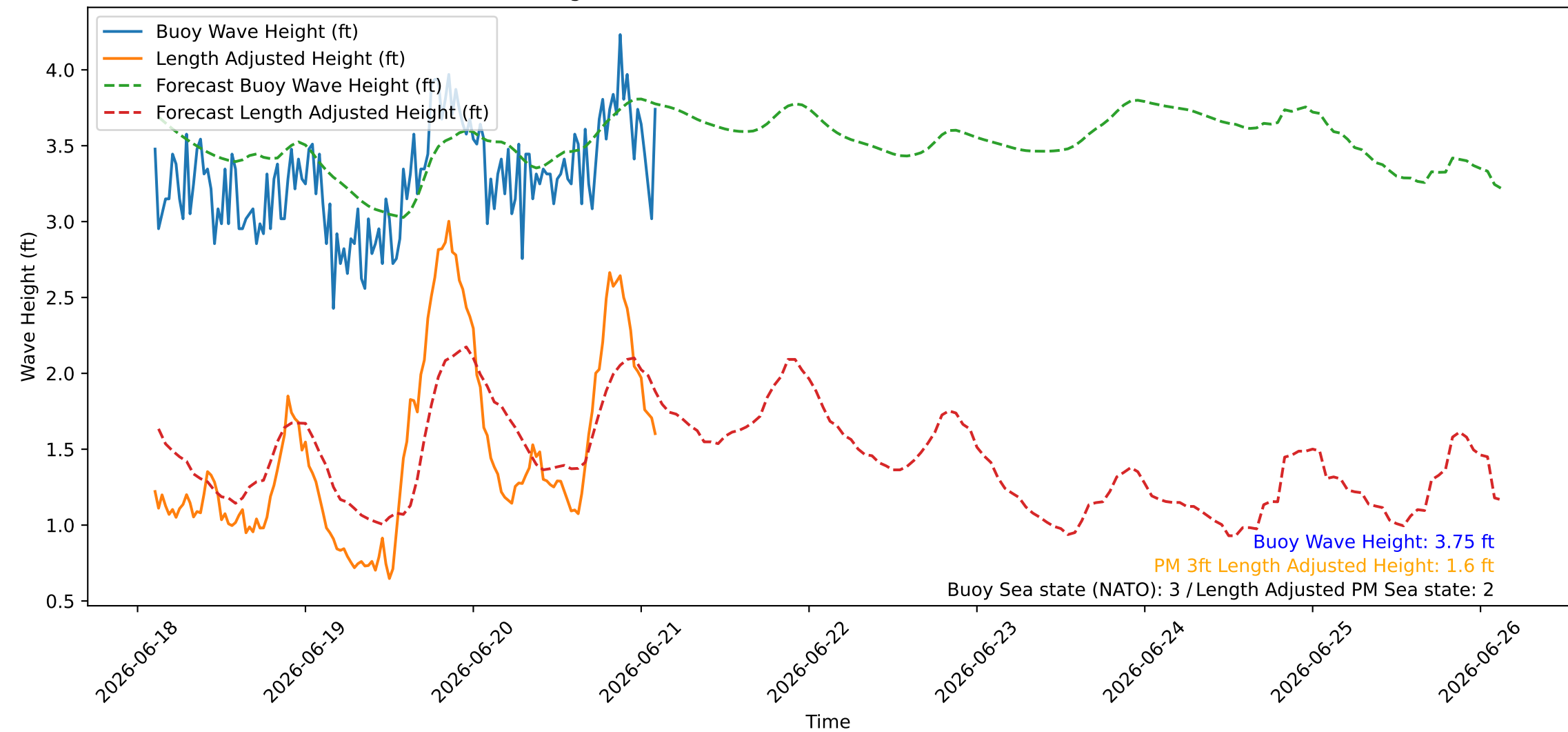
Wave Heights over Time for Green Beach at 2026-06-21 02:41:07
