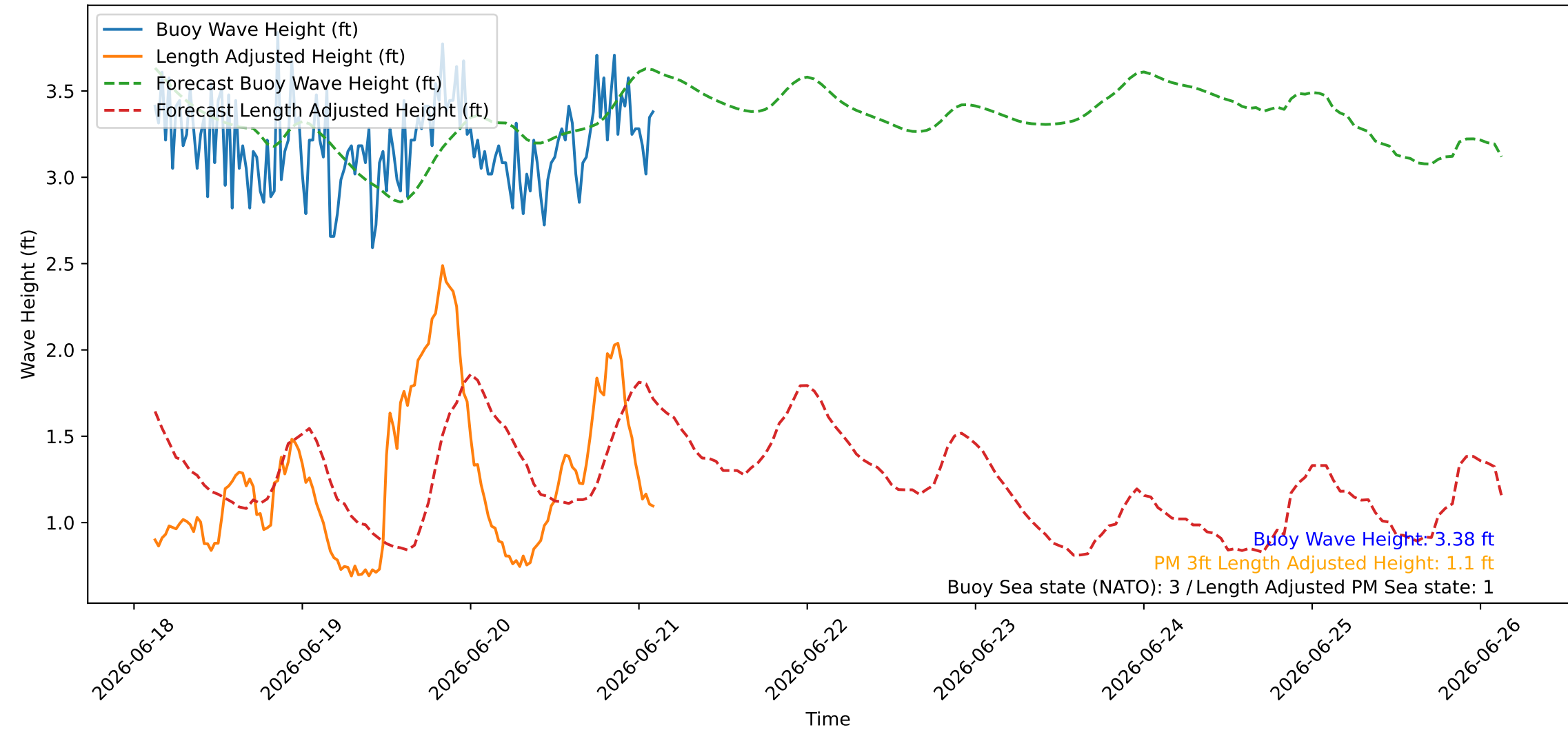
Wave Heights over Time for Red Beach at 2026-06-21 02:40:45
