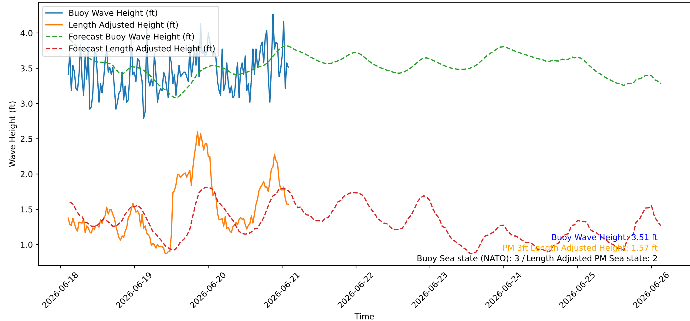
Wave Heights over Time for Oceanside Harbor at 2026-06-21 02:40:26
